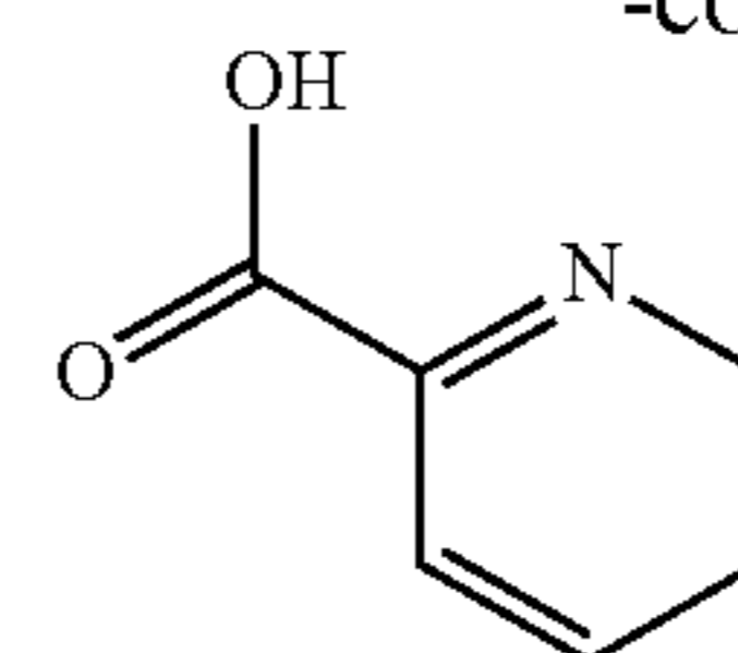
5,6-dihydropyridine-2-carboxylic acid
