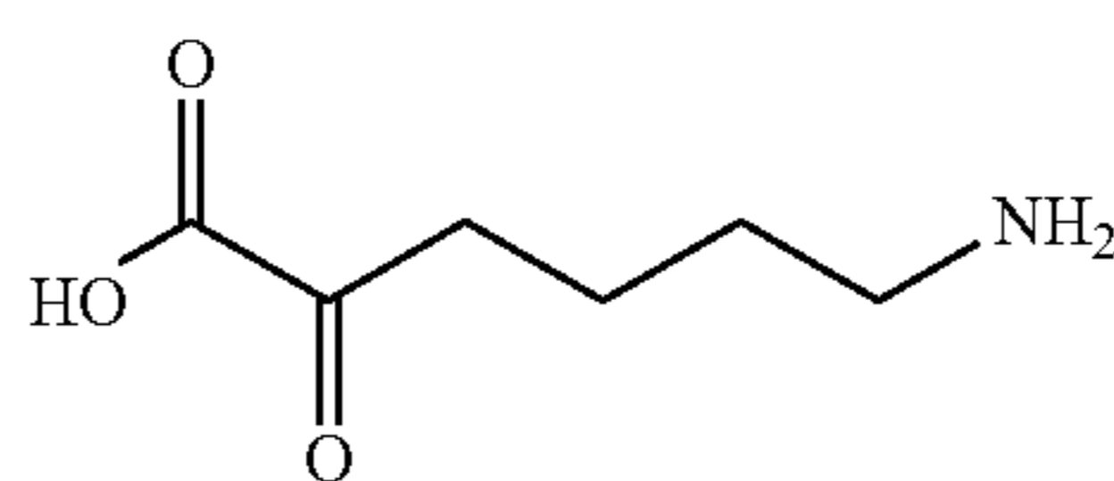
6-amino-2-oxohexanoic acid
