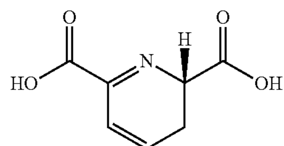
(S)-2,3-dihydropyridine-2,6-dicarboxylic acid
