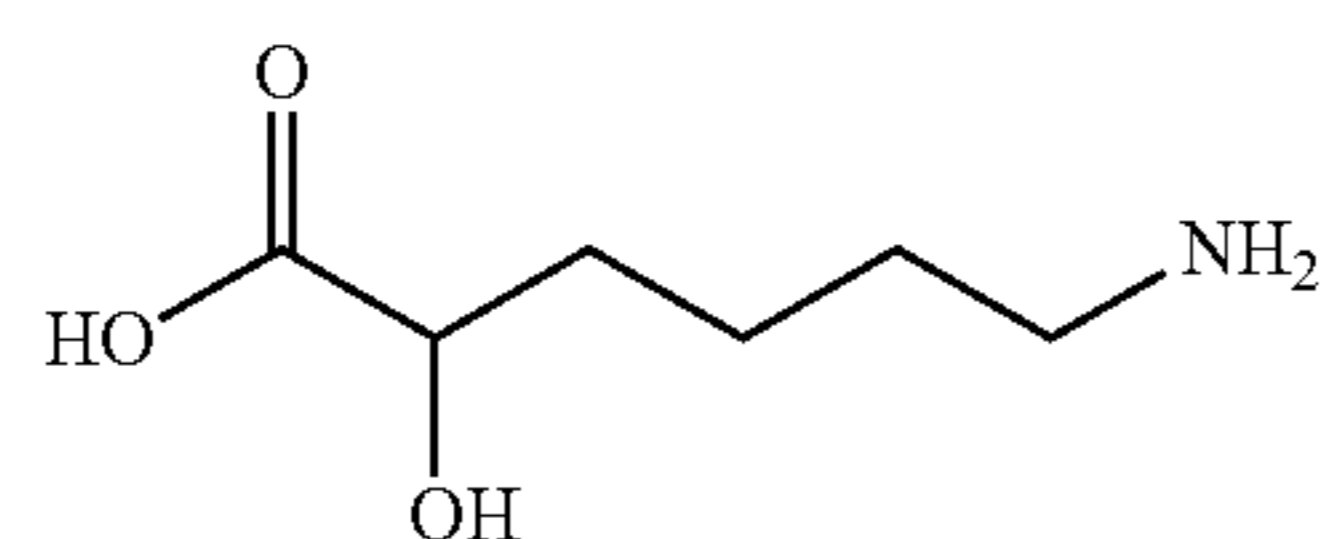
6-amino-2-hydroxyhexanoic acid
