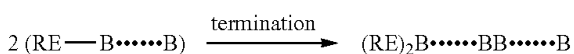
REACTION SCHEME 6:
