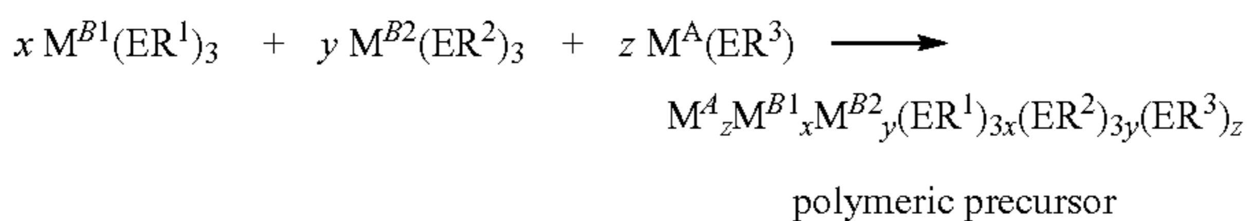
REACTION SCHEME 12:
