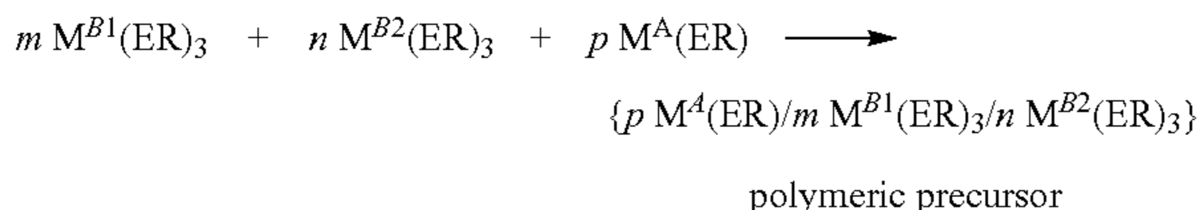
REACTION SCHEME 9:
