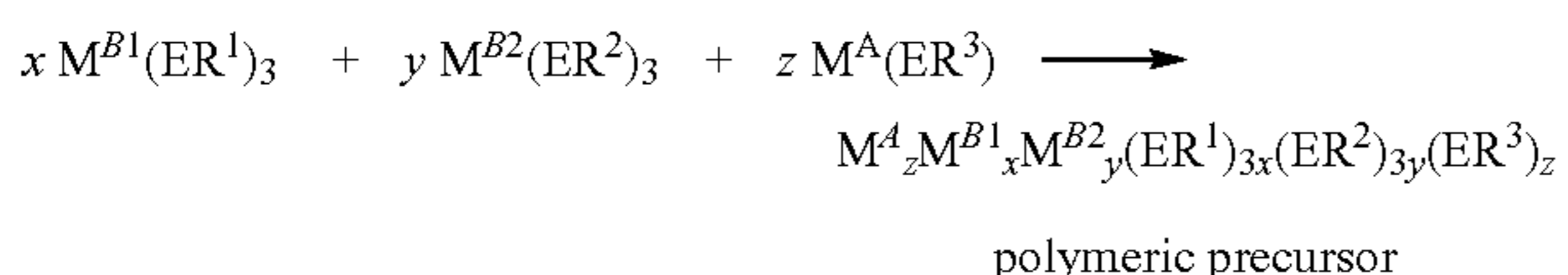
REACTION SCHEME 12:
