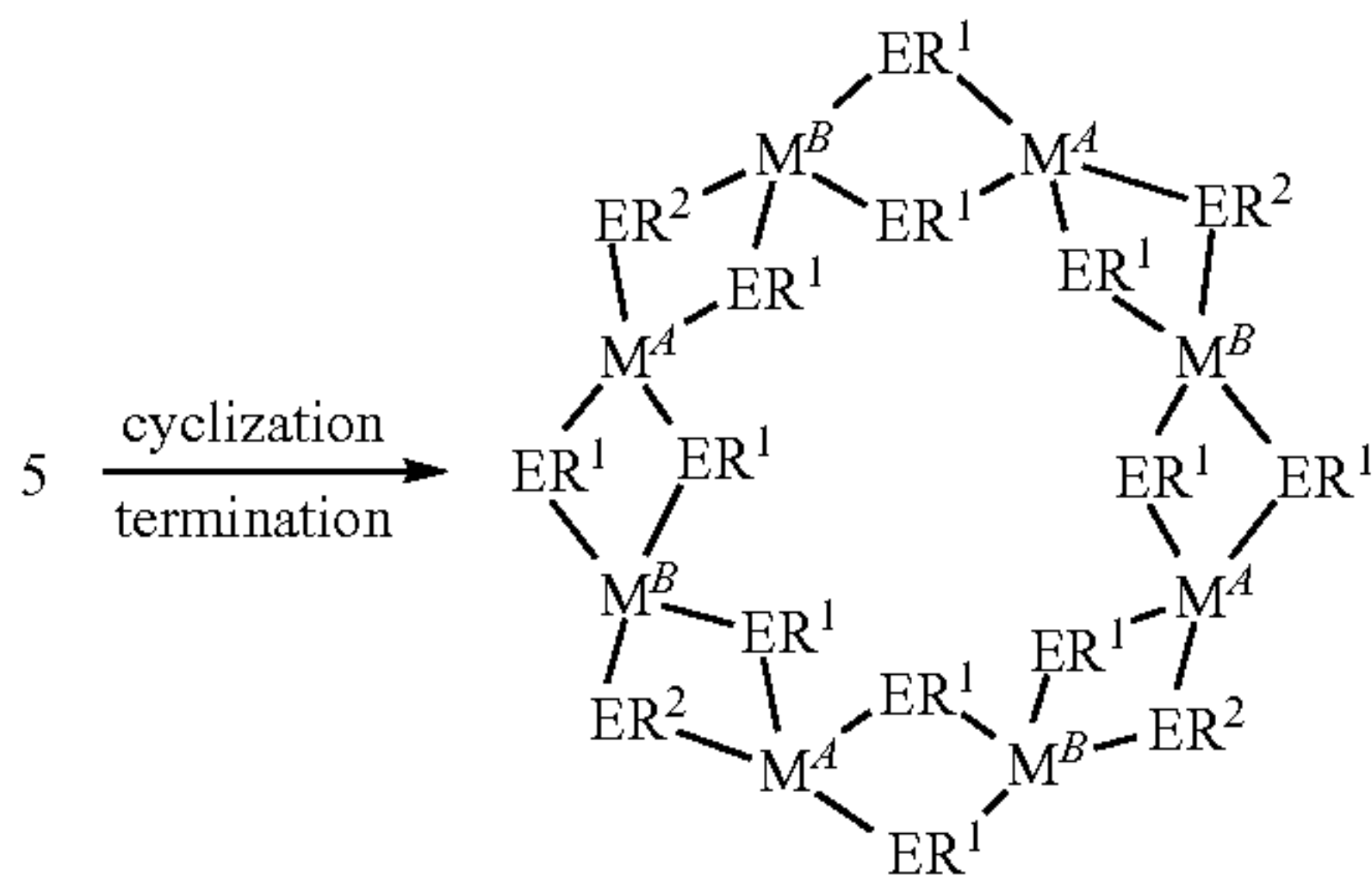
REACTION SCHEME 7:
