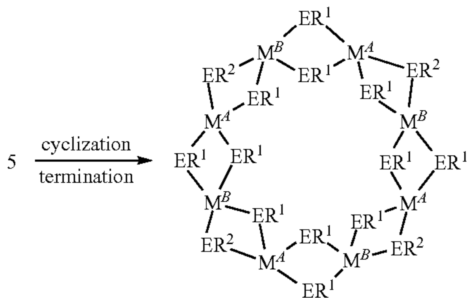
REACTION SCHEME 7:
