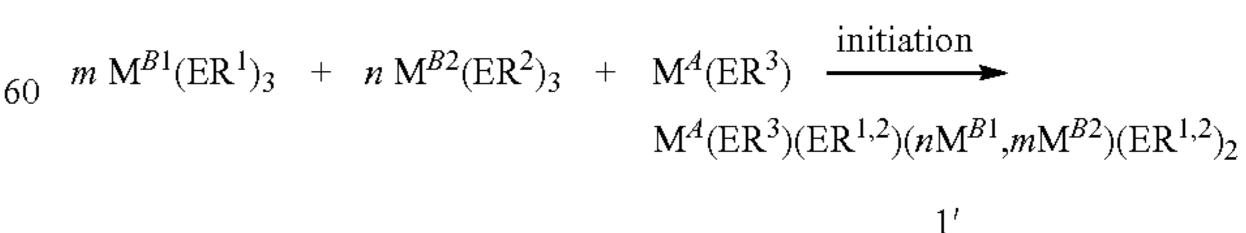
REACTION SCHEME 8:
