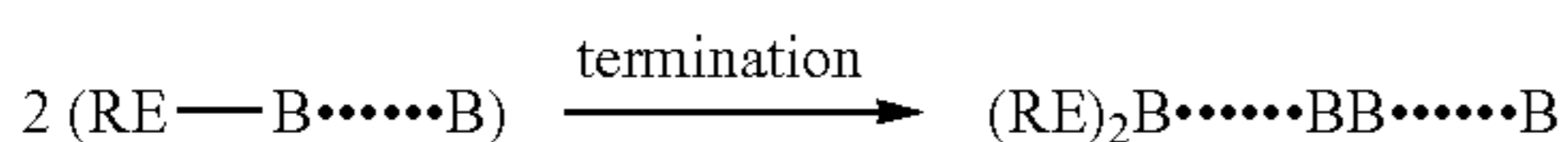
REACTION SCHEME 6:
