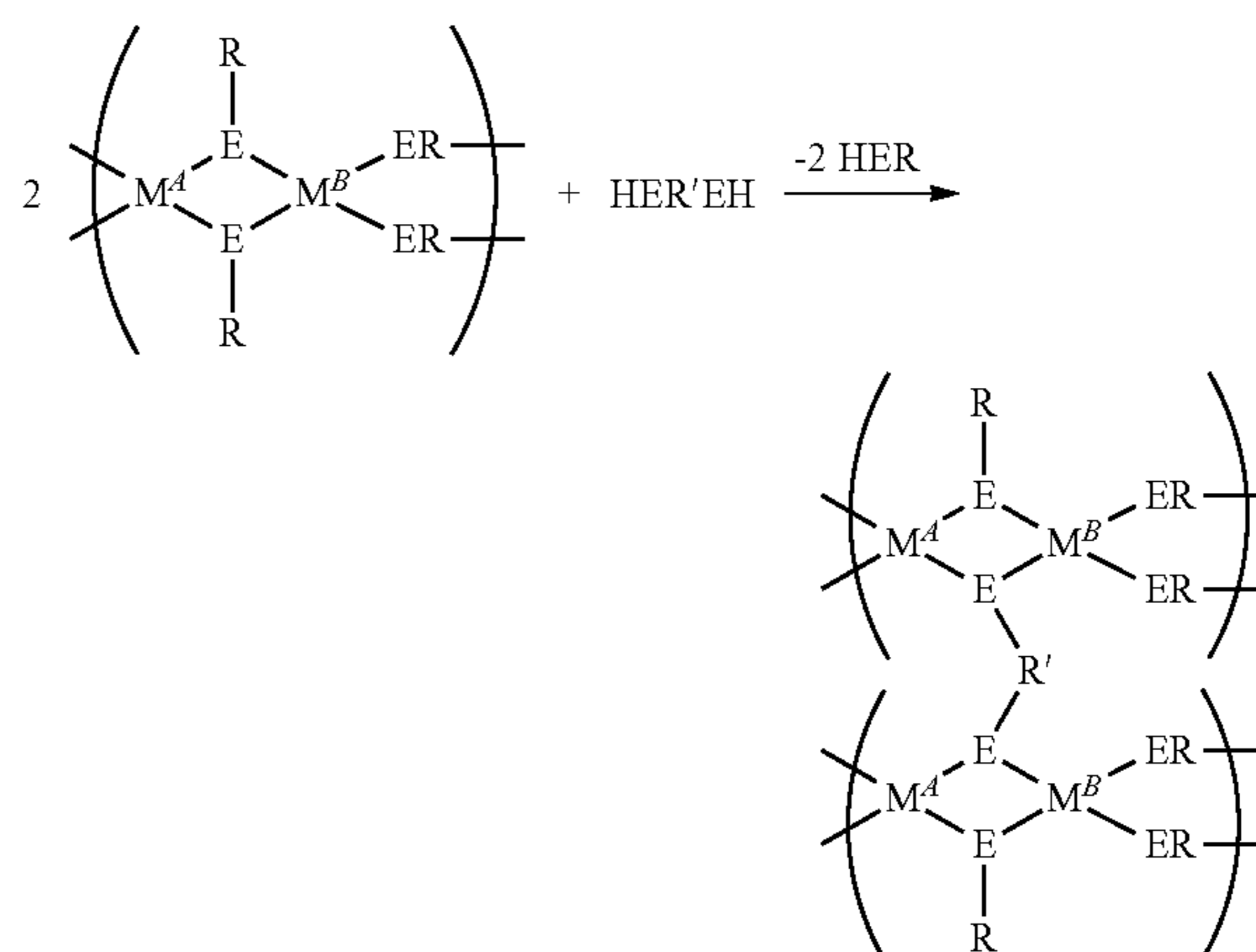
REACTION SCHEME 14
