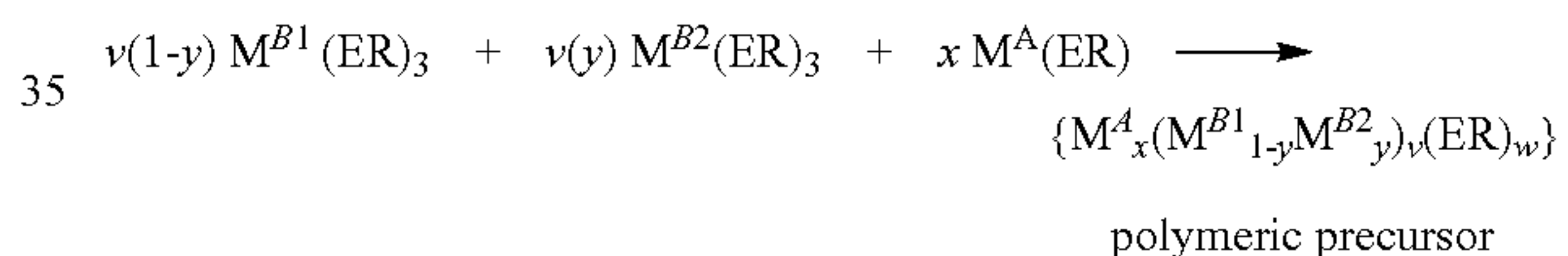
REACTION SCHEME 11:
