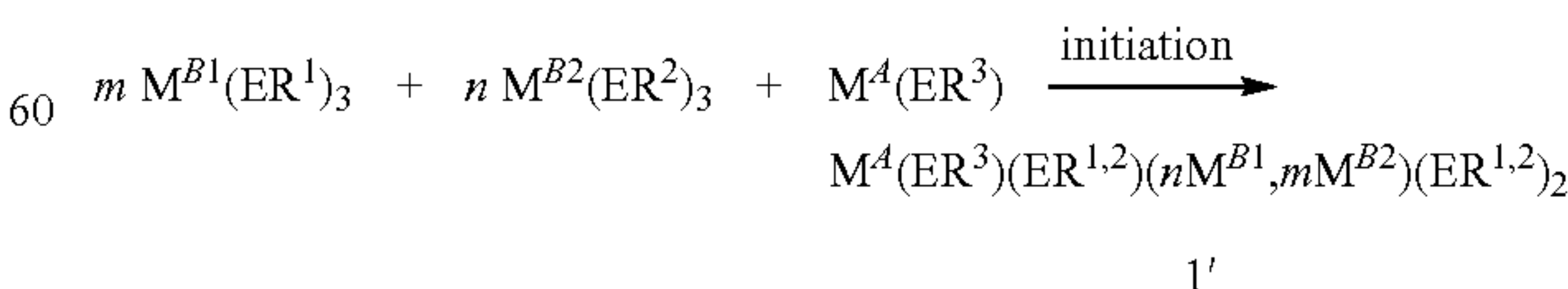
REACTION SCHEME 8:
