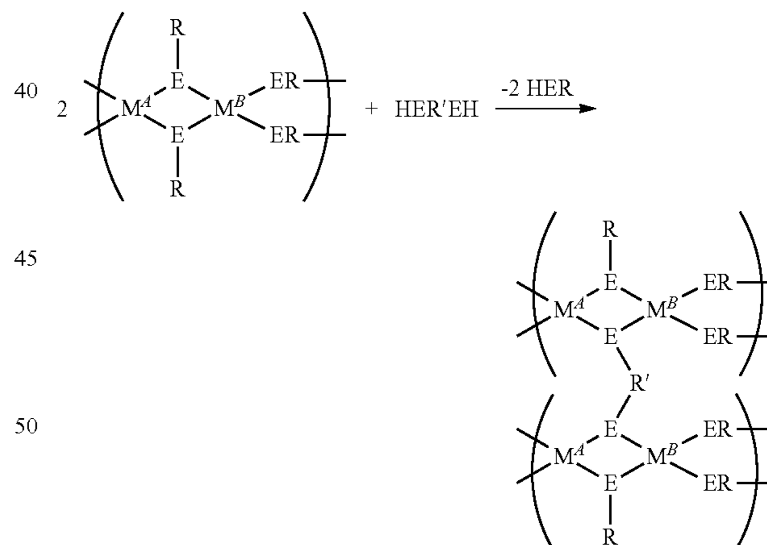
REACTION SCHEME 14
