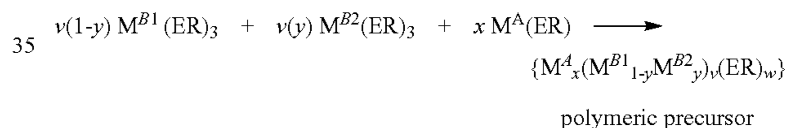
REACTION SCHEME 11:
