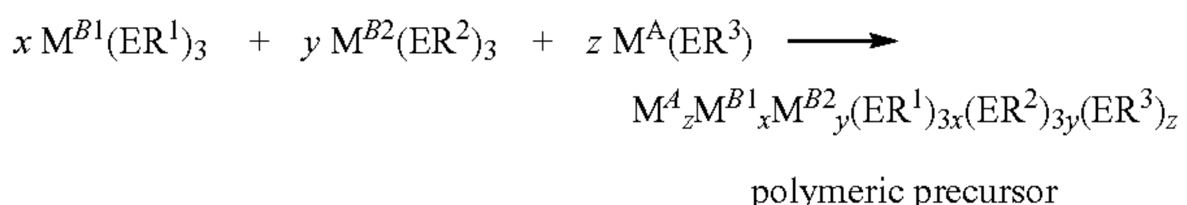
REACTION SCHEME 12:
