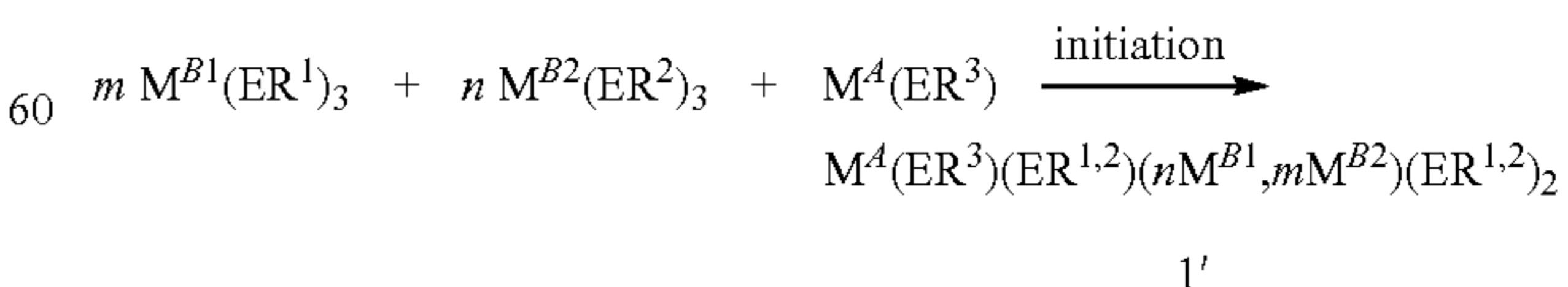
REACTION SCHEME 8:
