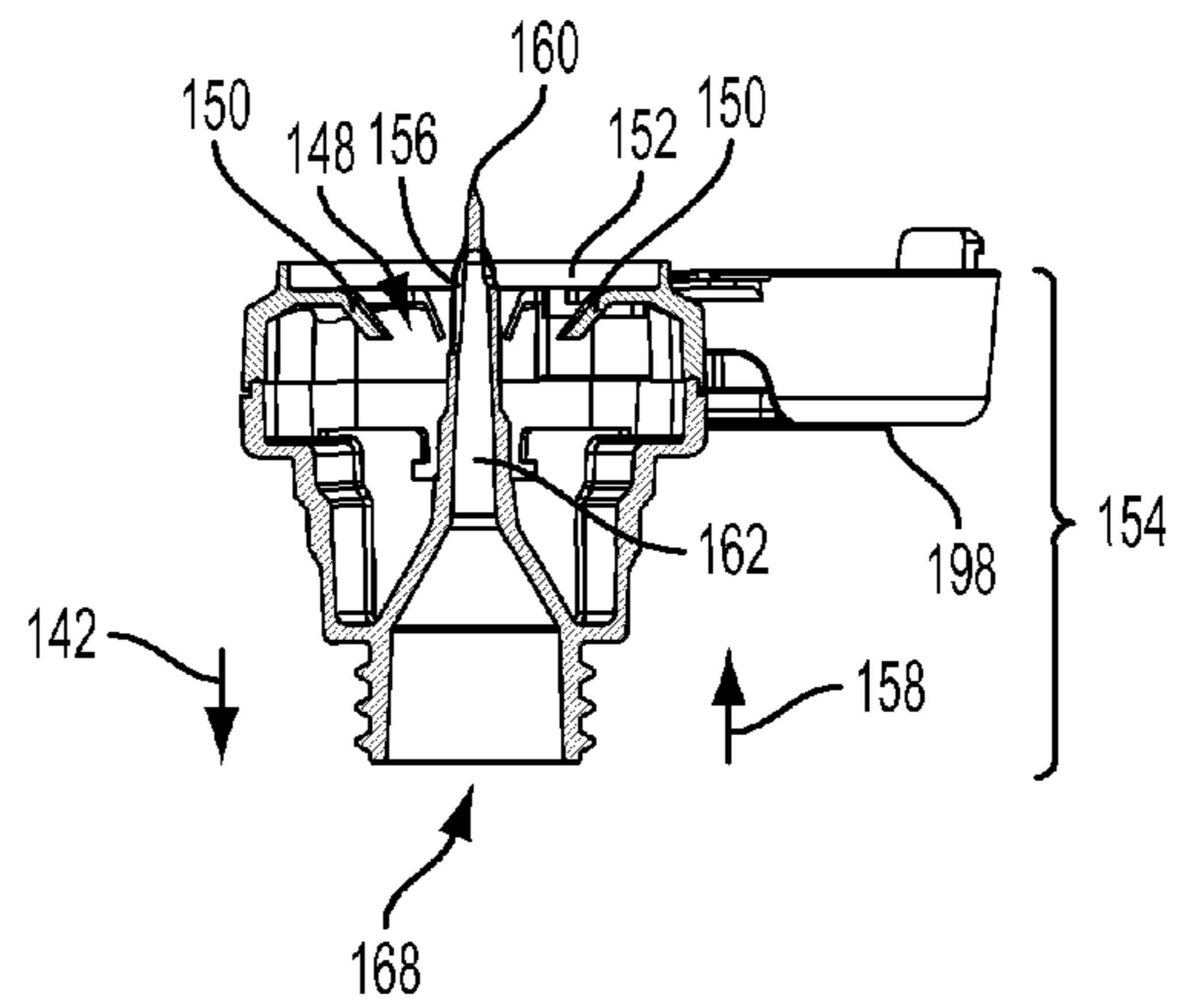
SECTION C - C FIG. 4D
