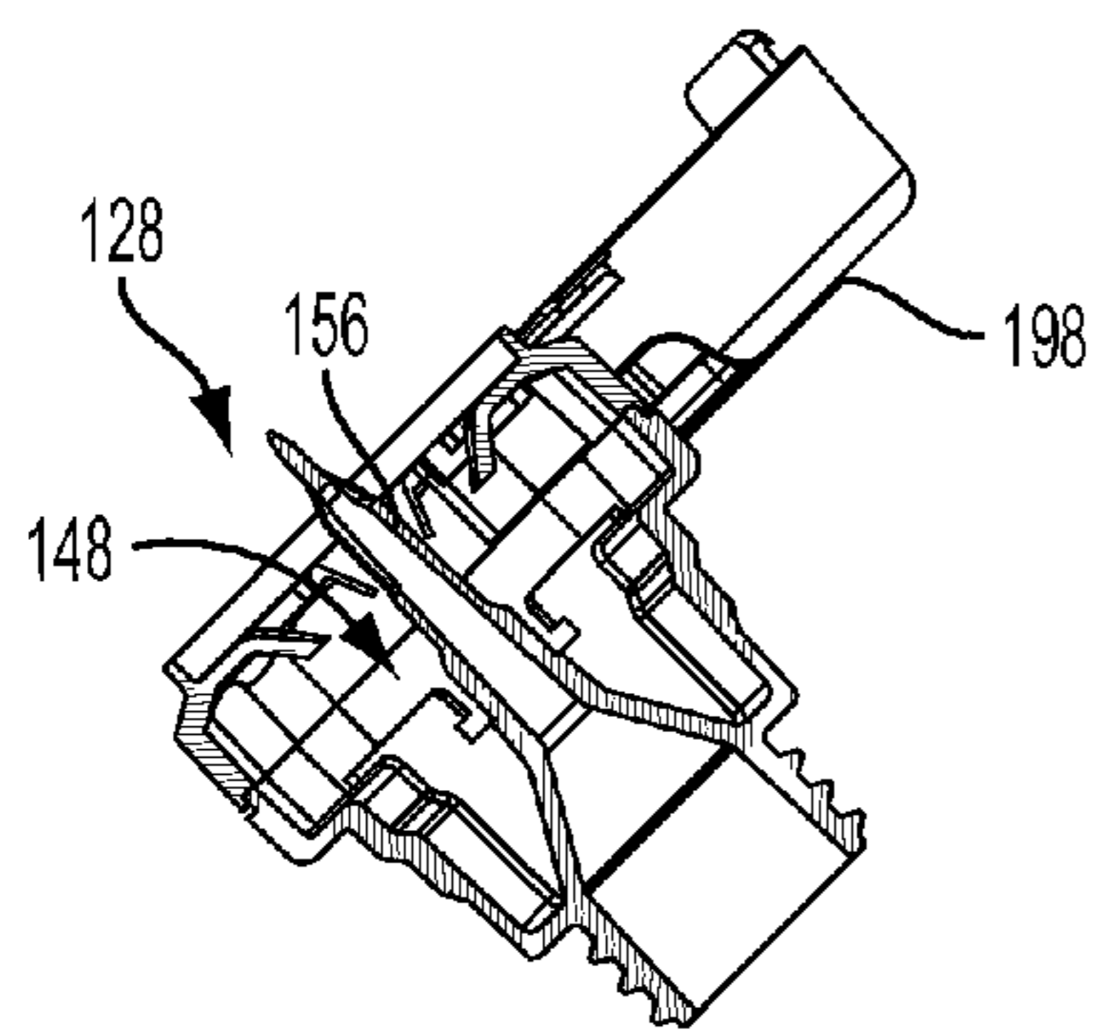
SECTION A - A FIG. 4C
