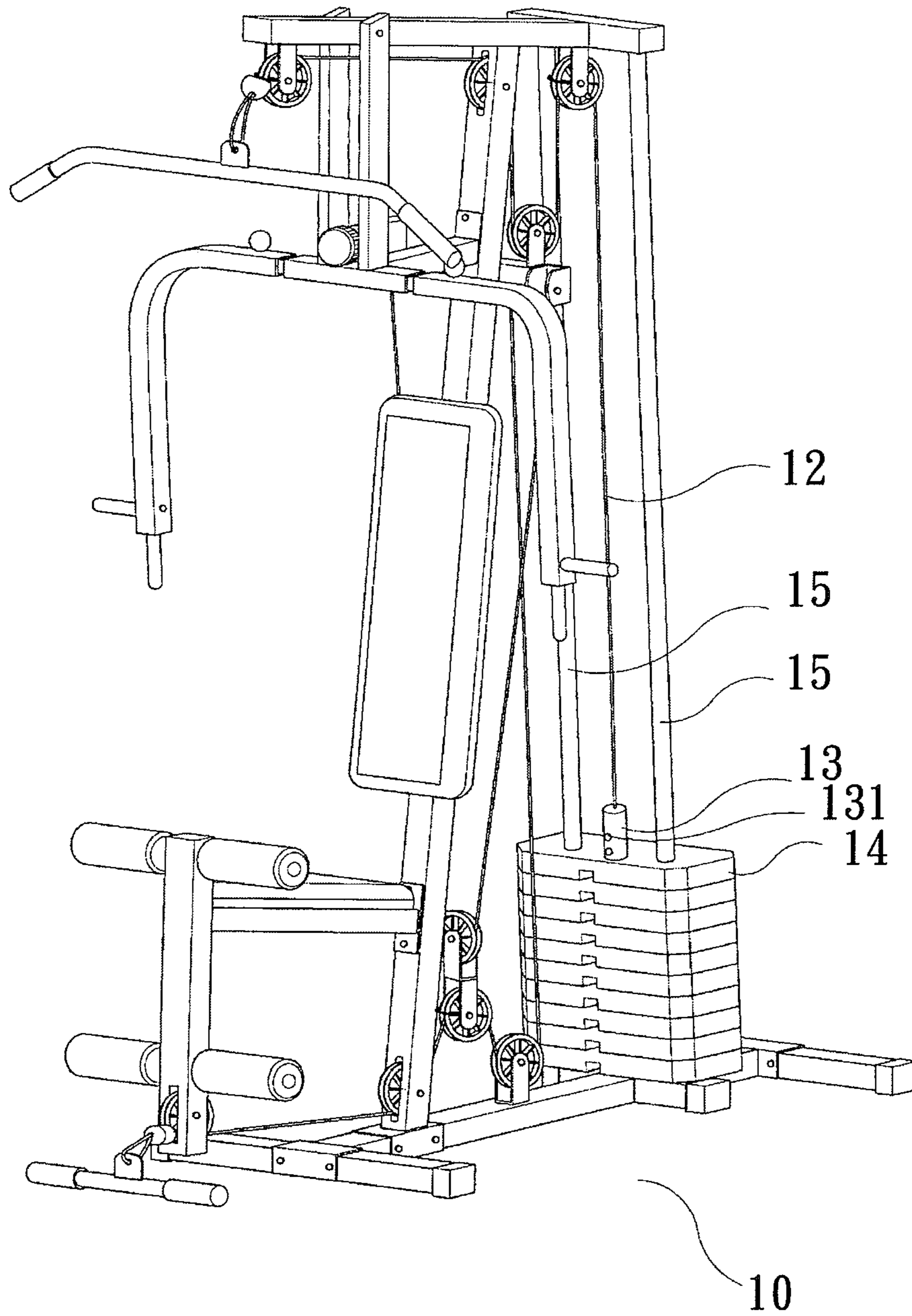
FIG. 1 Prior Art
