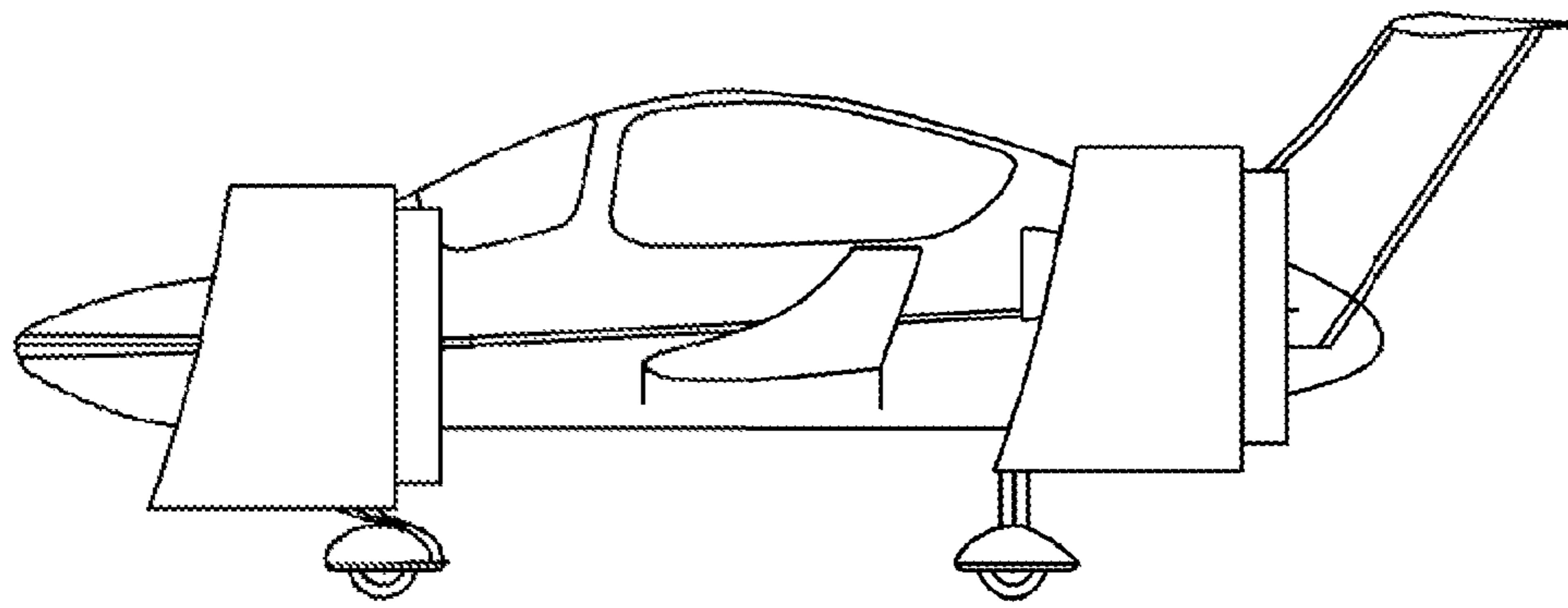
DUCT POSITION-FORWARD FLIGHT WITH FORWARD THRUST
