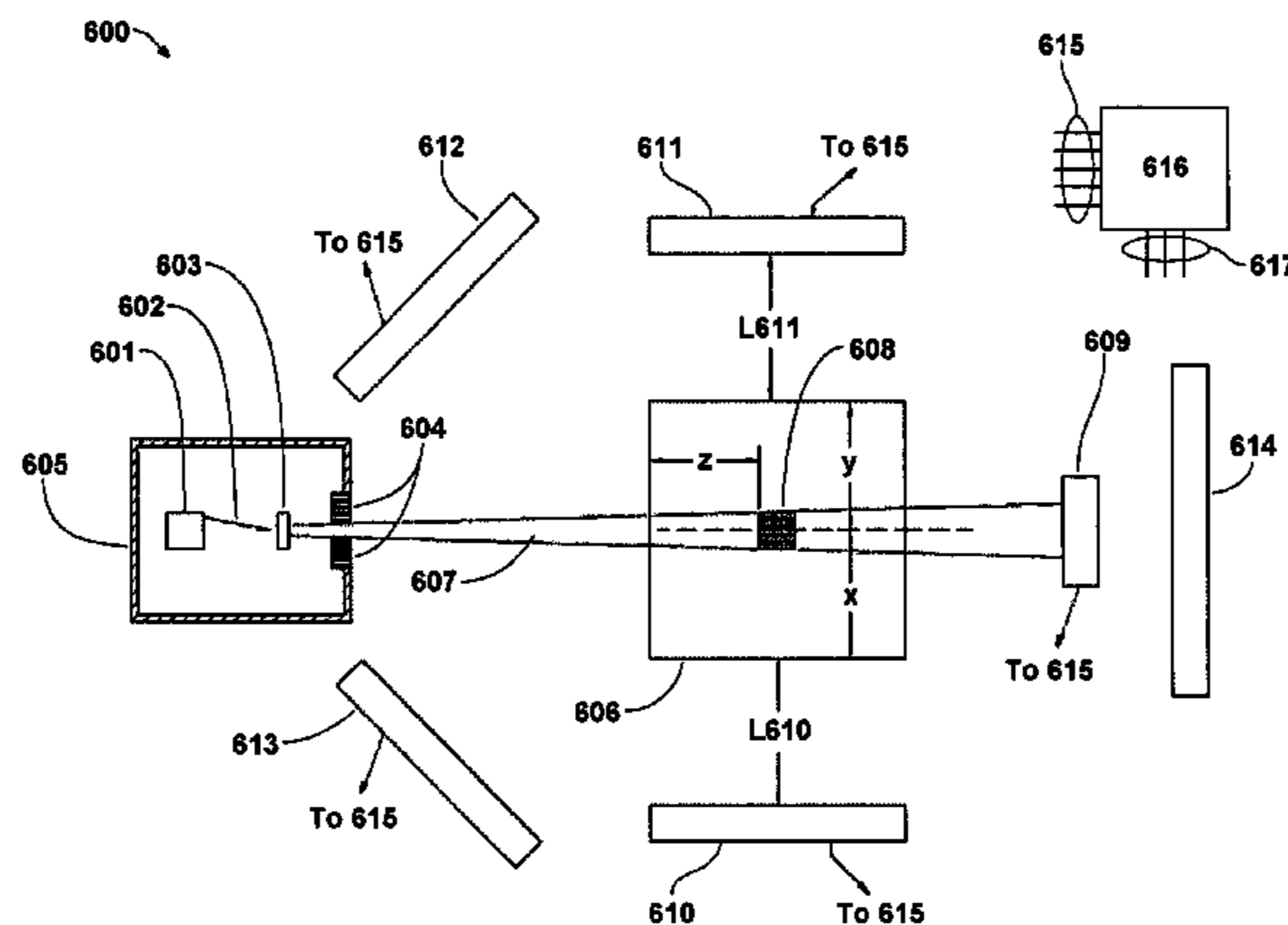
Detector System
