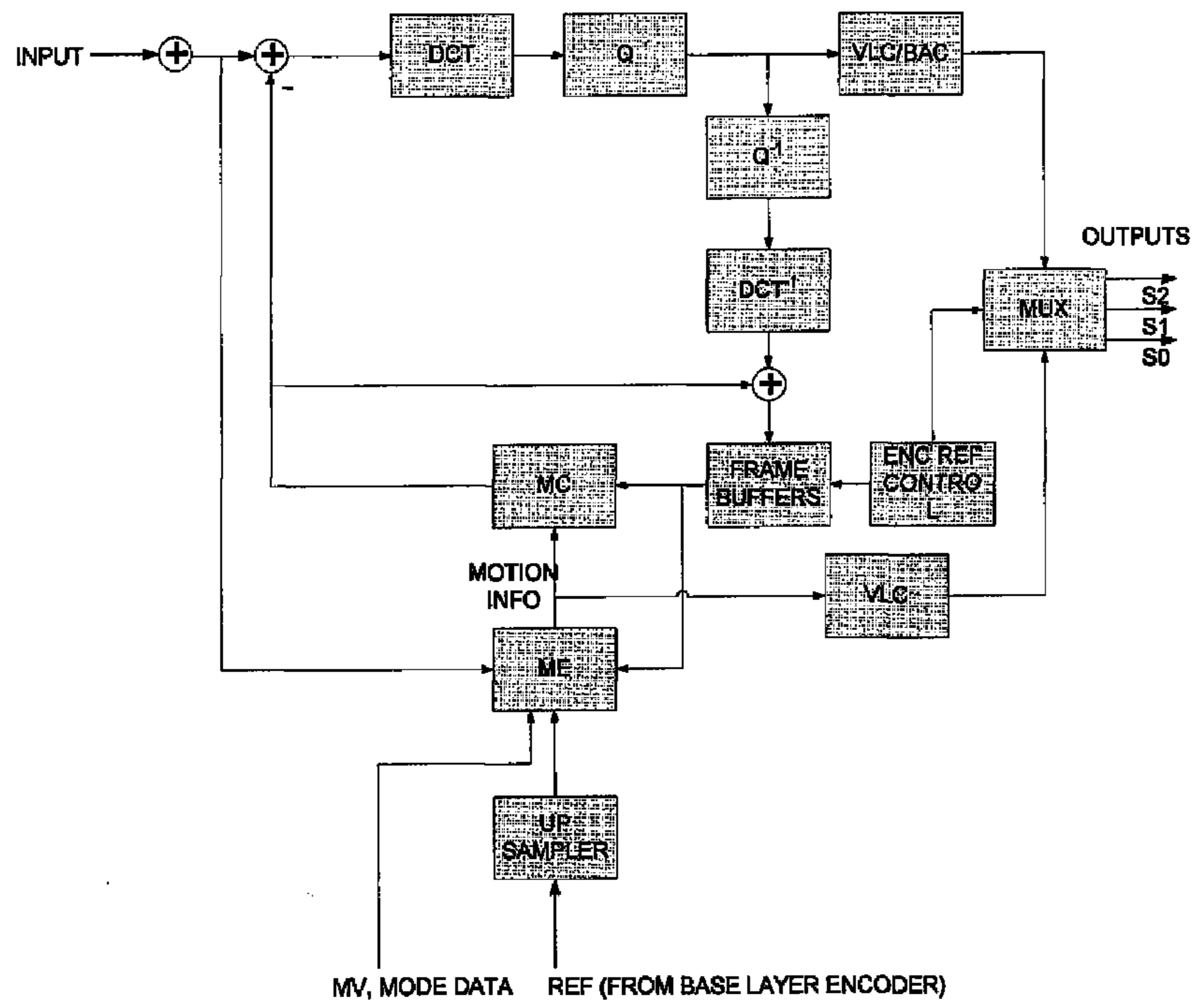
FIG. 6: SPATIAL SCALABILITY ENHANCEMENT LAYER CODEC
