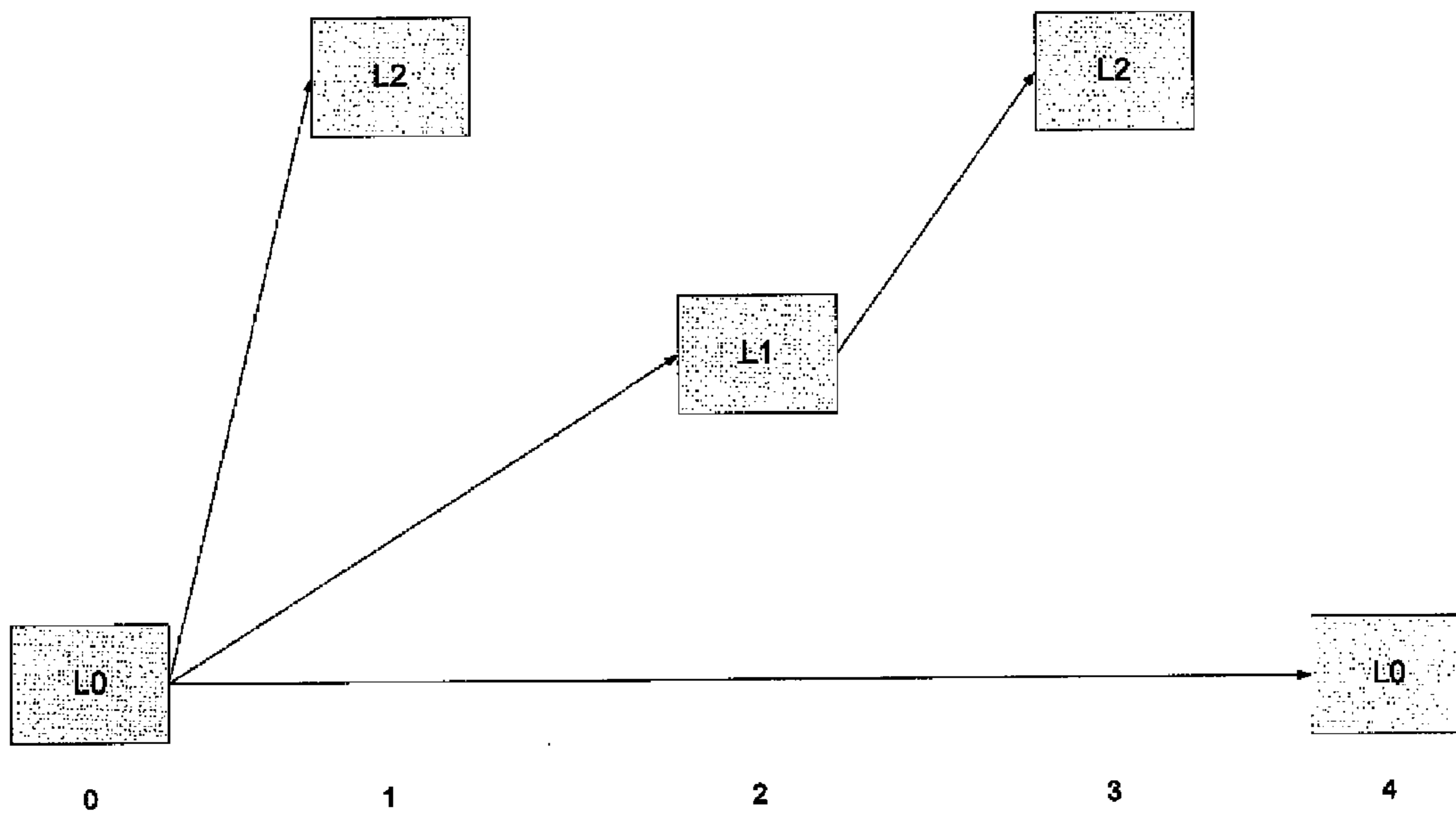
FIG. 4: PICTURE CODING STRUCTURE
