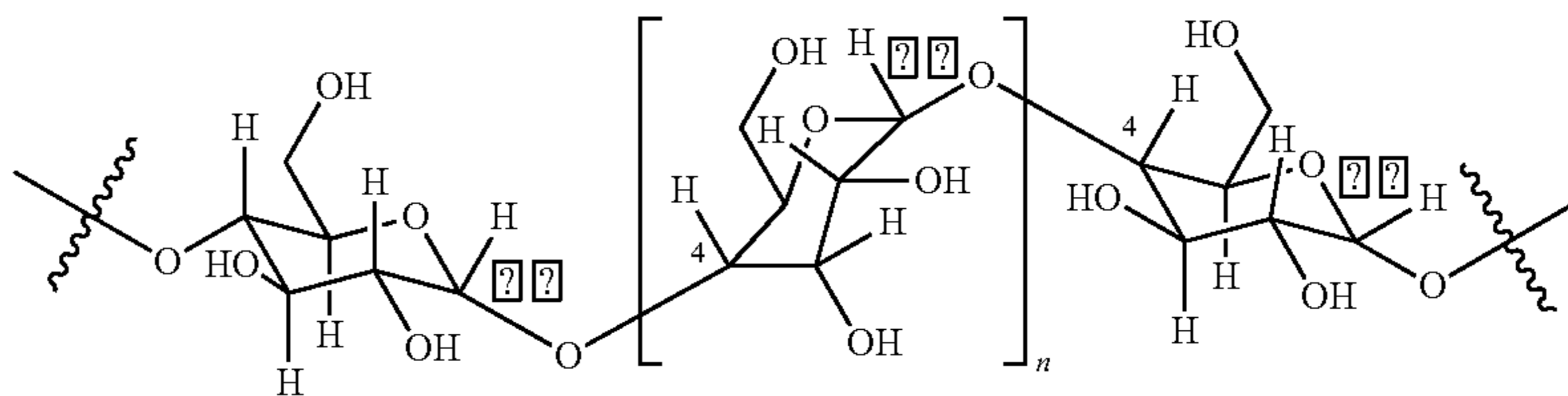
FIG. 2. Representative Partial Structure of Amylose
