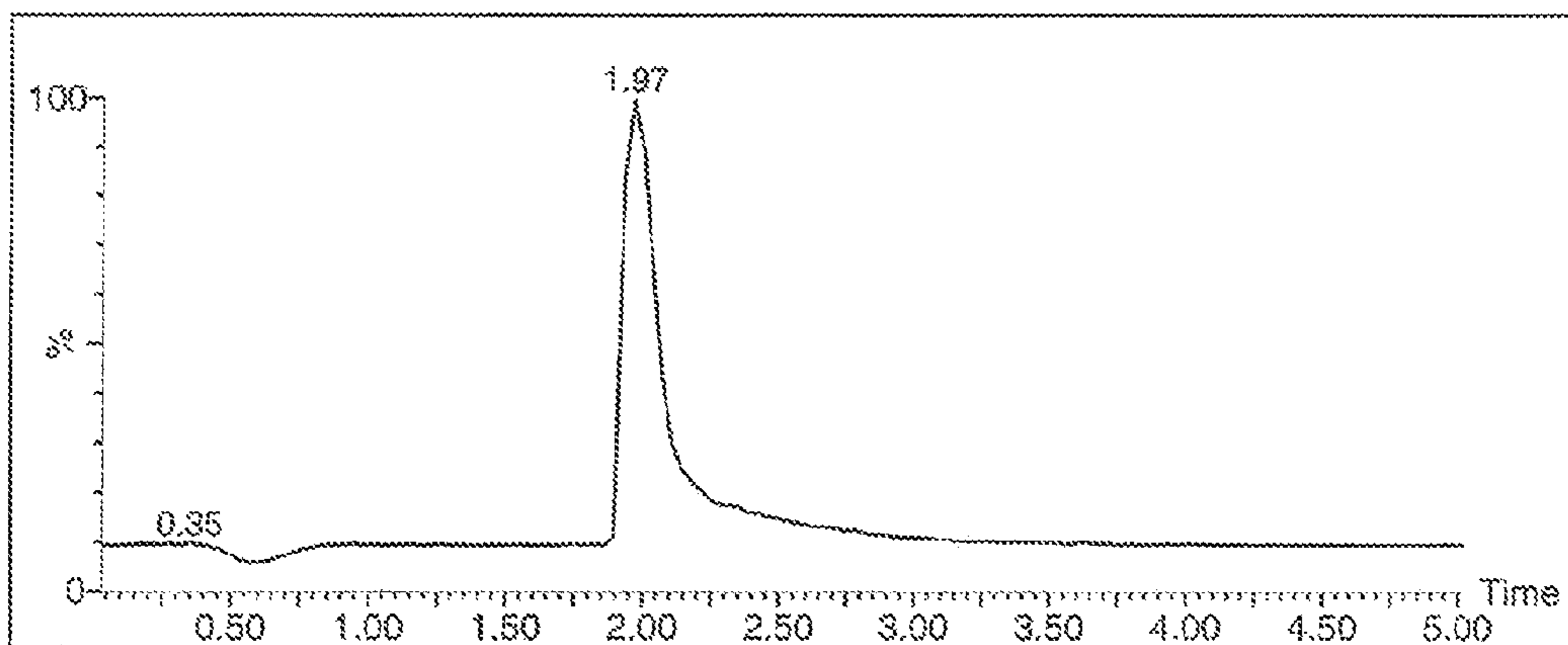
LC Trace - bis-MOM-dehydroequisol
