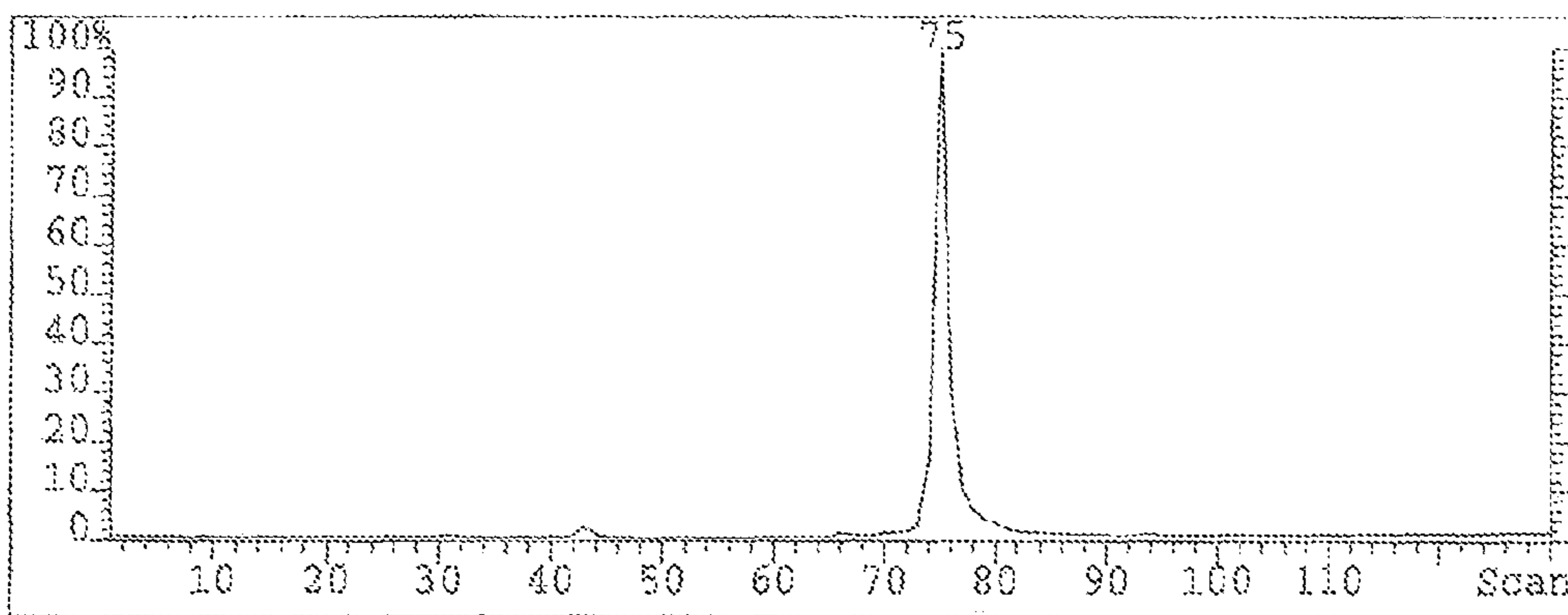
GC Trace - chroman-ol
