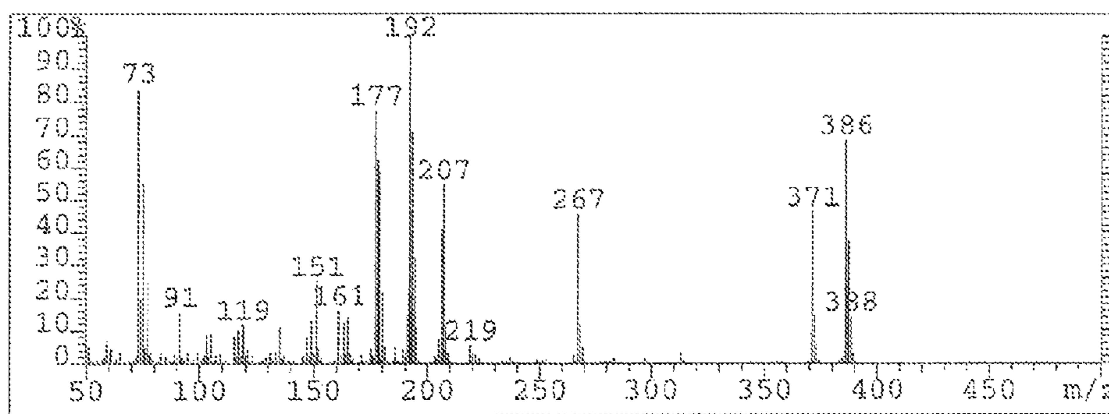
Spectrum - R Equol - TMS Derivative
