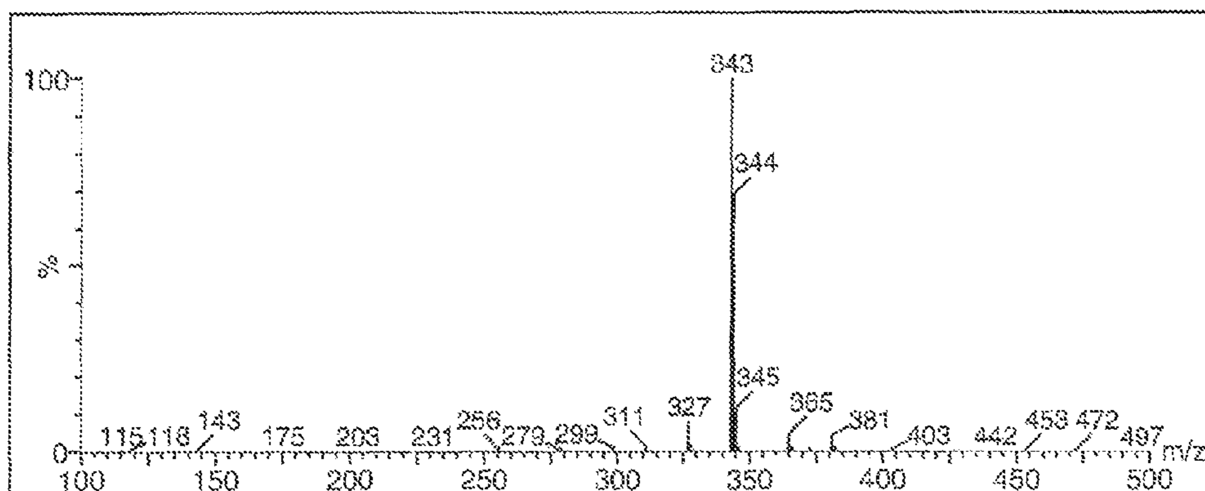
Spectrum - bis-MOM Daidzein
