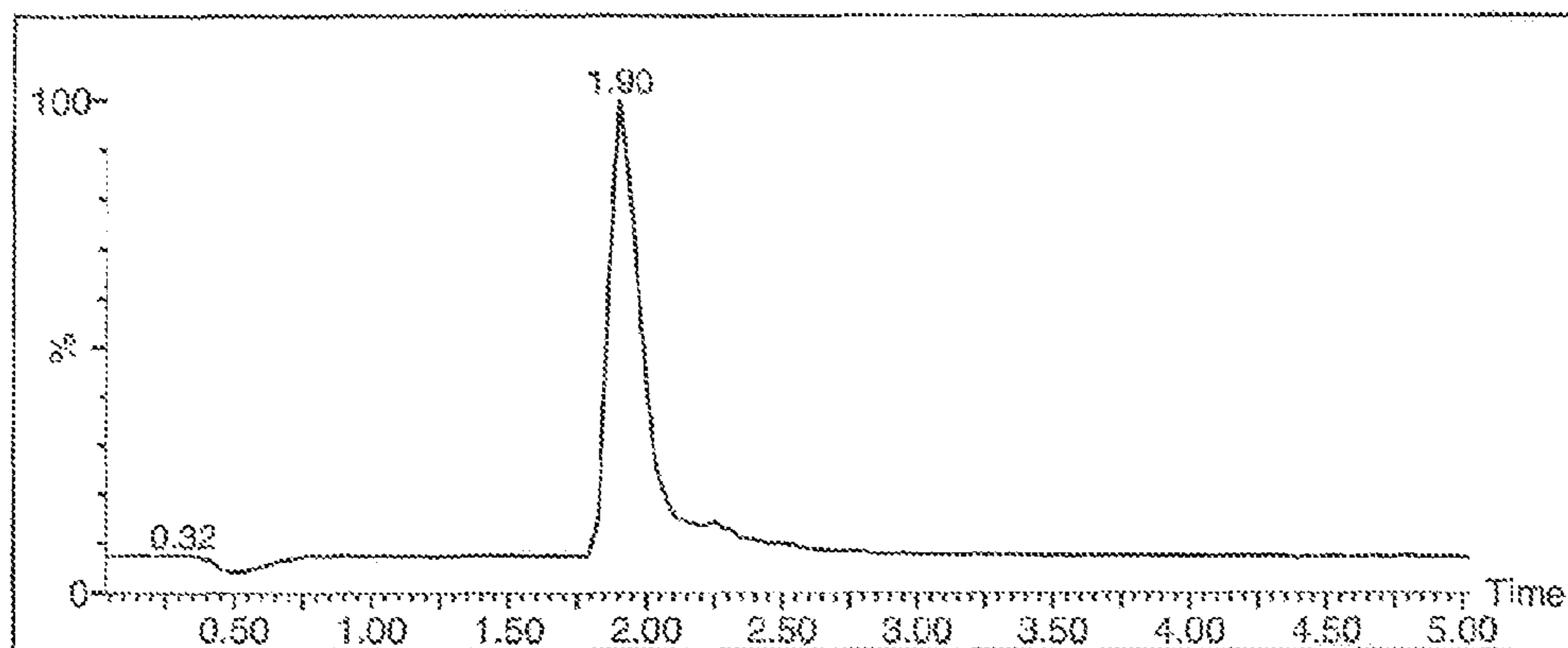
LC Trace - bis-MOM Daidzein
