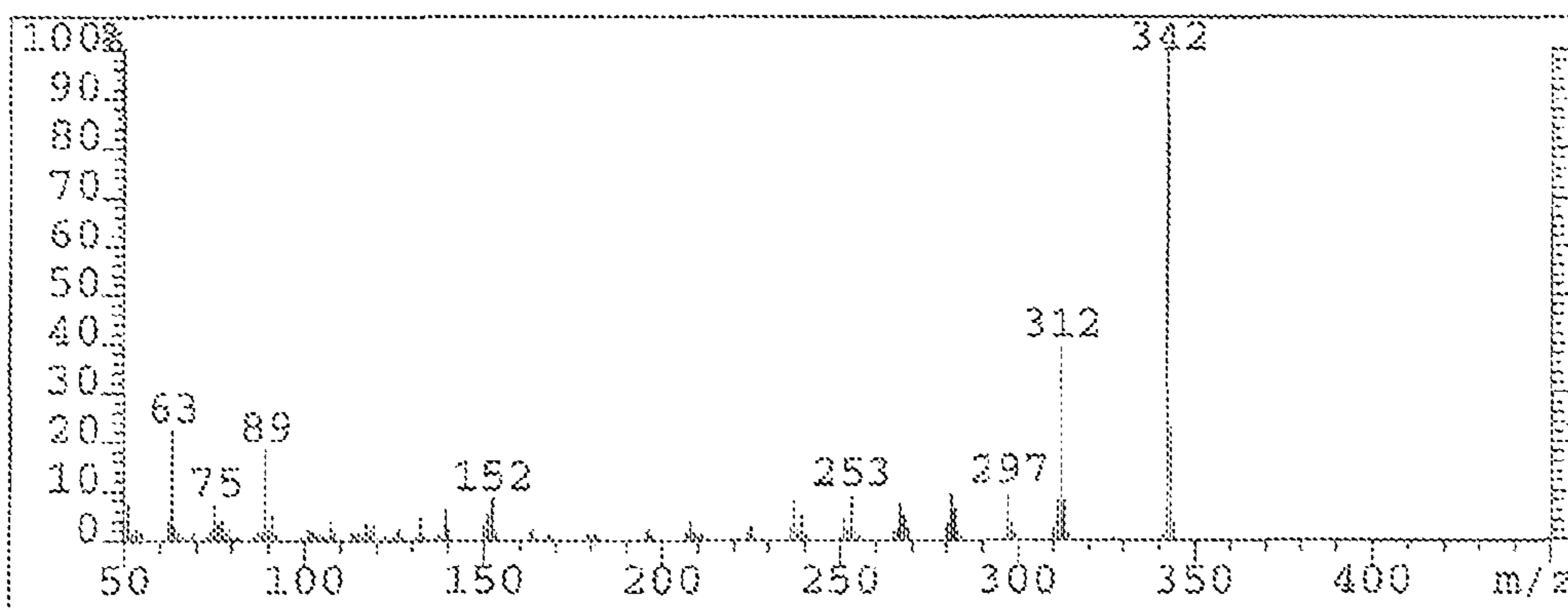
Spectrum - bis-MOM Daidzein
