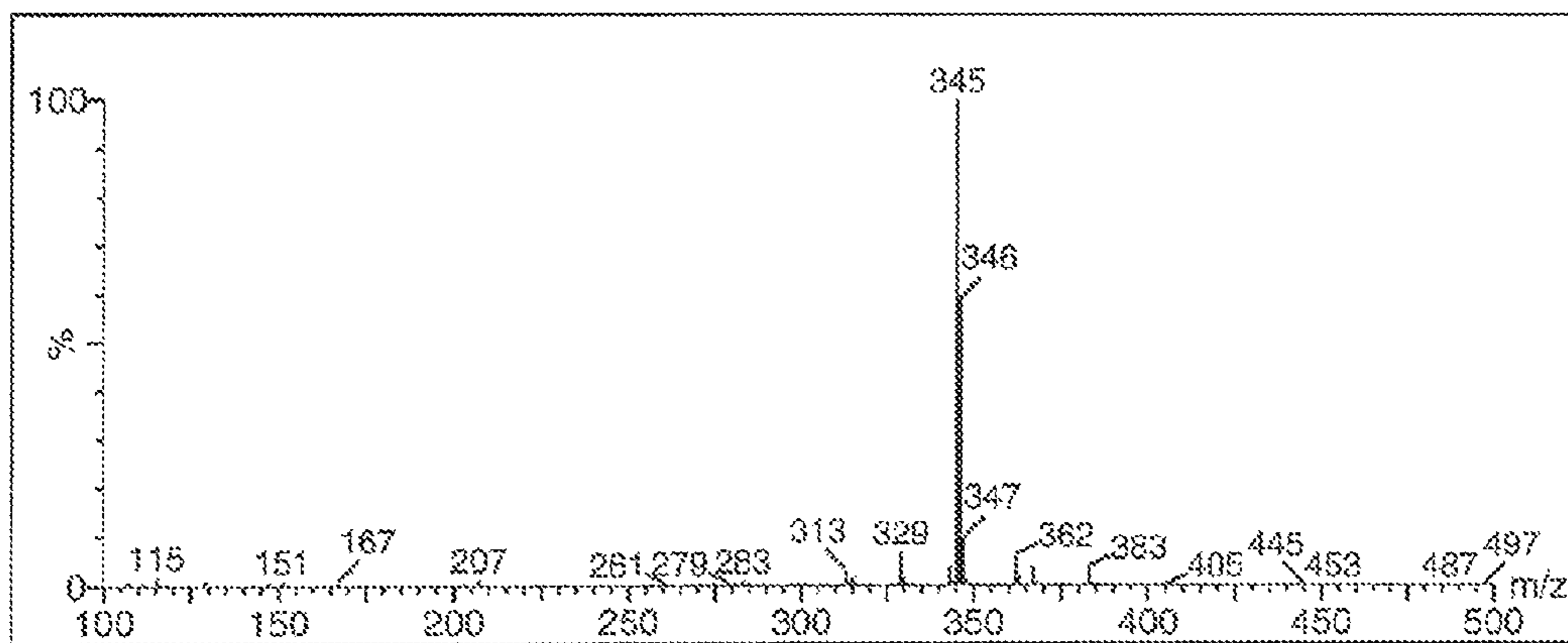
Spectrum - chroman-4-one
