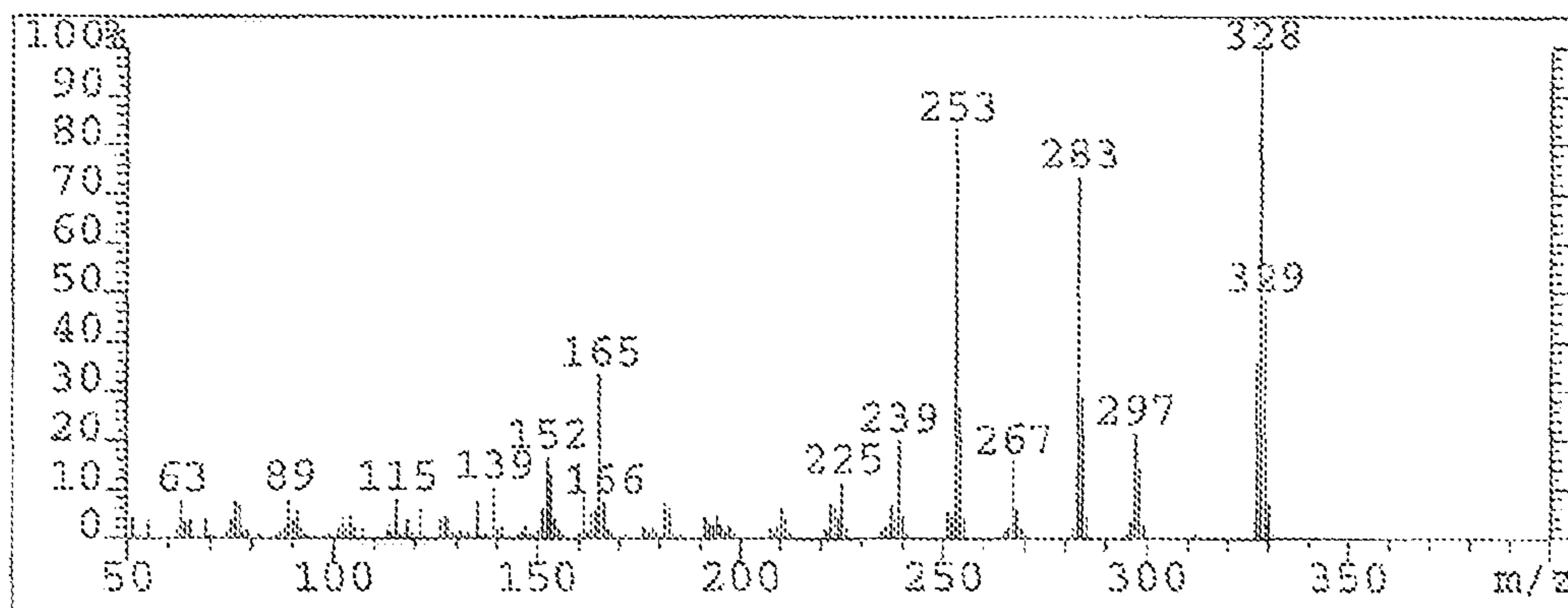
Spectrum - bis-MOM-dehydroequisol
