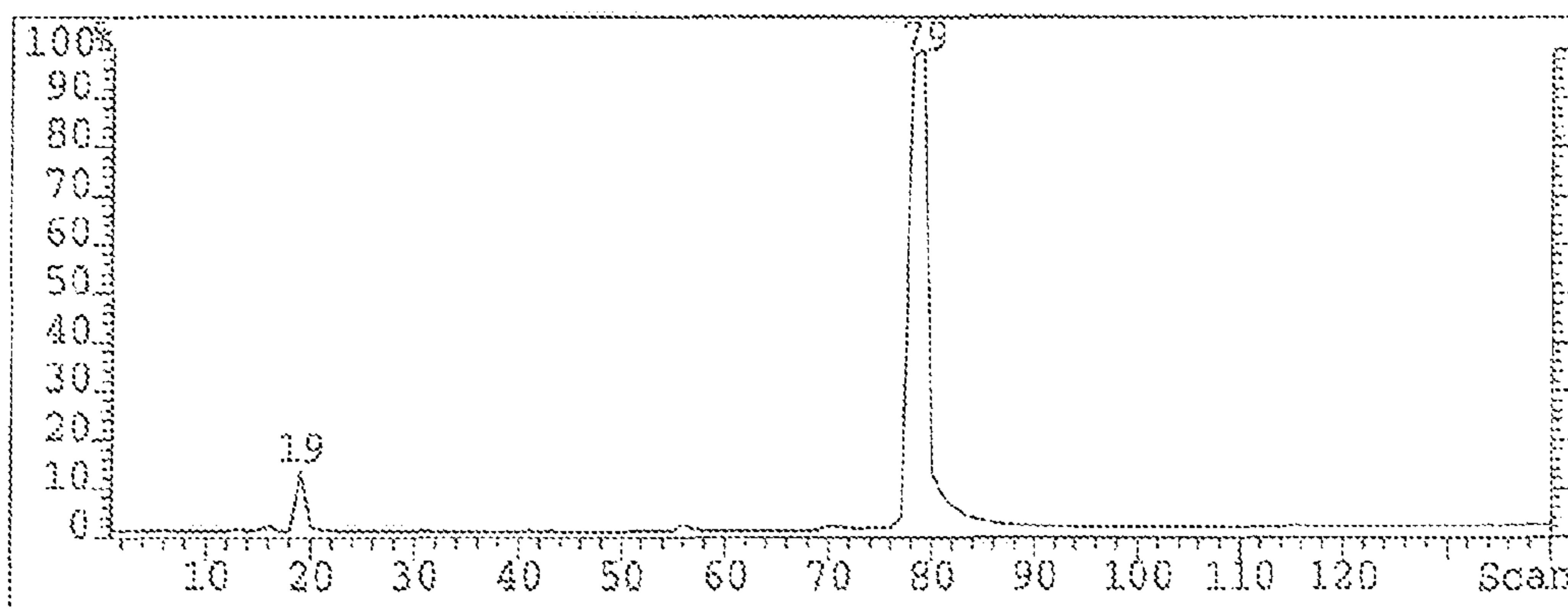
GC Trace - bis-MOM Daidzein
