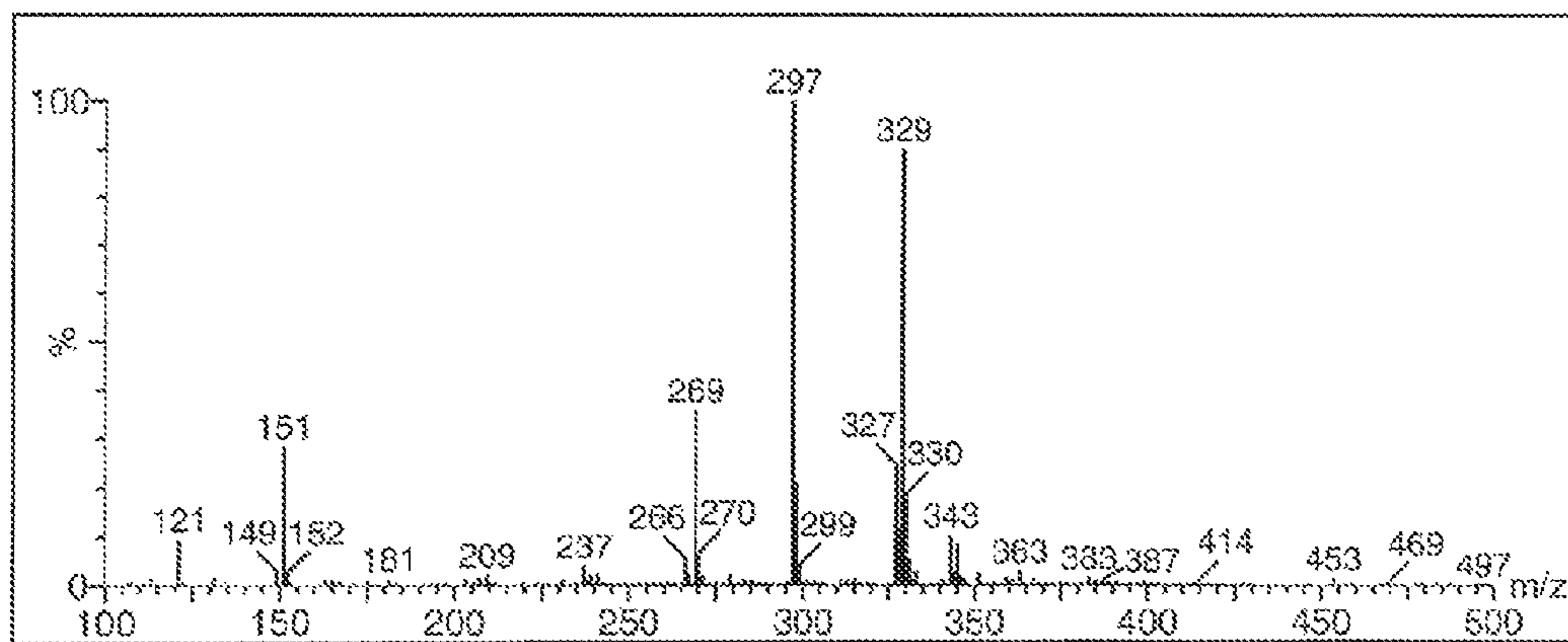
Spectrum - bis-MOM-dehydroequisol
