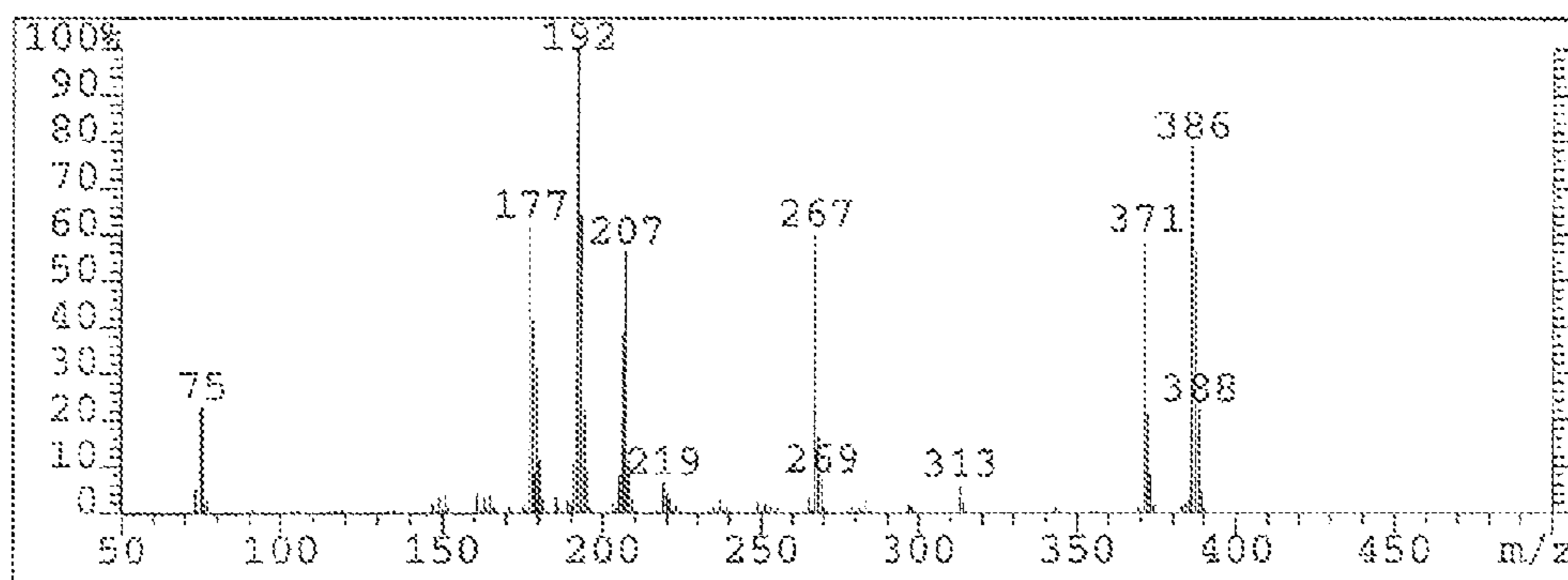
Spectrum - S Equol - TMS Derivative
