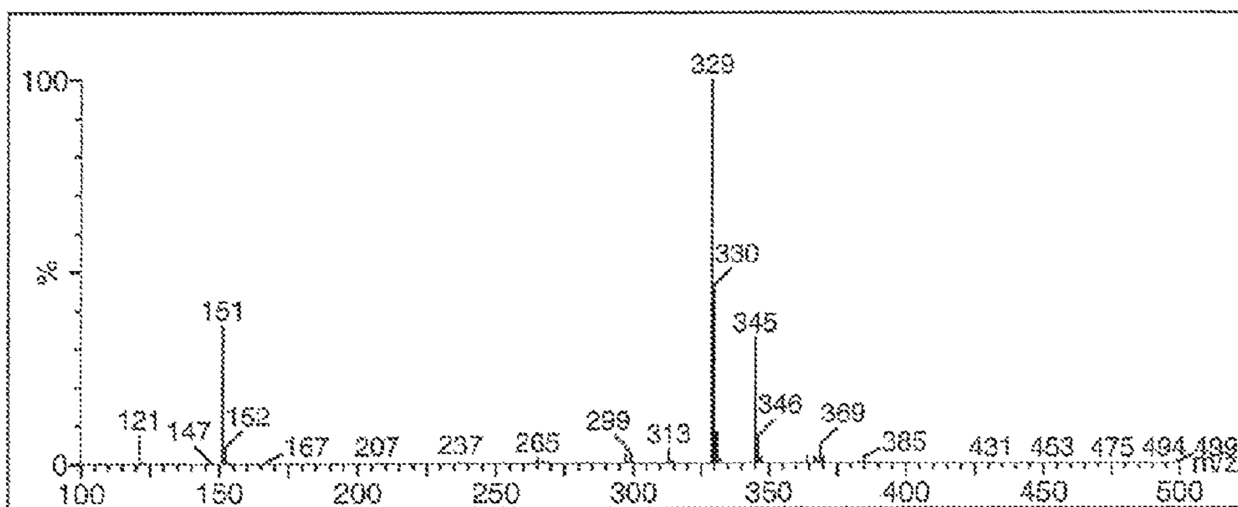
Spectrum - chroman-ol
