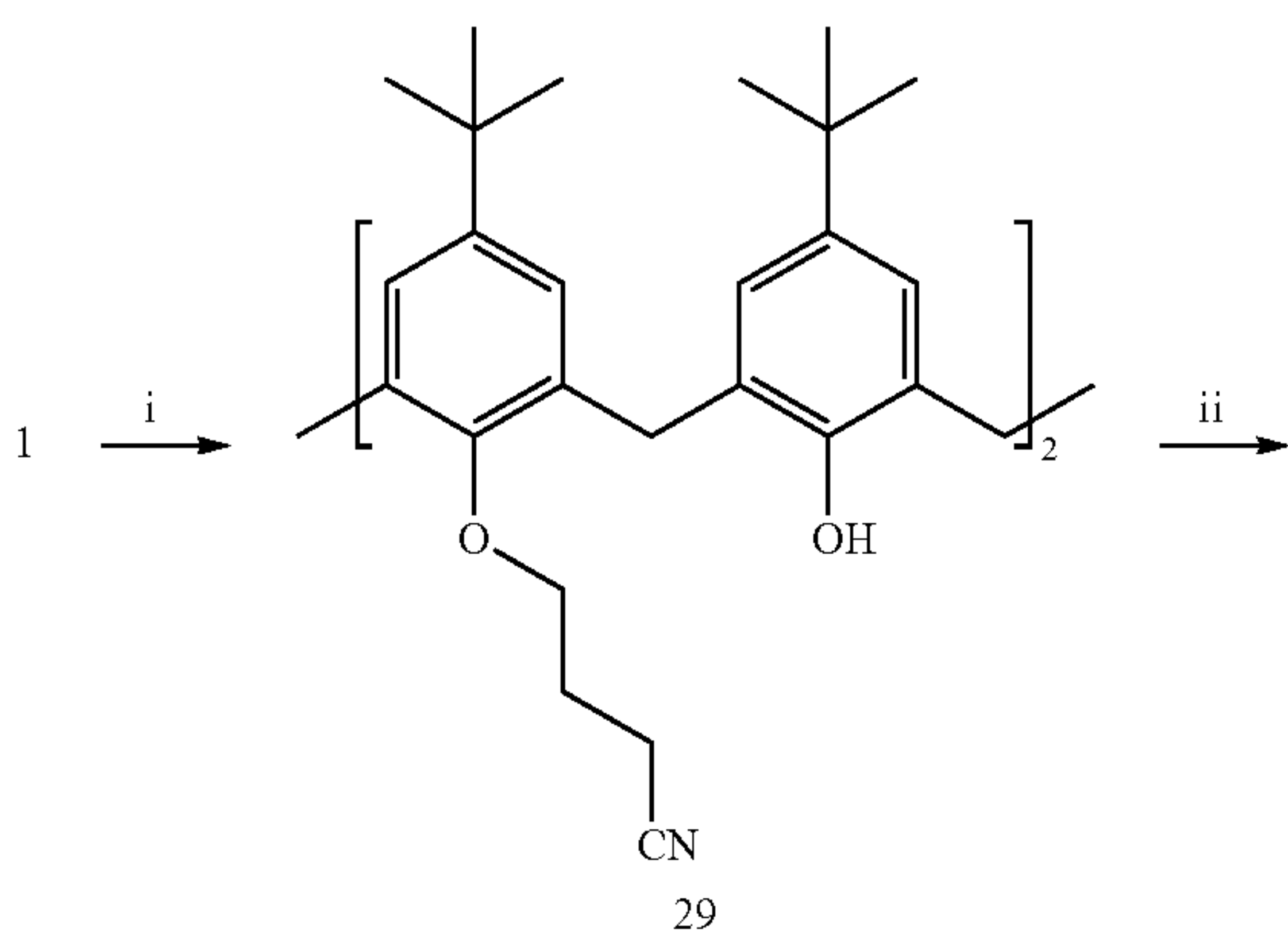
Scheme 7
