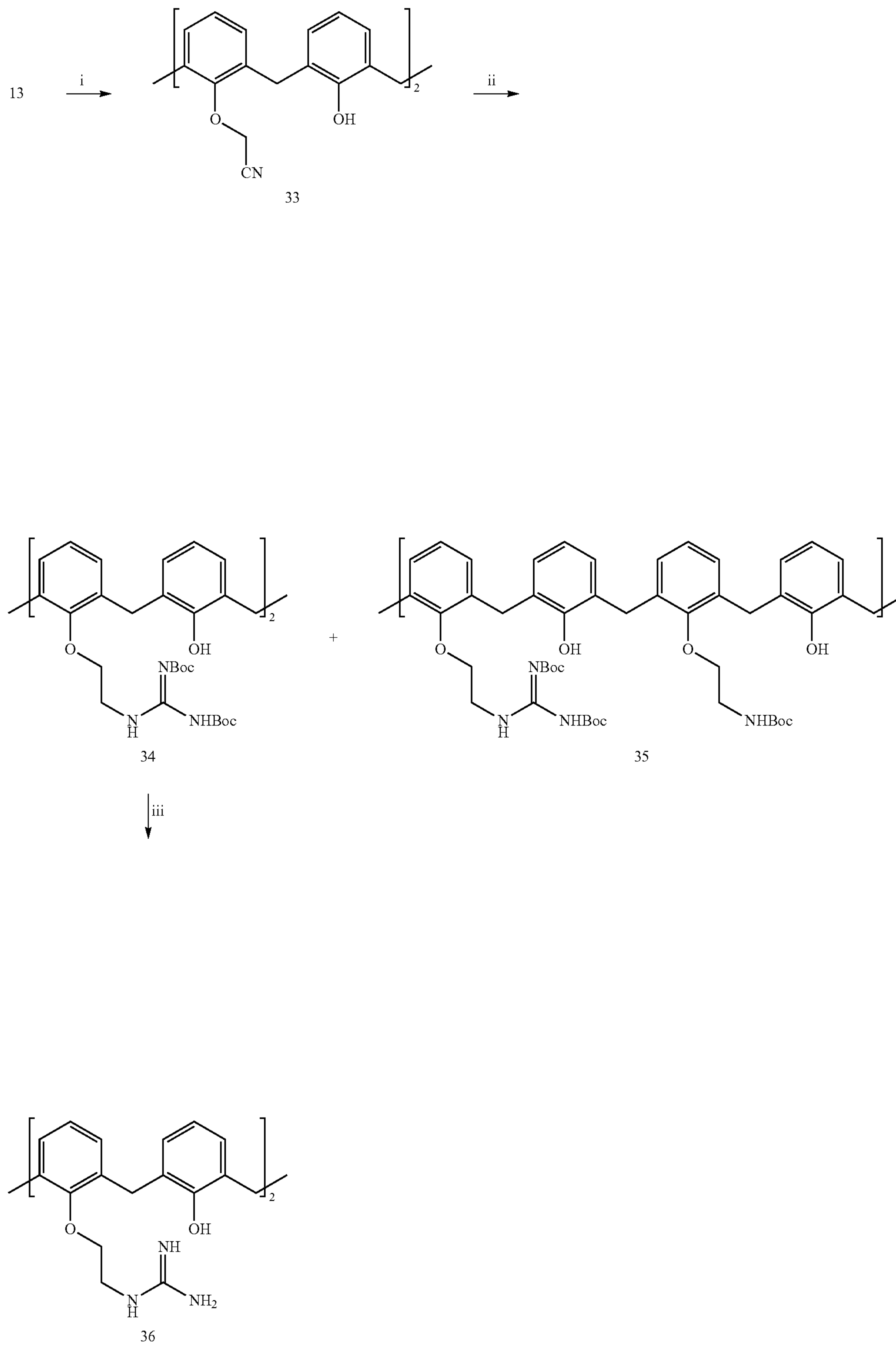
Scheme 8
