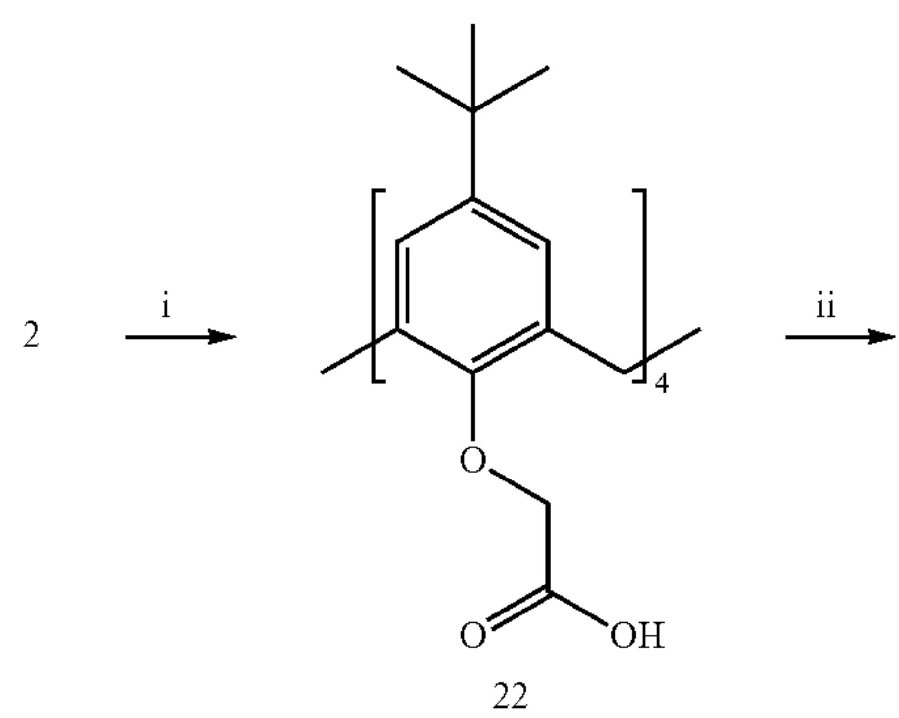
Scheme 5
