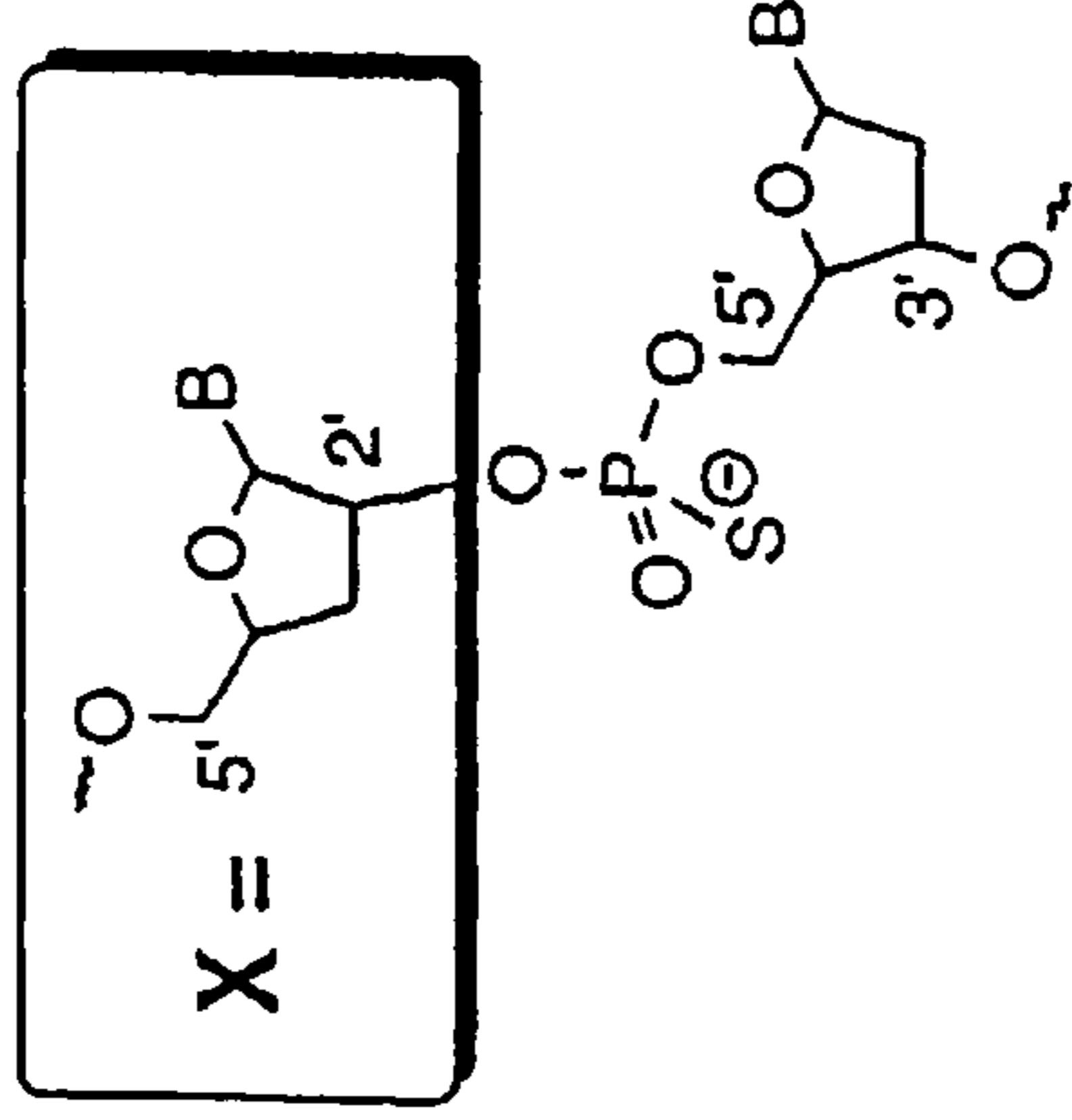
3'-Deoxynucleoside
