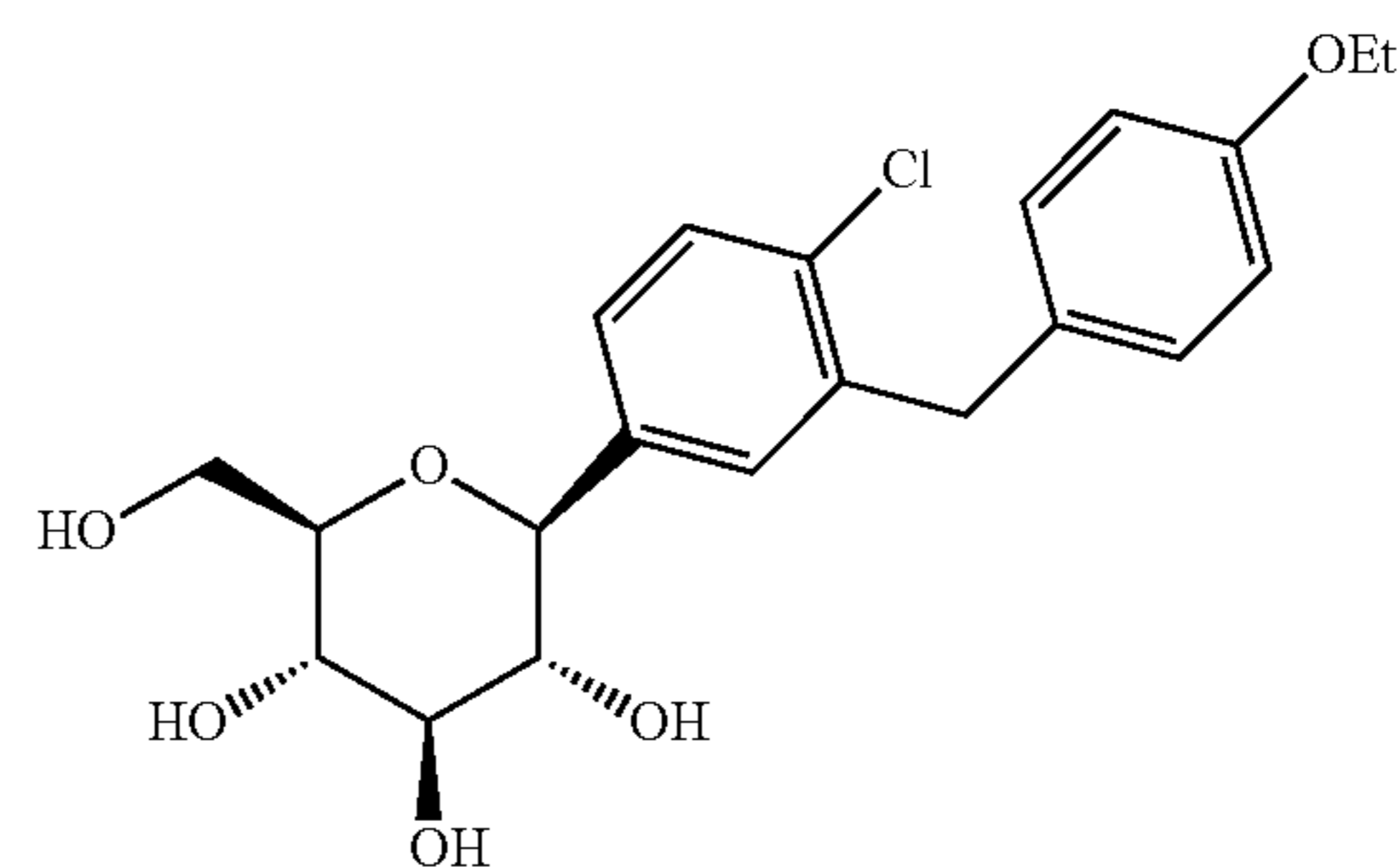
Compound I
