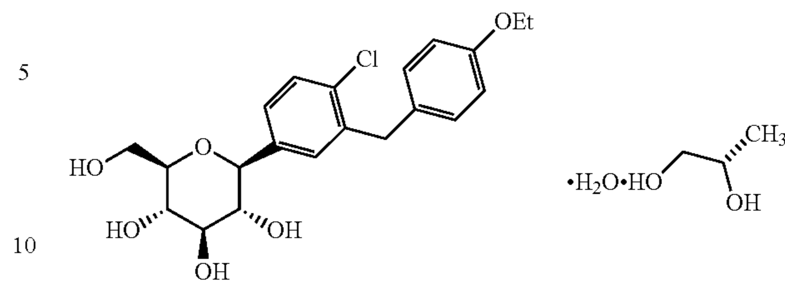
Compound Ia
