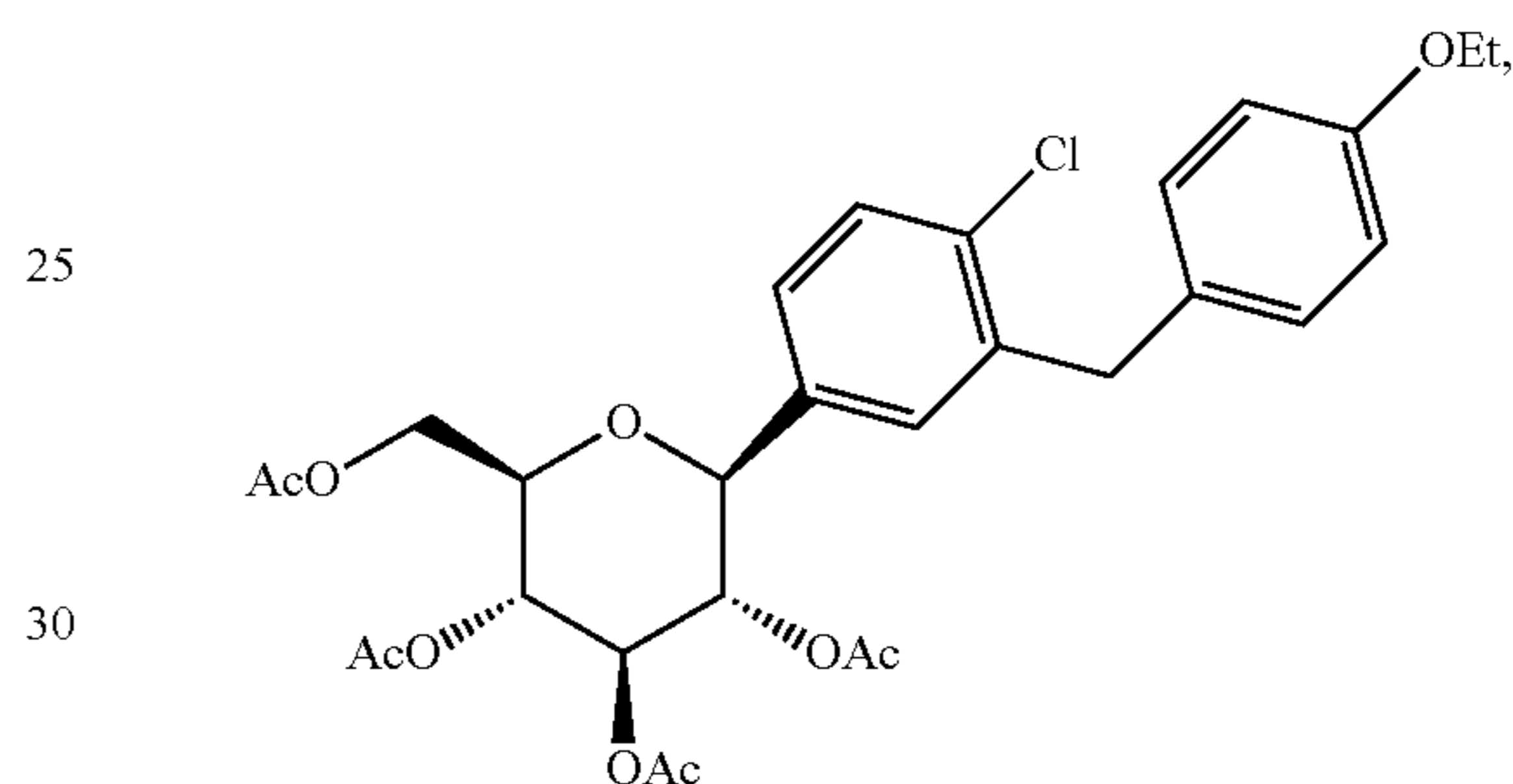
Compound A
