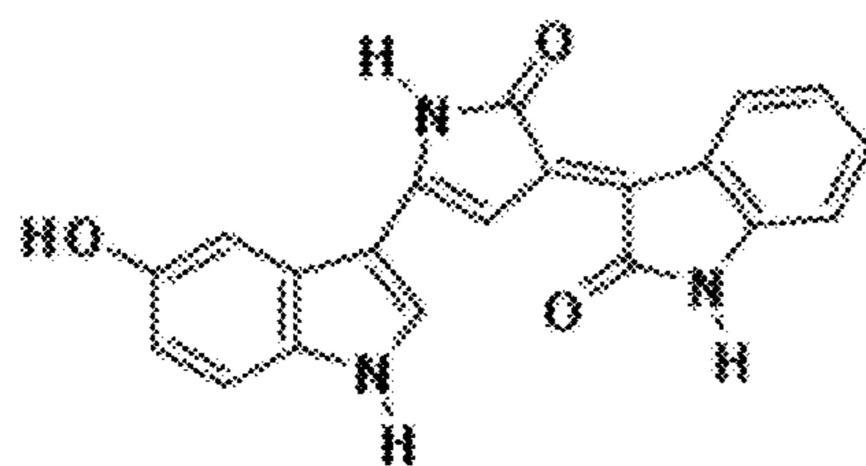
Violacein (2)
