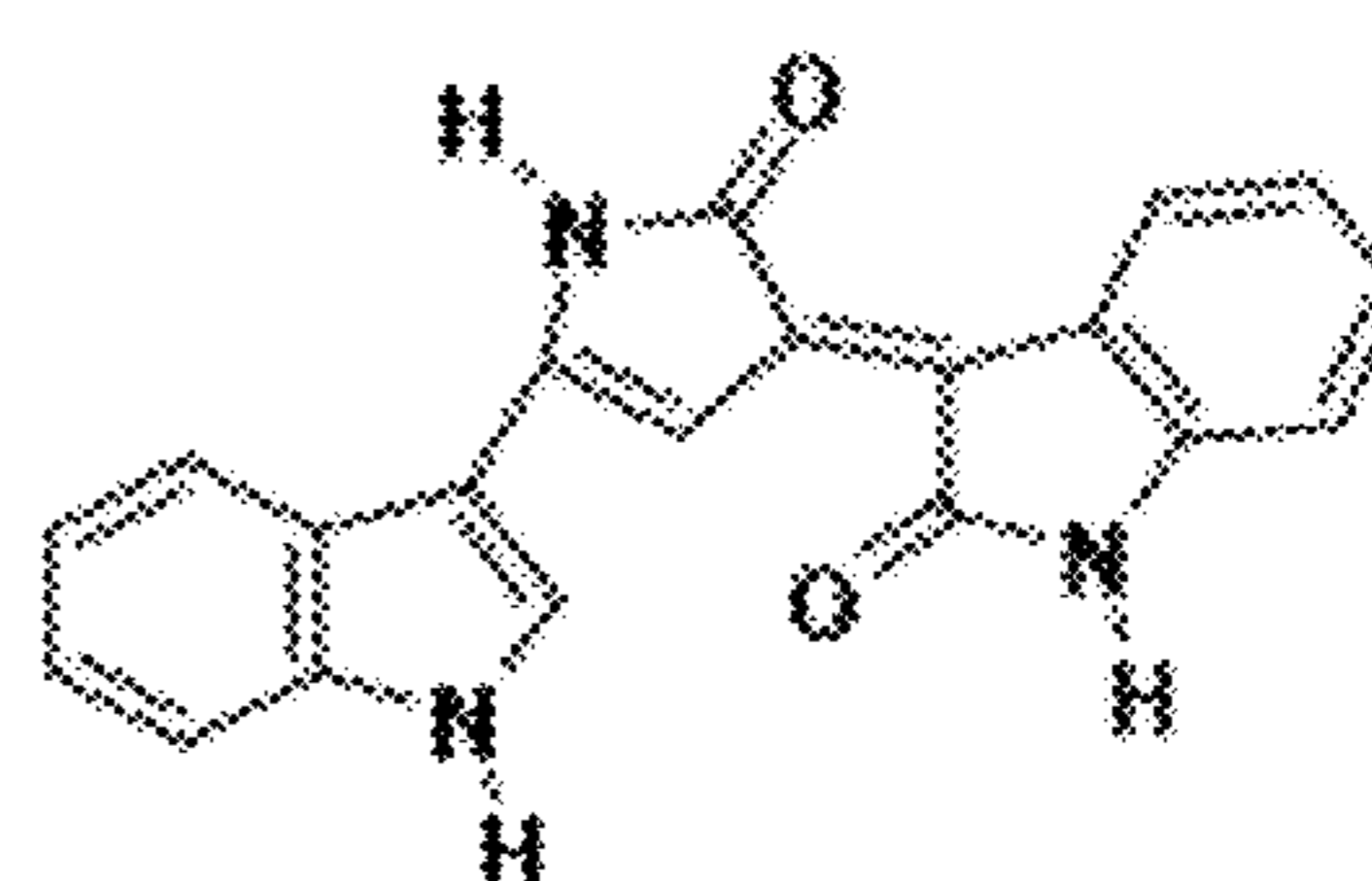
Deoxyviolacein (3)
