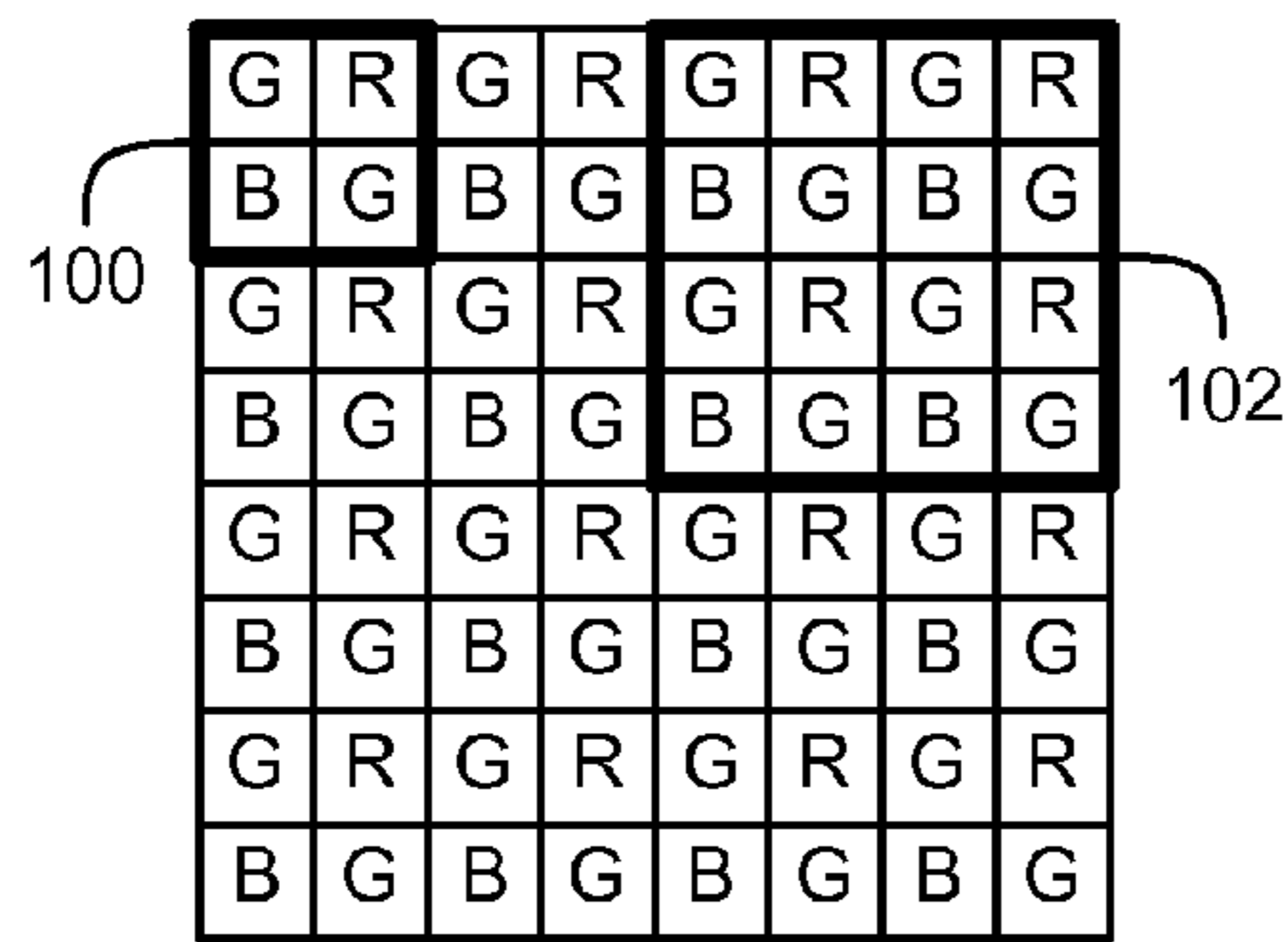
FIG. 2 (PRIOR ART)
