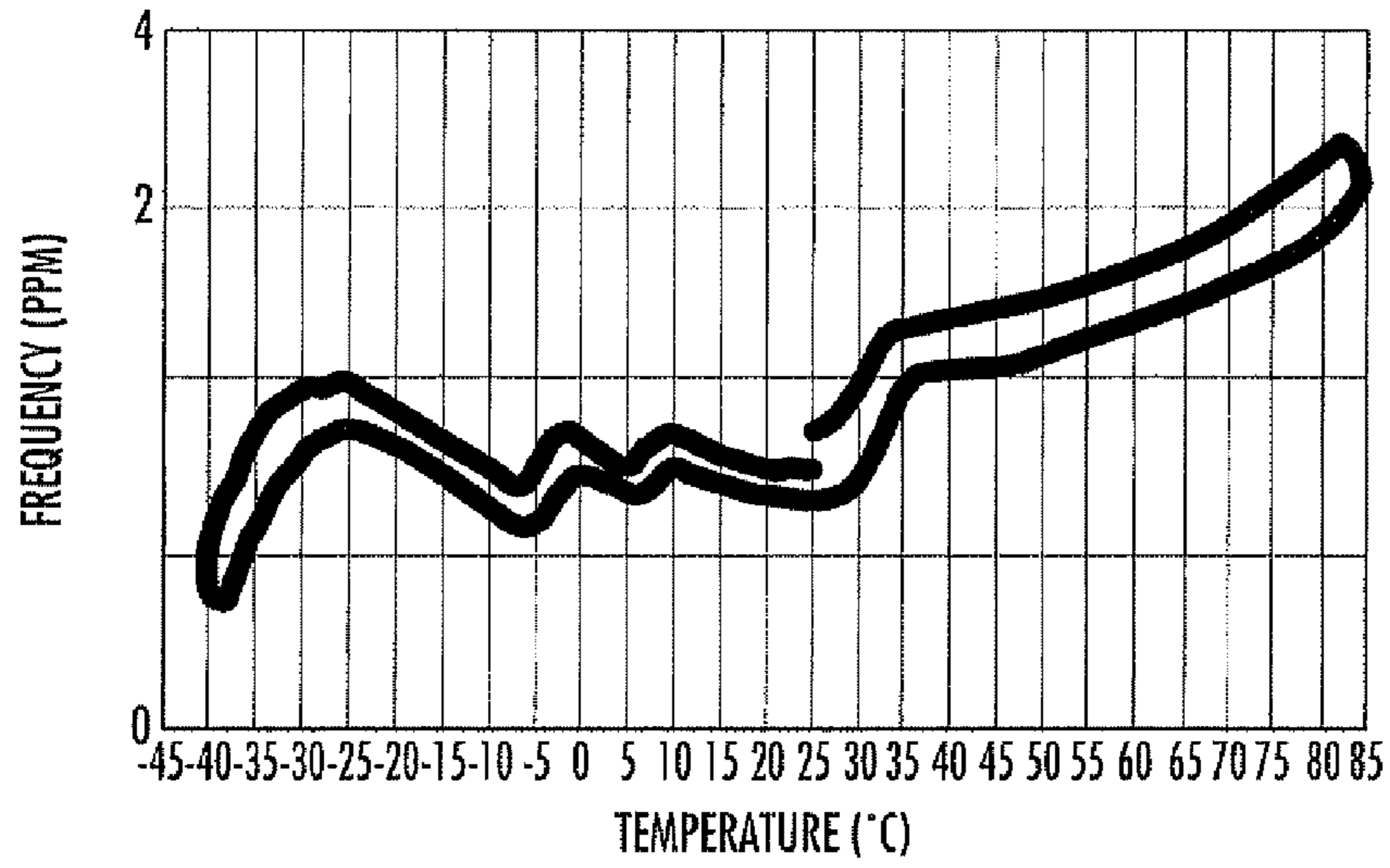
FIG. 11 (PRIOR ART)
