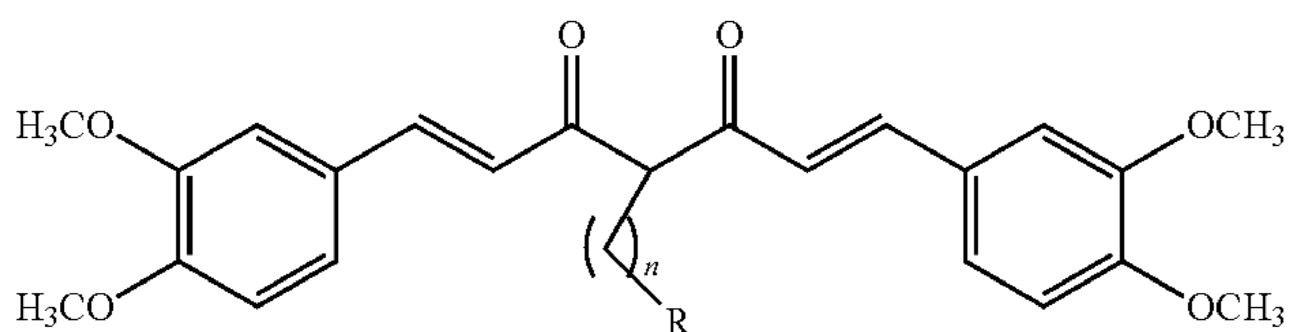
Compound Q44: n = 1, R = COOC 2 H 5
