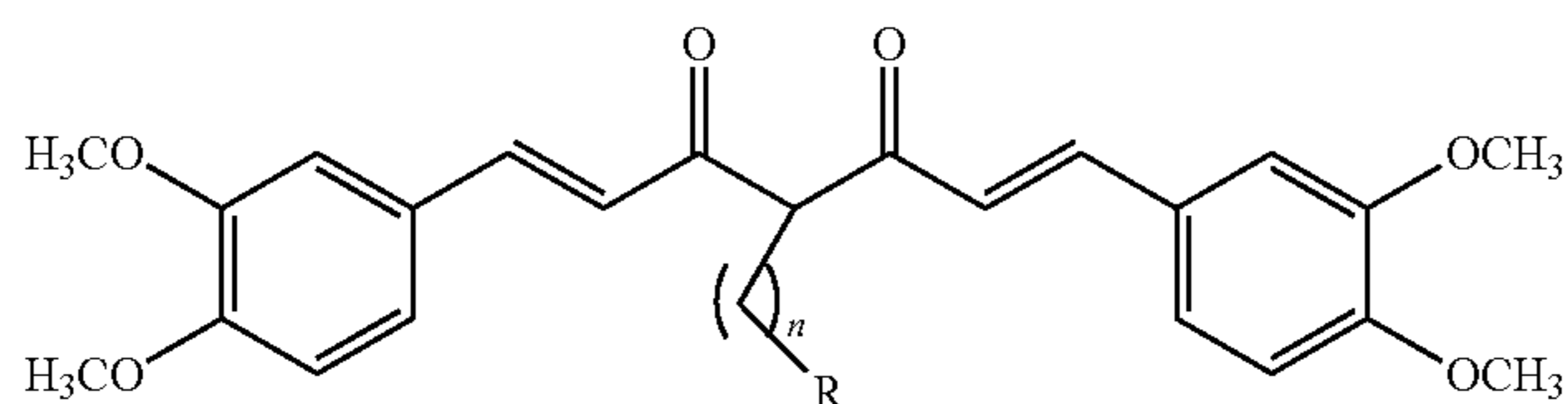
Compound Q49: n = 1, R = CON(C 2 H 5 ) 2
