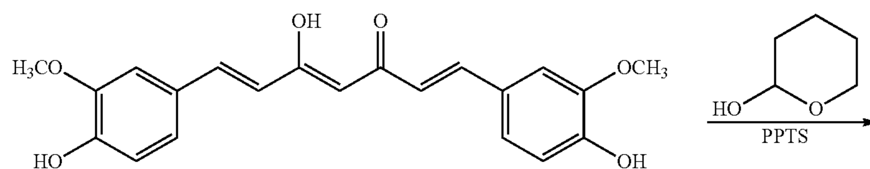
5-Hydroxy-1,7-bis(4-hydroxy-3-methoxyphenyl)hepta-1,4,6-trien-3-one
