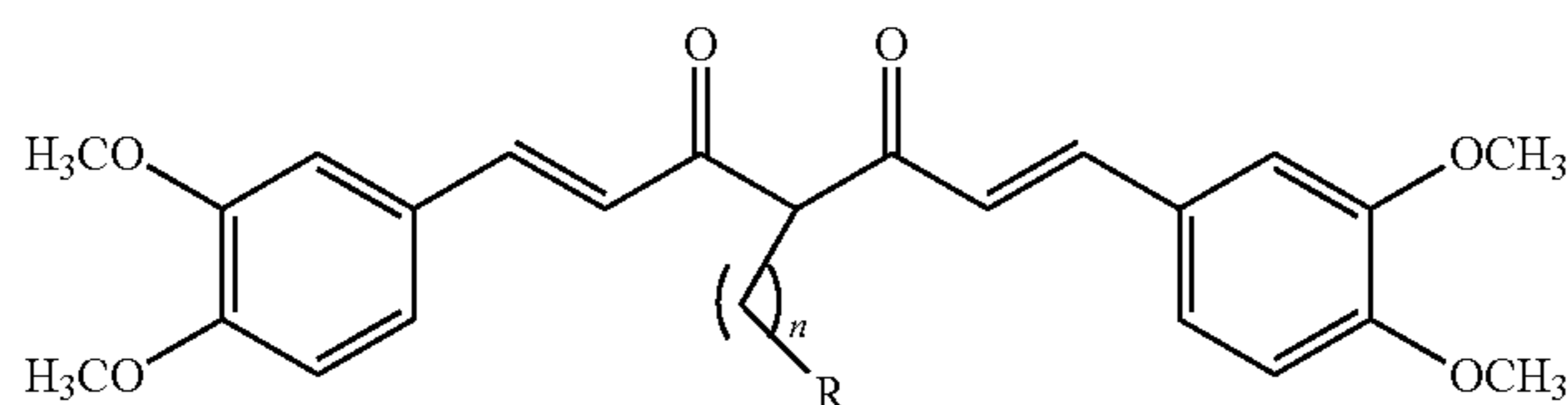
Compound Q49: n = 1, R = CON(C 2 H 5 ) 2 Compound Q77: n = 1, R = CON(CH 3 ) 2
