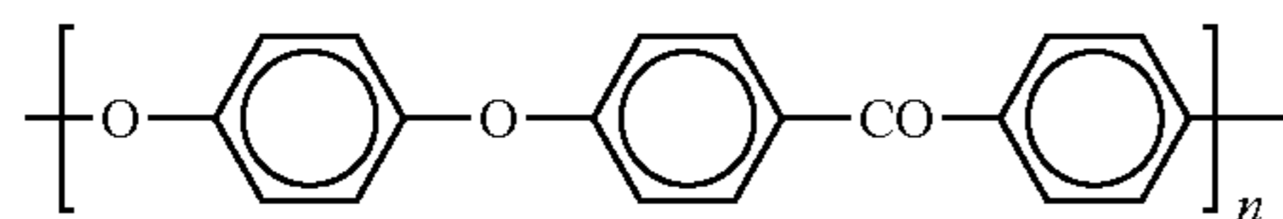
PEEK
