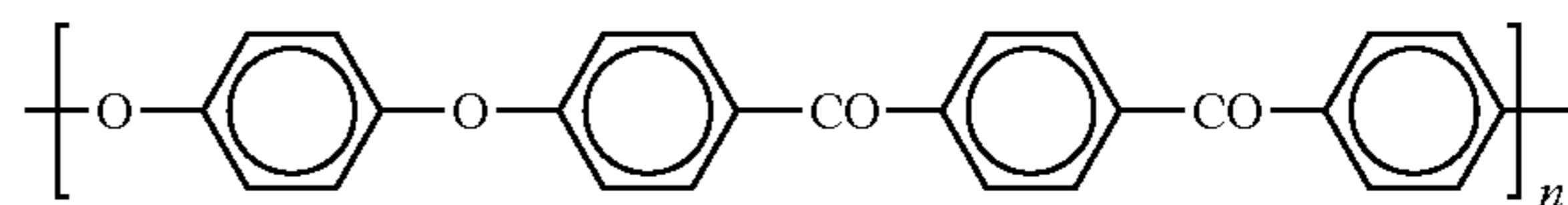
PEEKK
