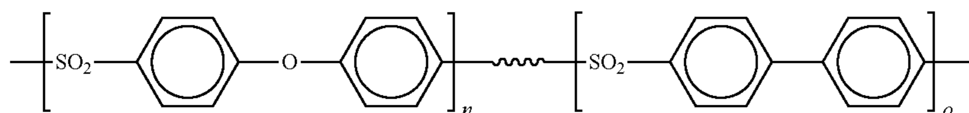
®Victrex 720 P
