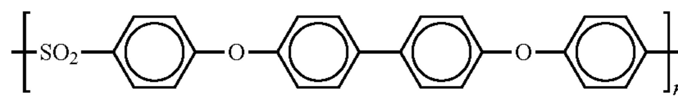
®Radel R
