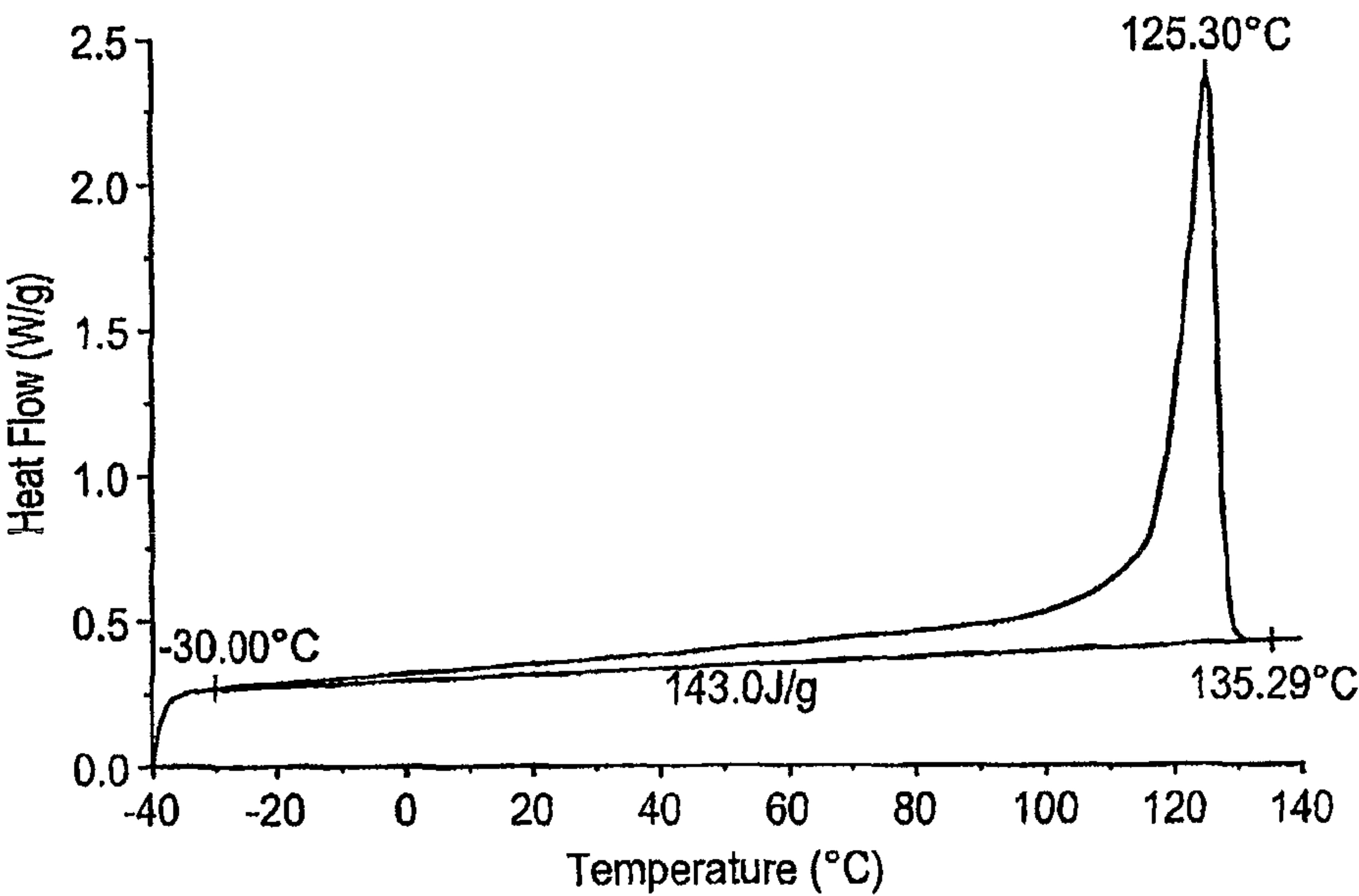
FIG. 24 DSC Comparative C*
