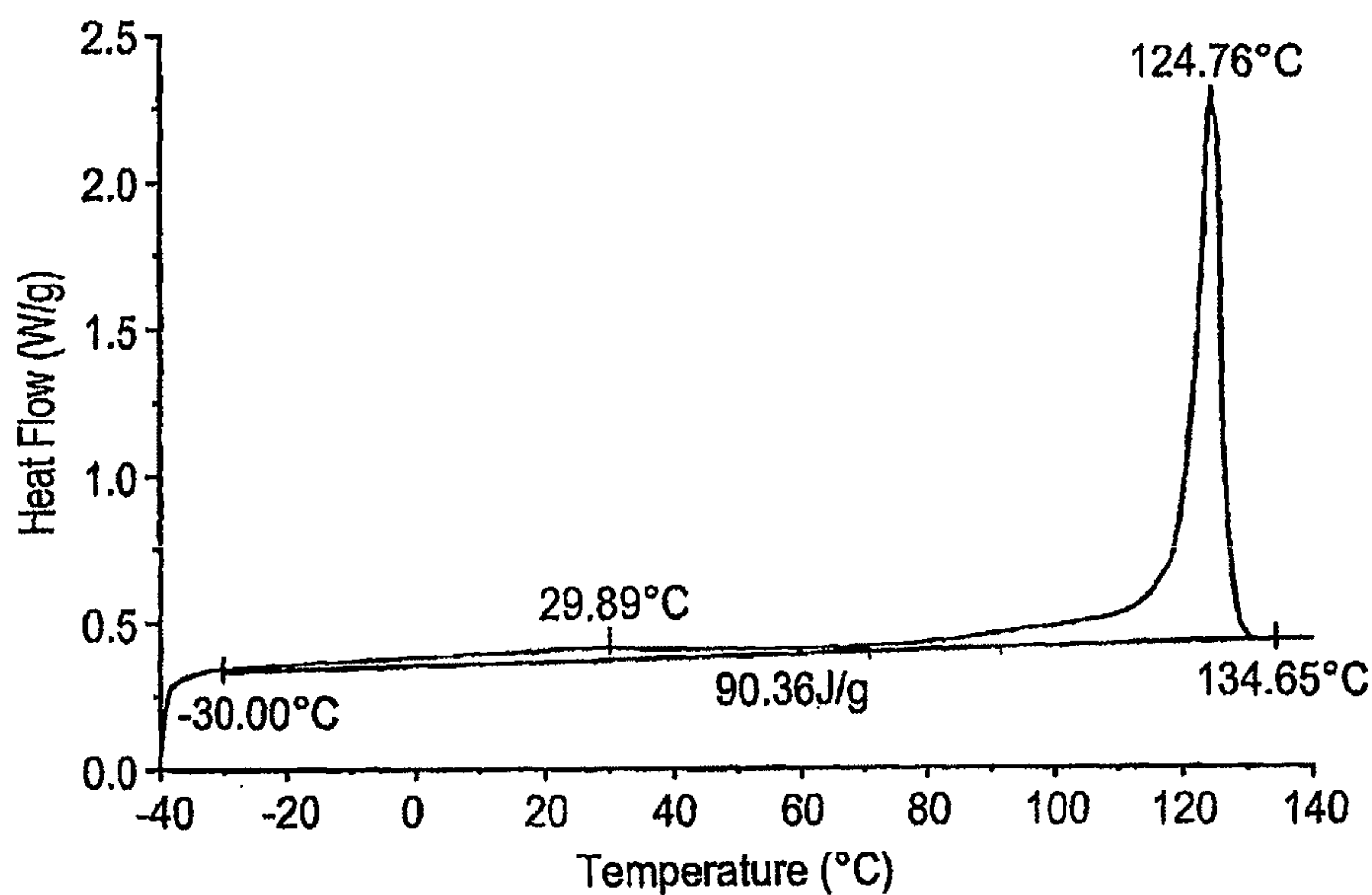
FIG. 27 DSC Comparative F*
