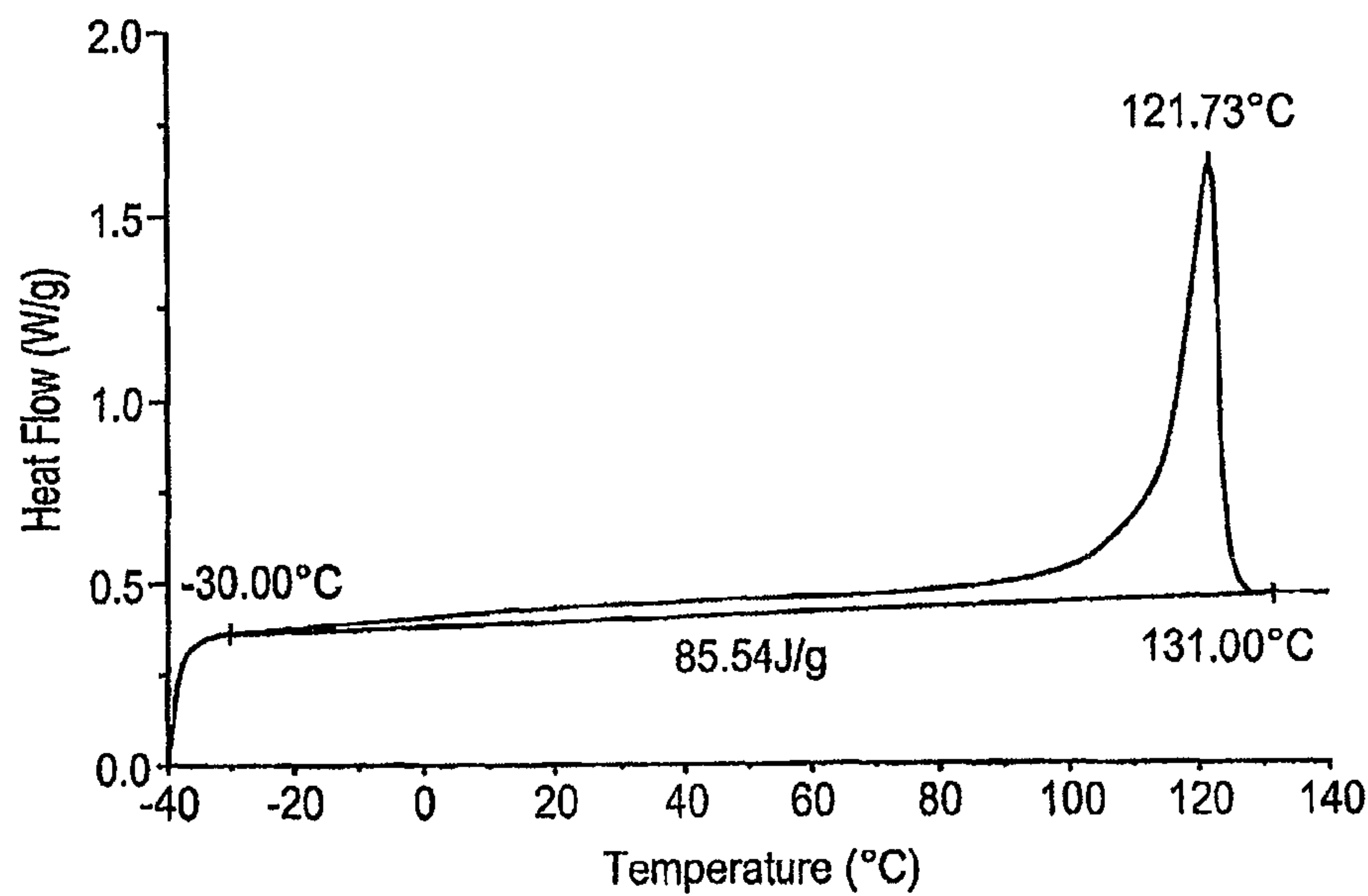
FIG. 47 DSC Comparative N*
