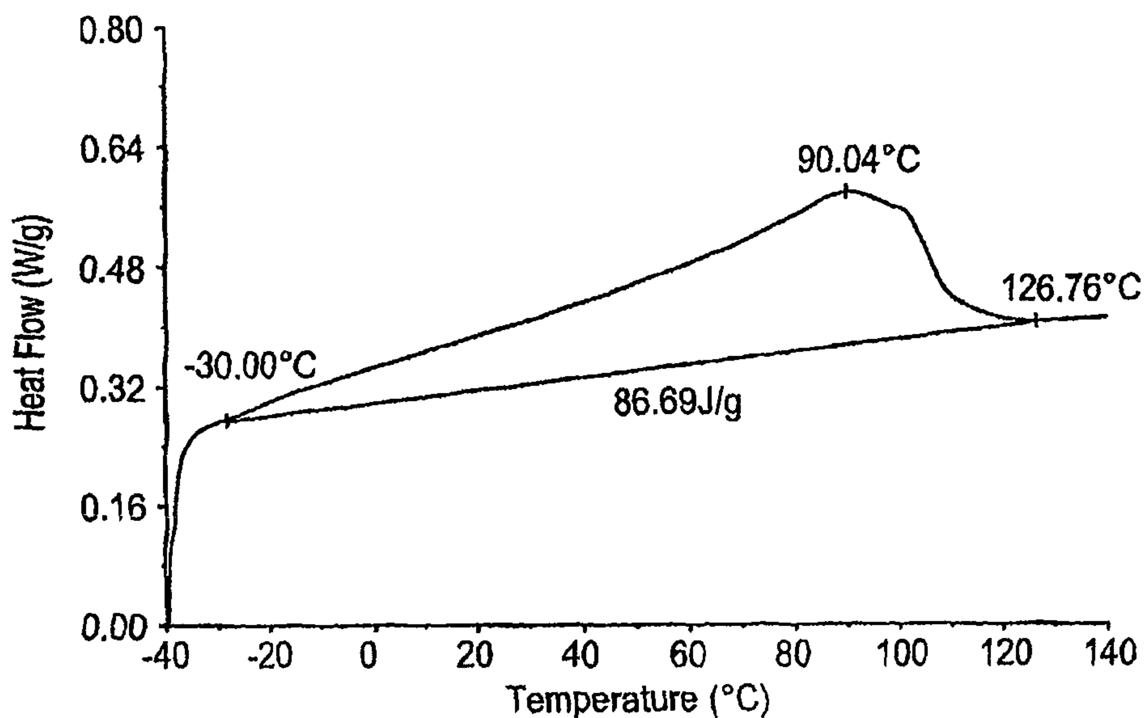
FIG. 22 DSC Comparative A*
