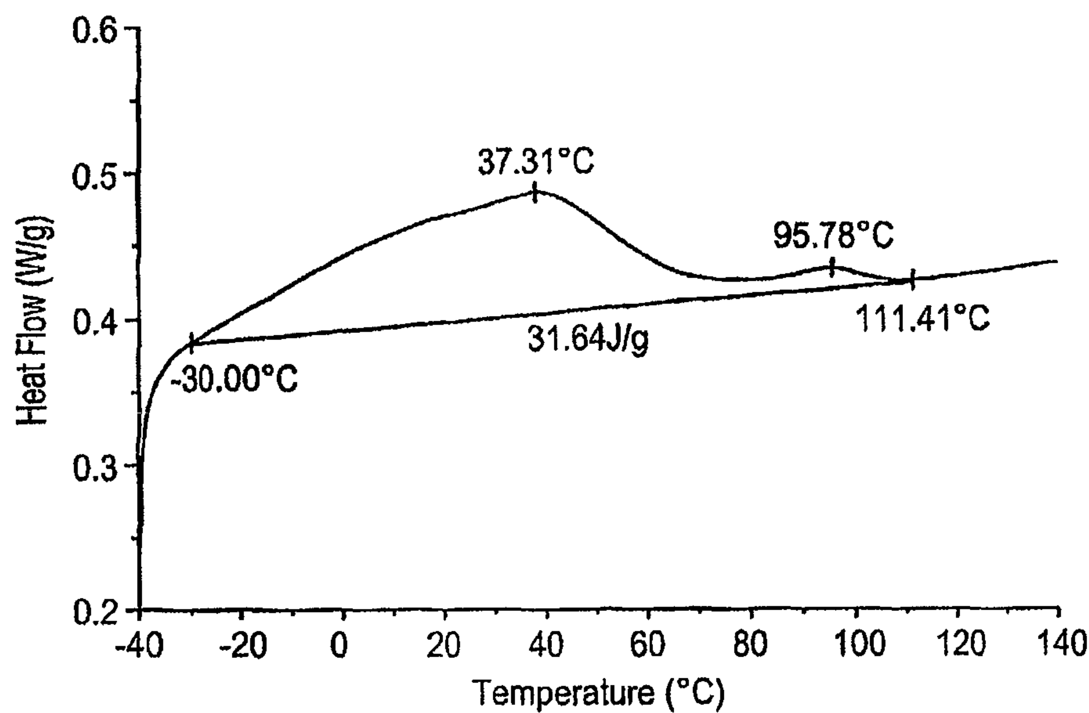
FIG. 25 DSC Comparative D*
