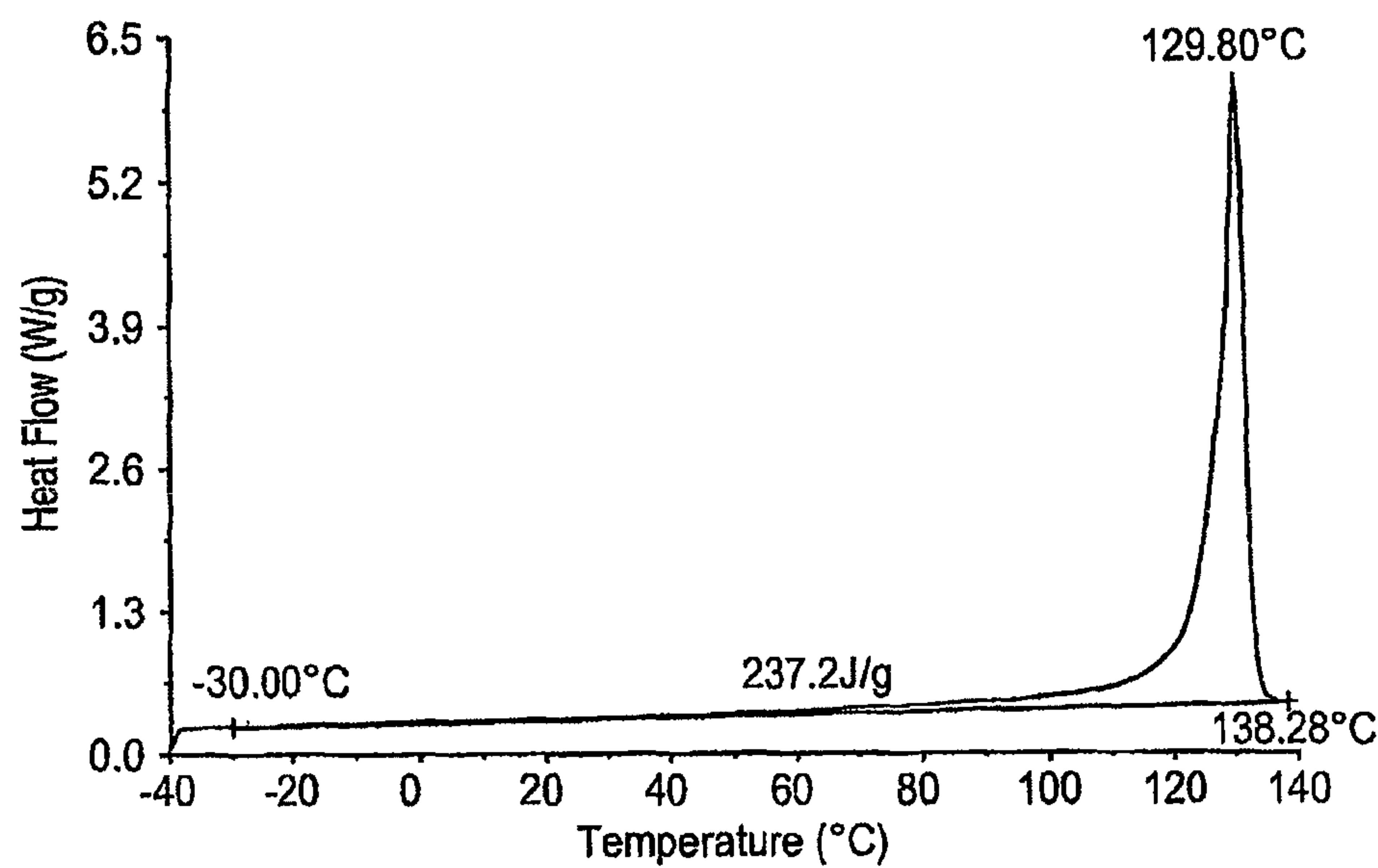
FIG. 23 DSC Comparative B*
