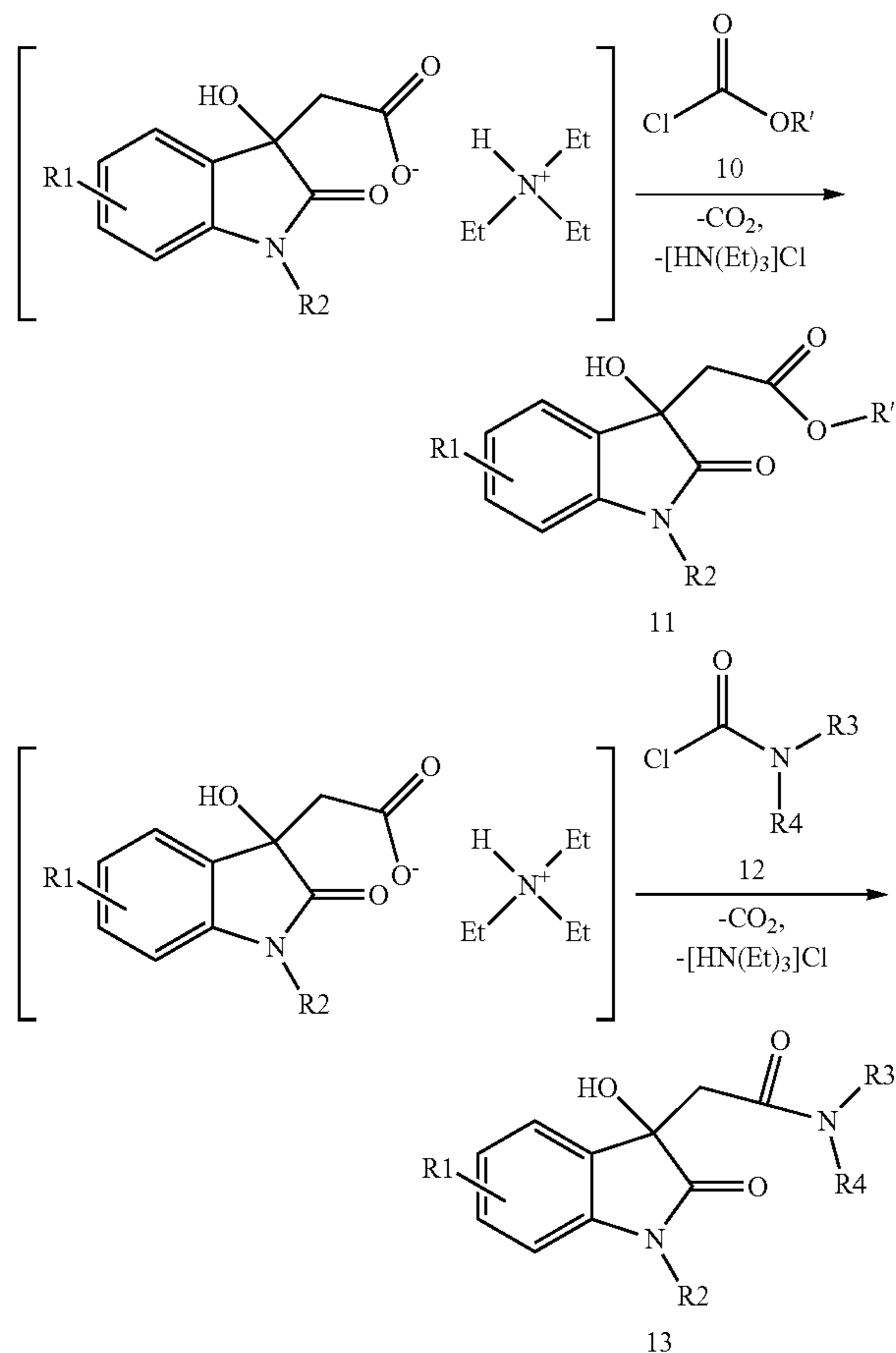
Scheme 7: Synthesis of esters 11 and amides 13 of 9
