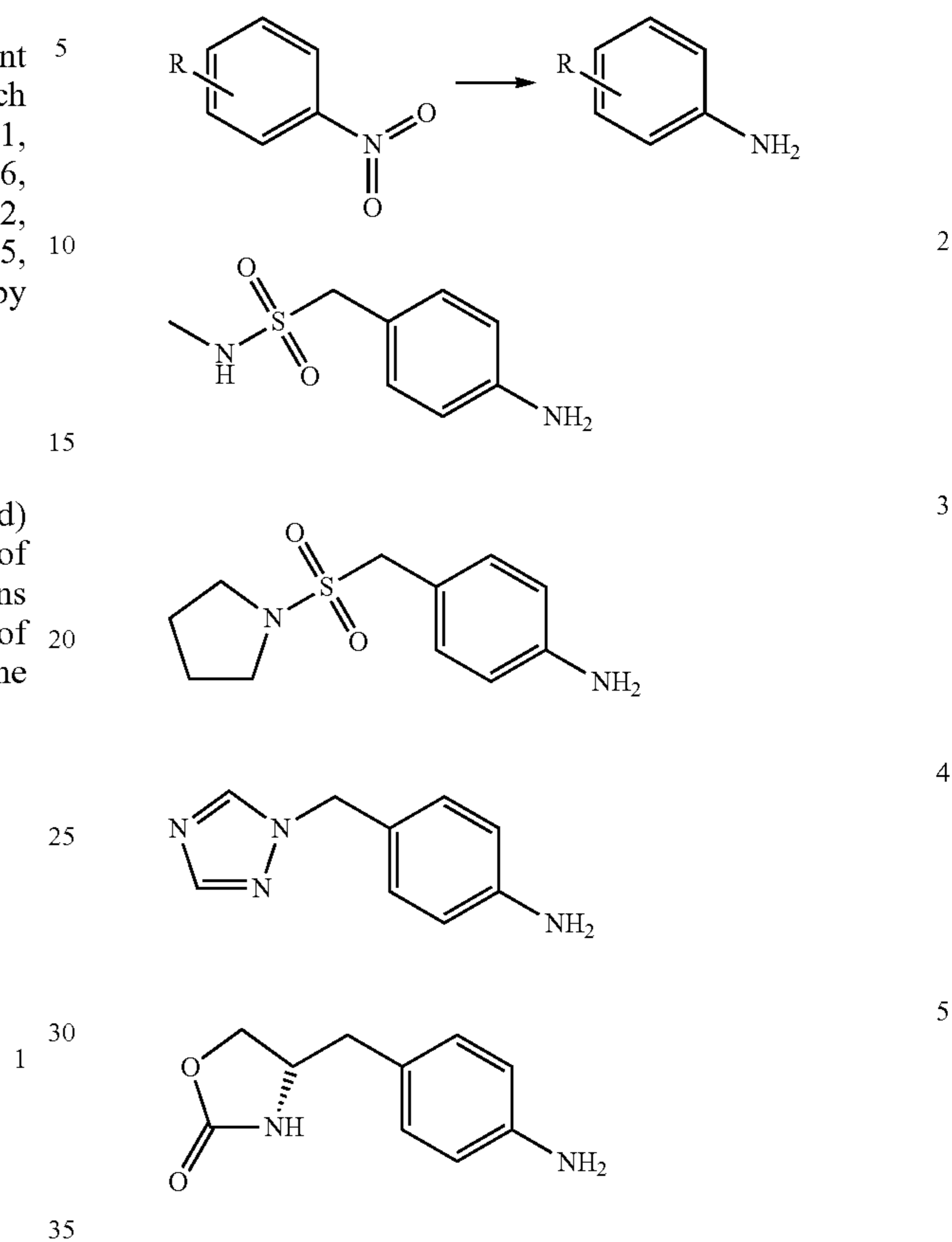
Scheme 1 Synthesis of aniline precursors for tryptamine derivatives (R = the para-substituents of the aniline moiety in 3, 4, 5 or 6)
