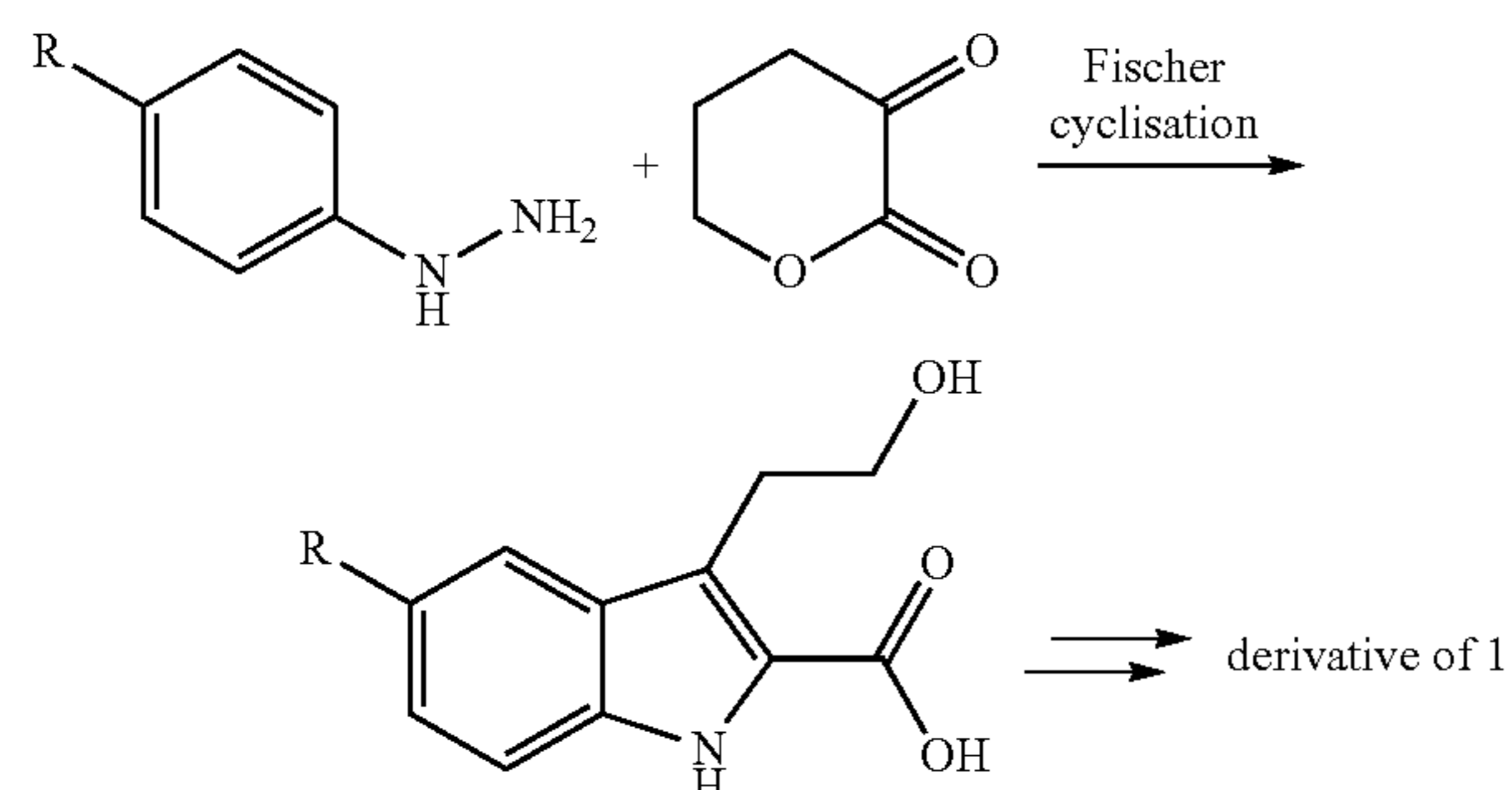
Scheme 3: Alternative Carbonyl compounds for the Fischer cyclisation
