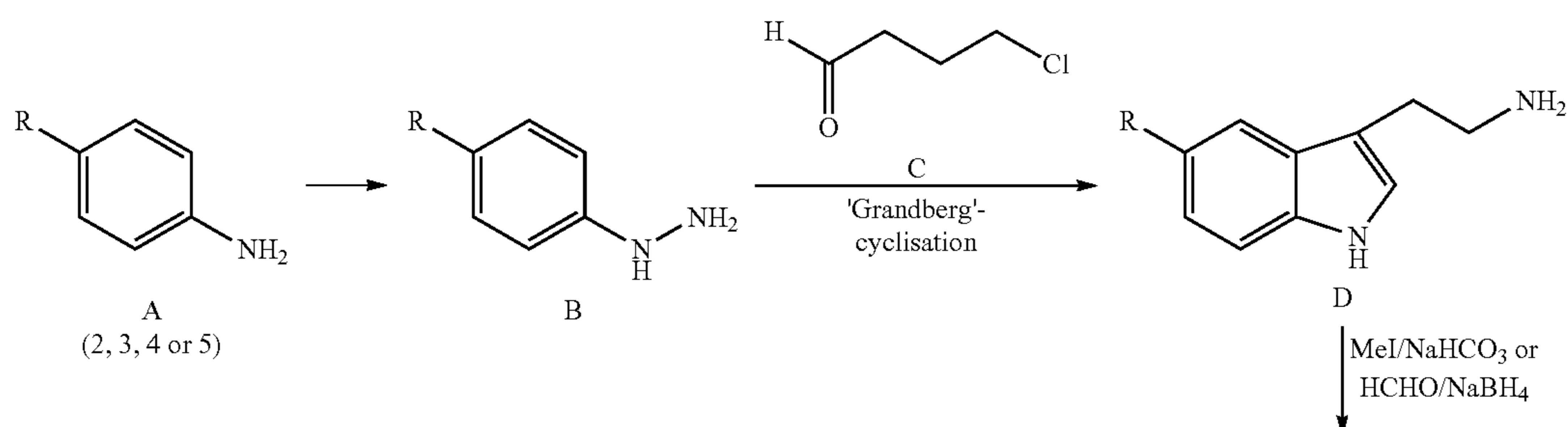
Scheme 2. Synthesis of tryptanes from their aniline precursors
