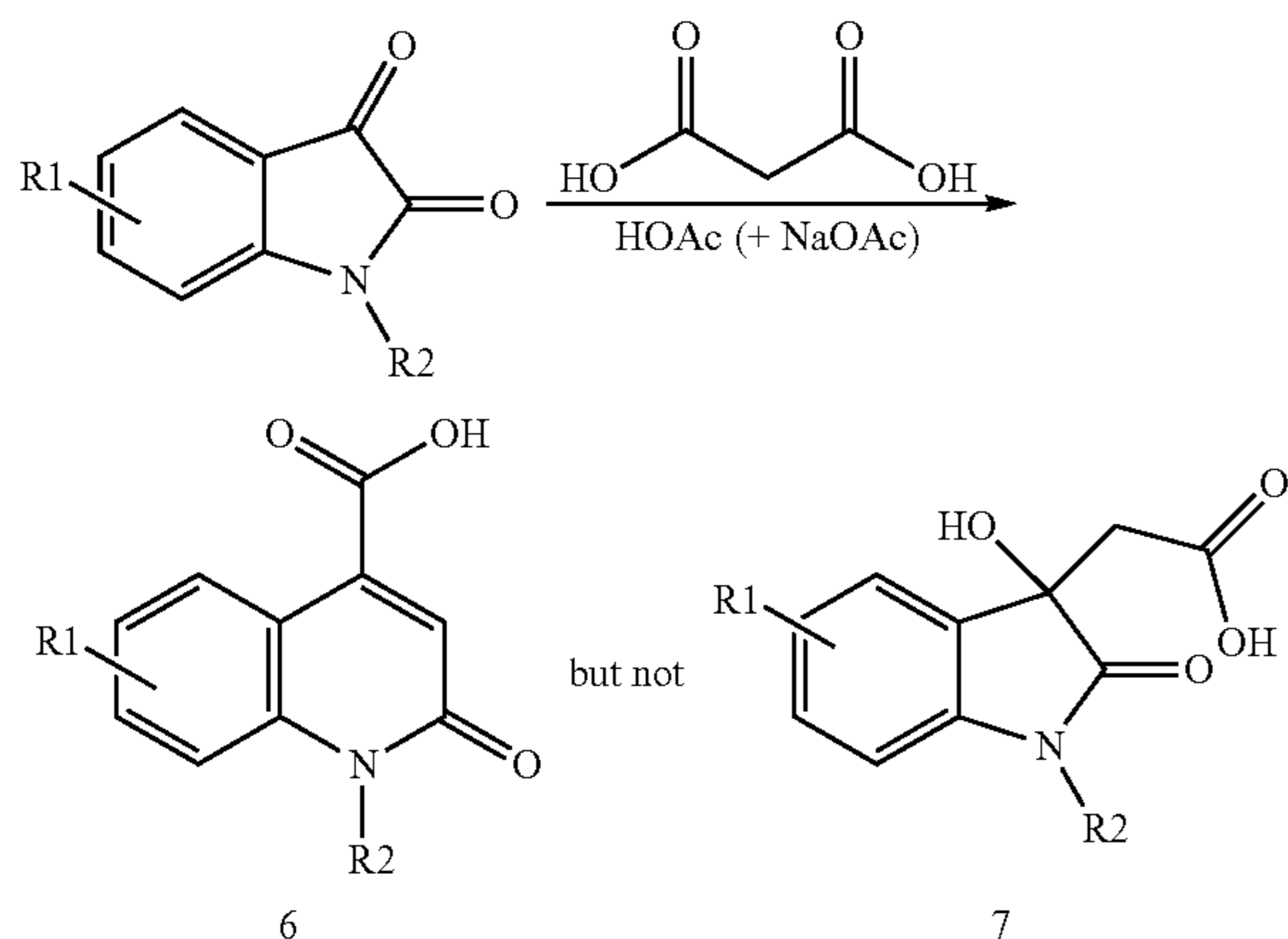
Scheme 5: Condensation of isatin with malonic acid in acetic acid
