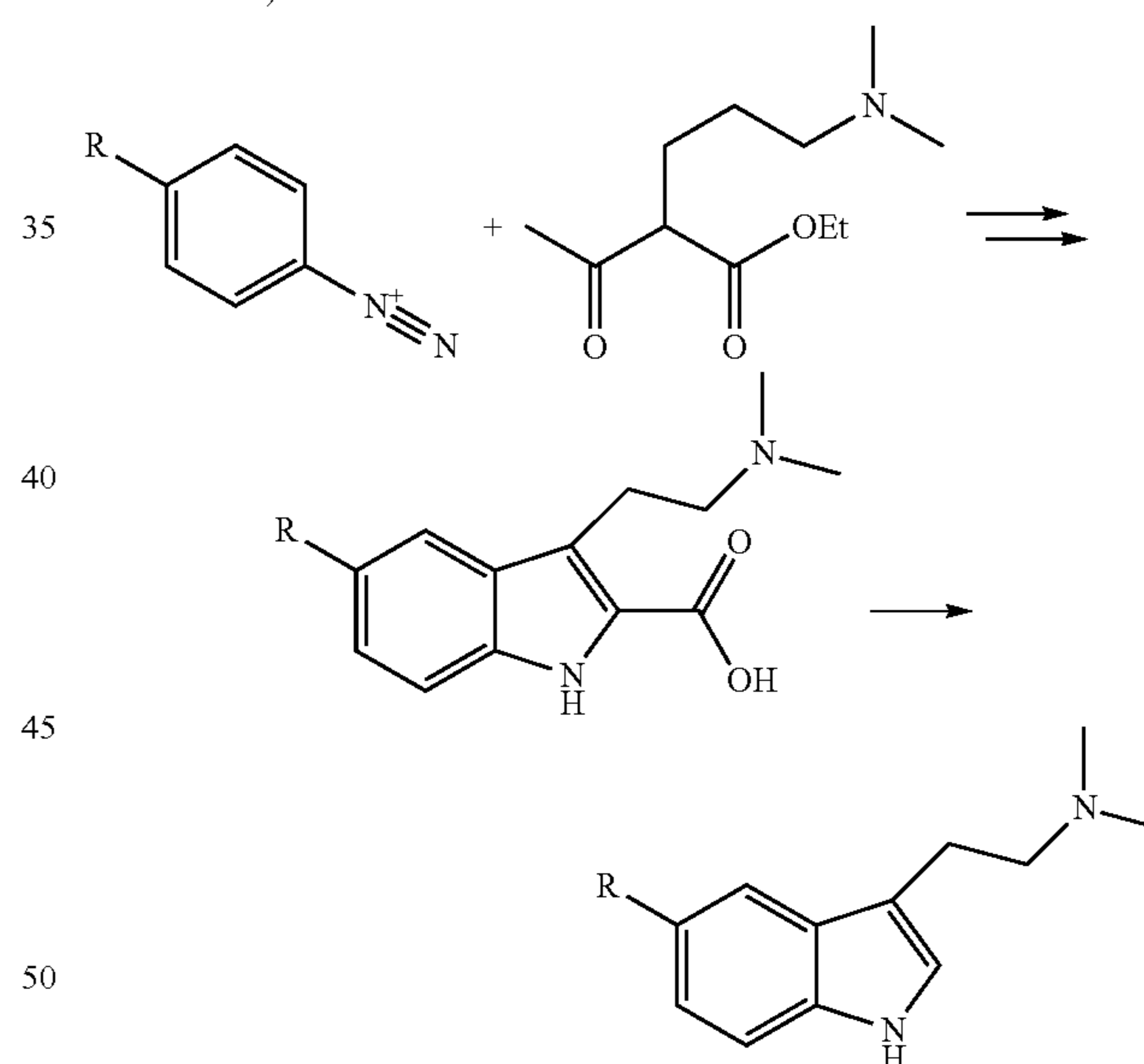
Scheme 4: Alternative to the preparation of a phenyl hydrazine (synthesis of the N,N-dimethylpropyl-malonic acid ethyl ester is inconvenient)
