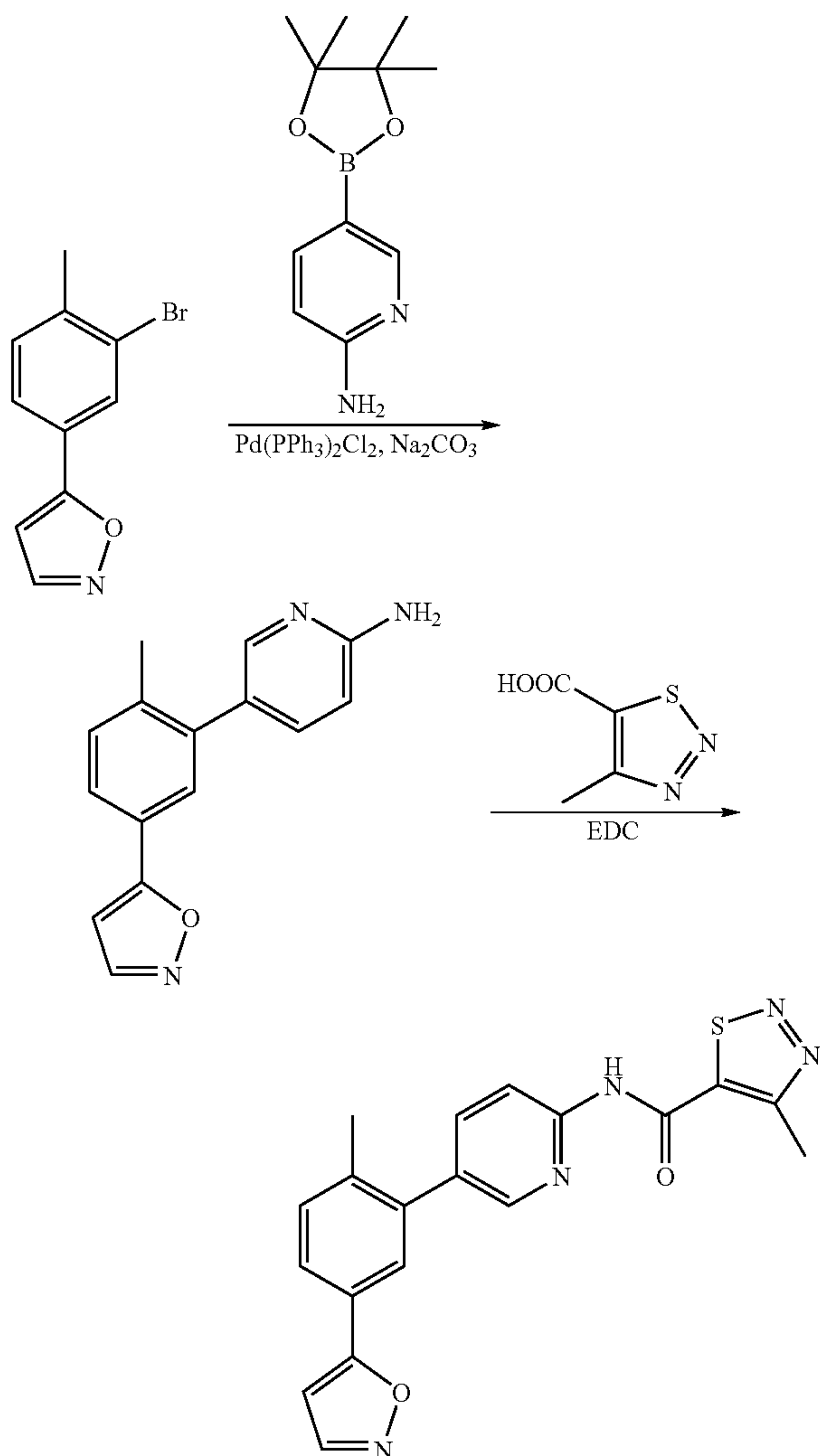
Compound 68
