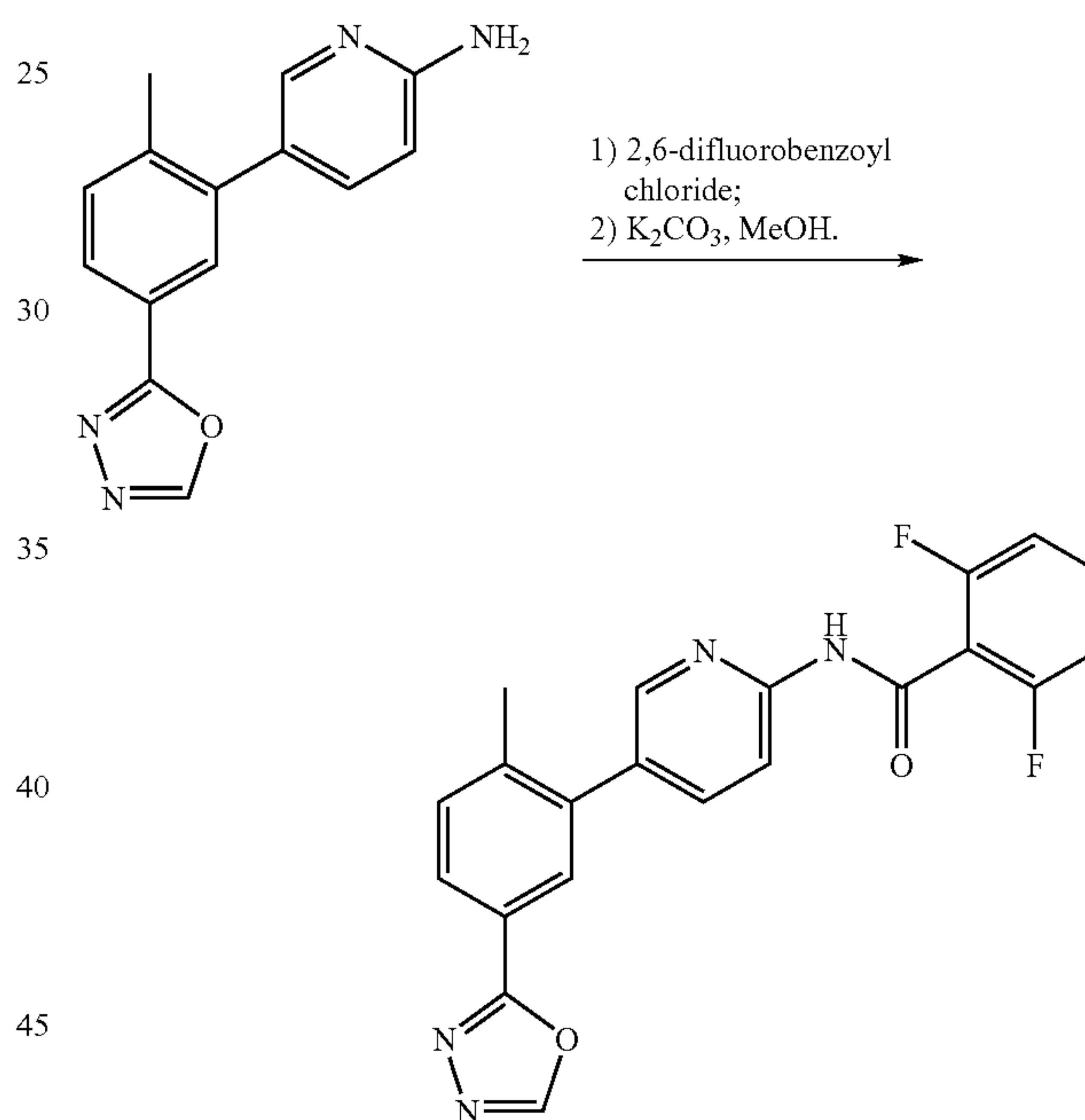
Compound 69
