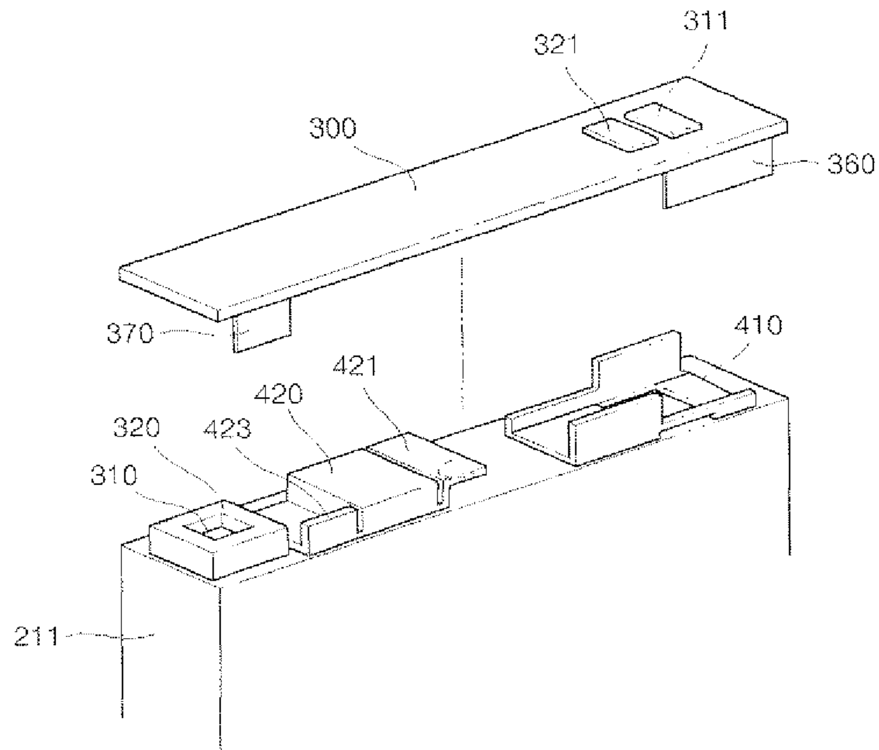
FIG. 2 PRIOR ART
