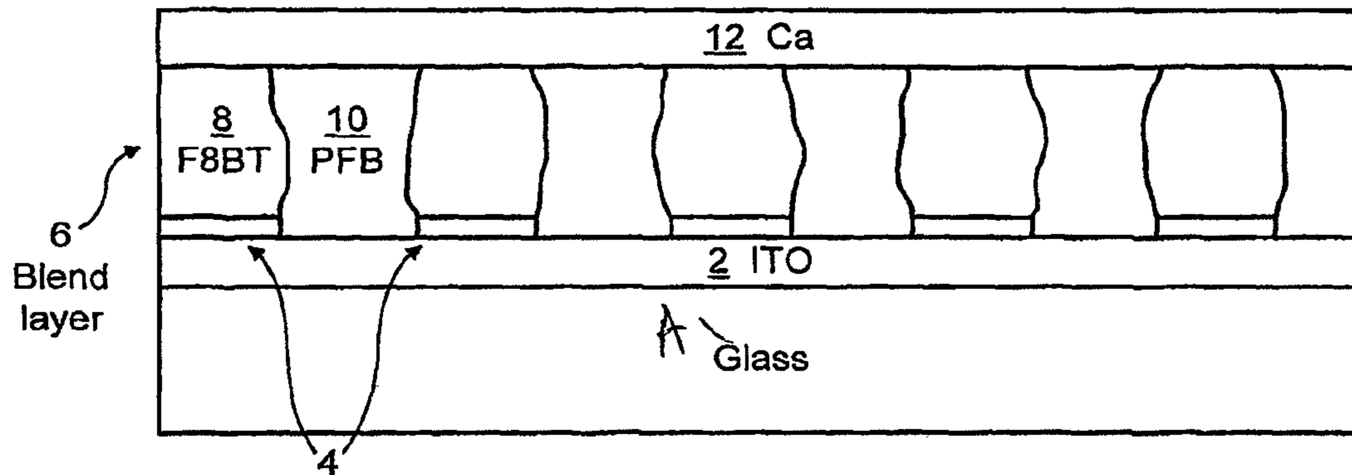
Au strips in cross section
