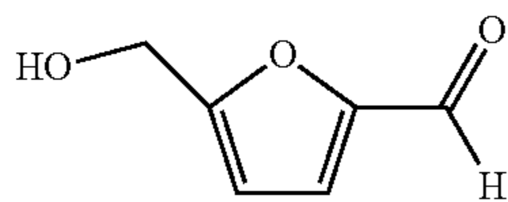
hydroxymethylfurfural
