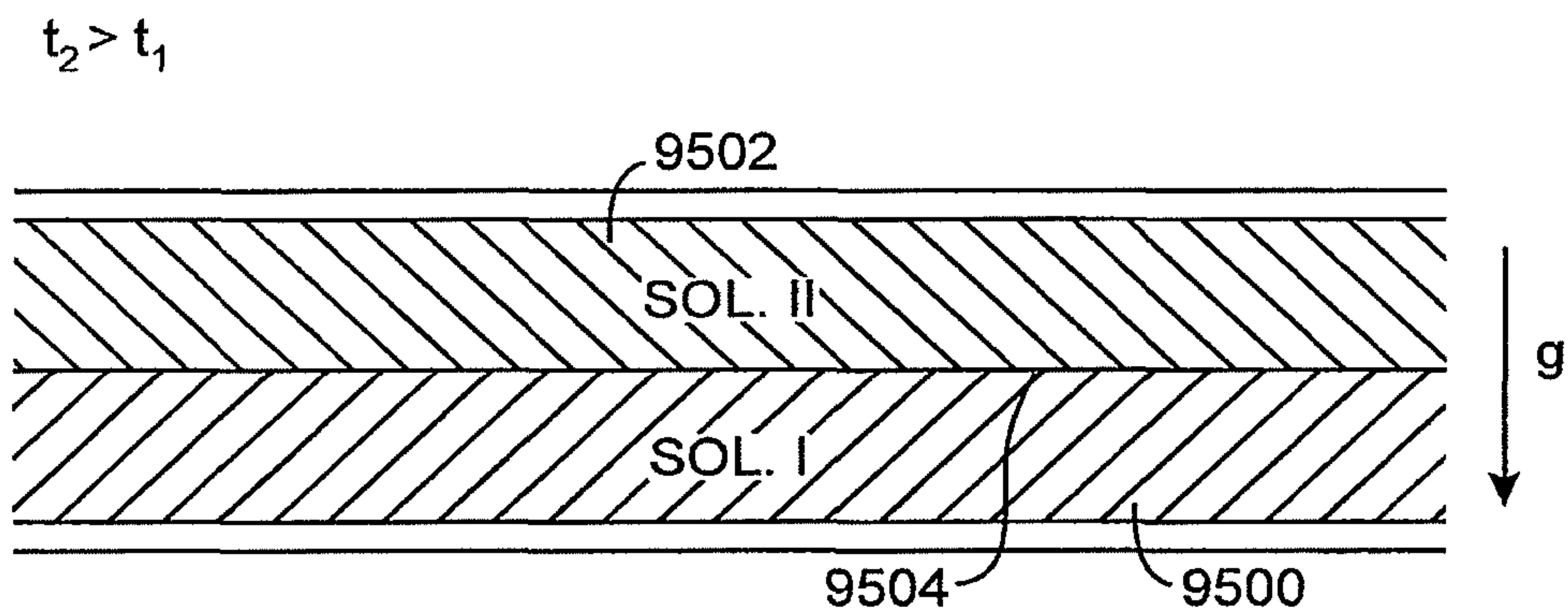
FIG. 32C (Prior Art)
