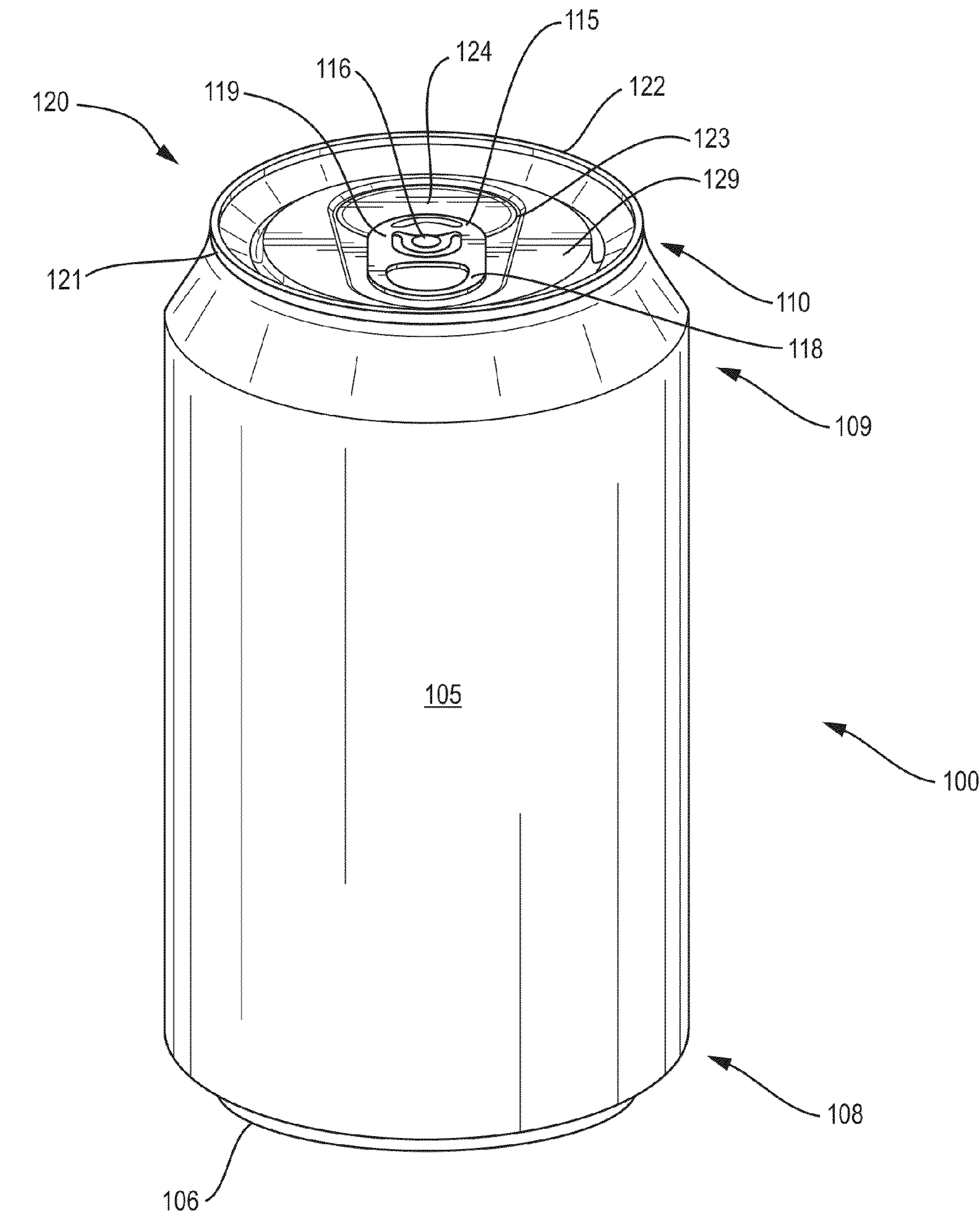
FIG. 1 (PRIOR ART)
