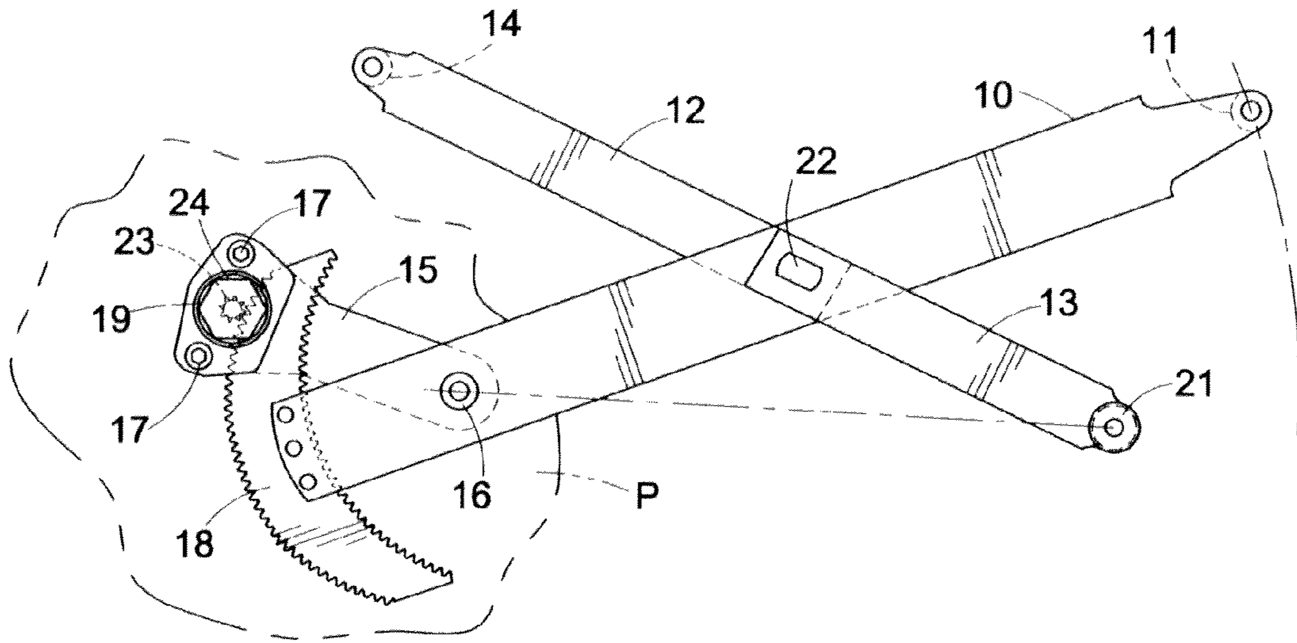
FIG. 1 (PRIOR ART)
