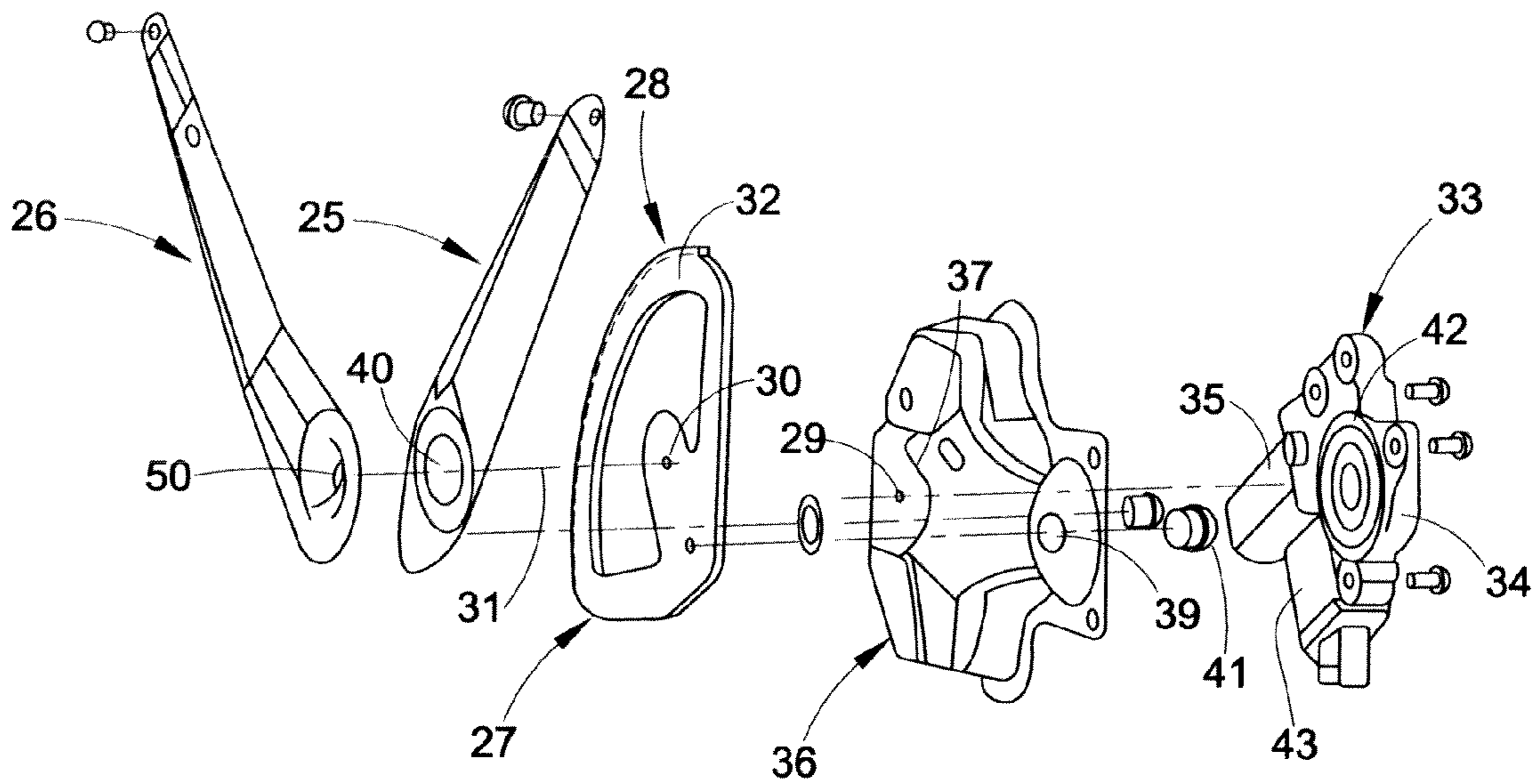
FIG. 2 (PRIOR ART)
