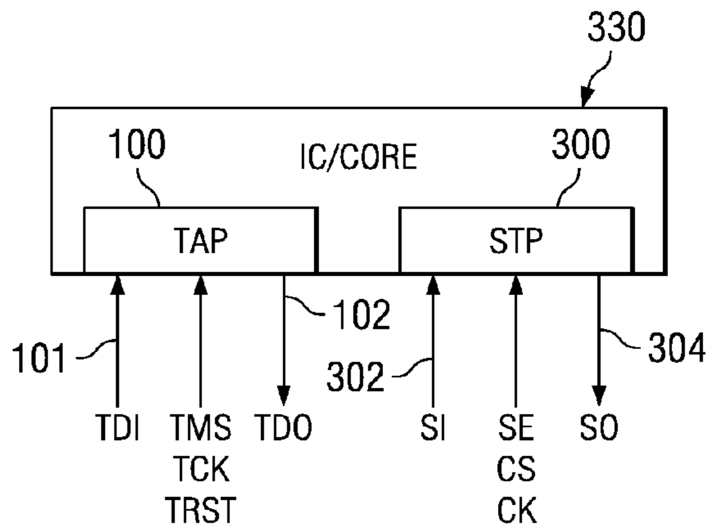
FIG. 3C (PRIOR ART)
