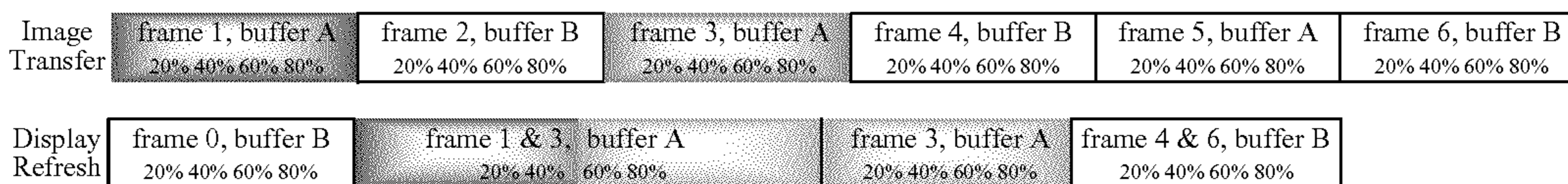
Two Buffers, display refresh slower than image transfer
