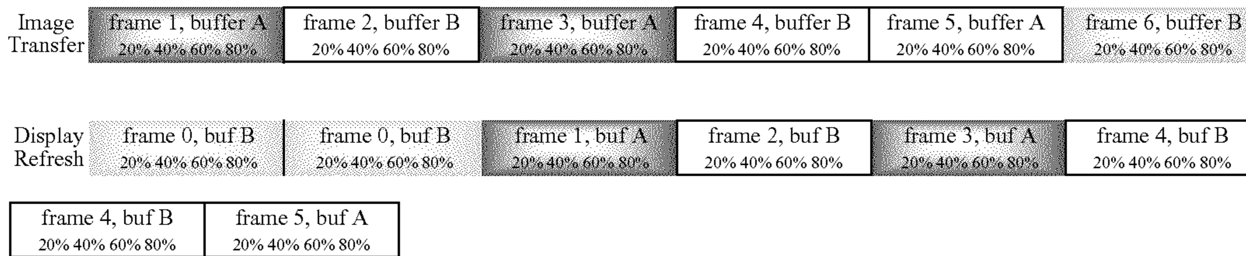
Two Buffers, display refresh much faster than image transfer
