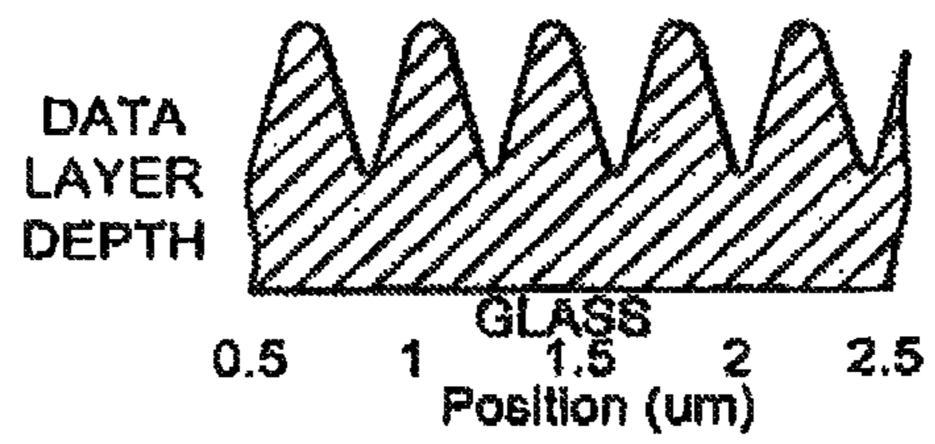
FIG. 2 PRIOR ART
