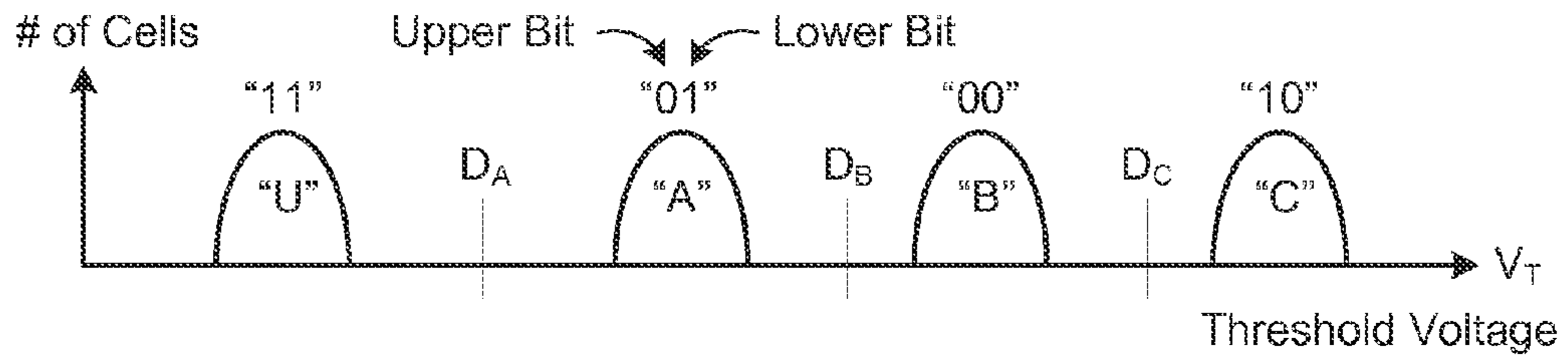
Multistate Memory (LM Gray Code)
