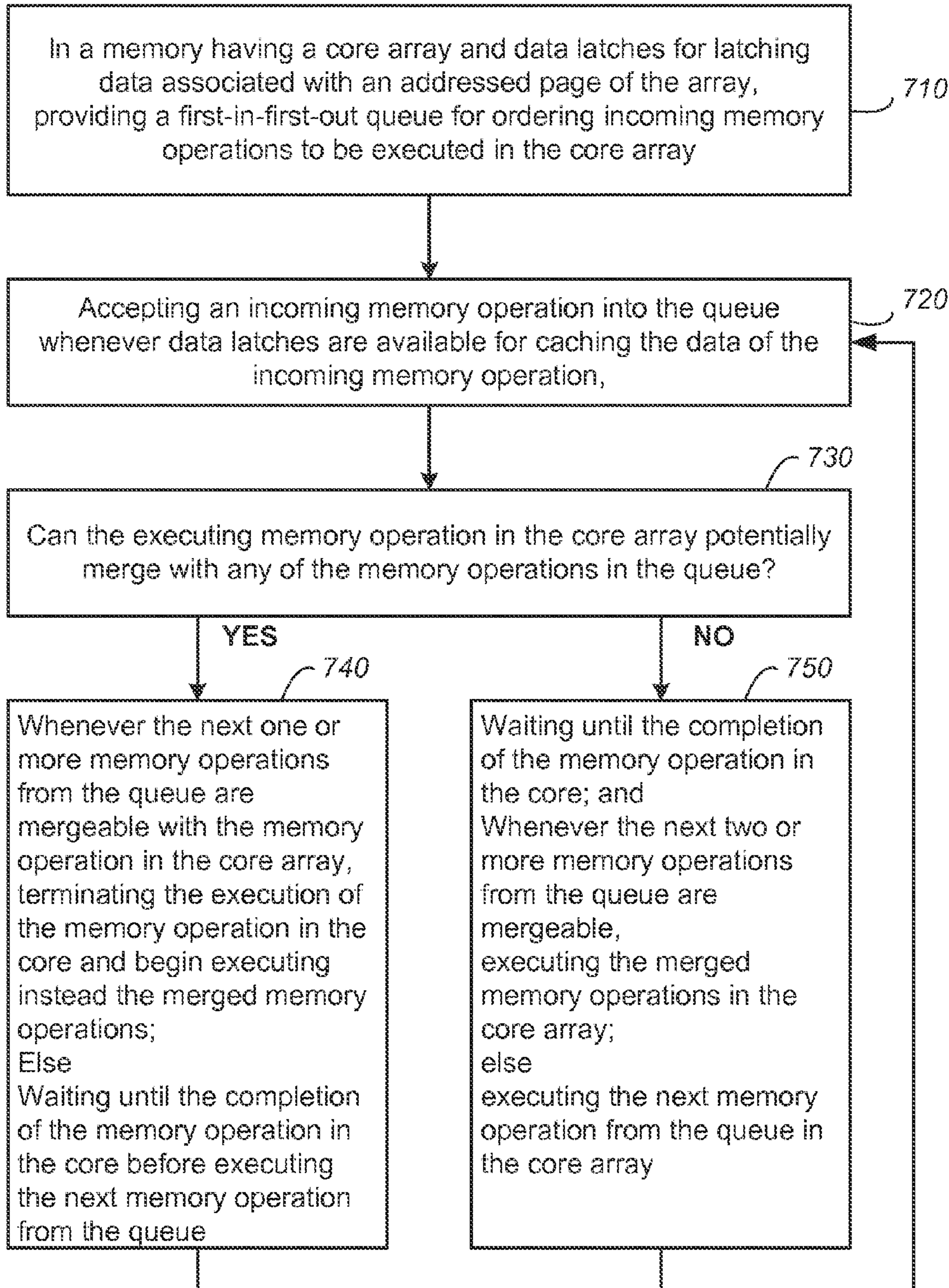
MULTIPLE MEMORY OPERATIONS MANAGEMENT
