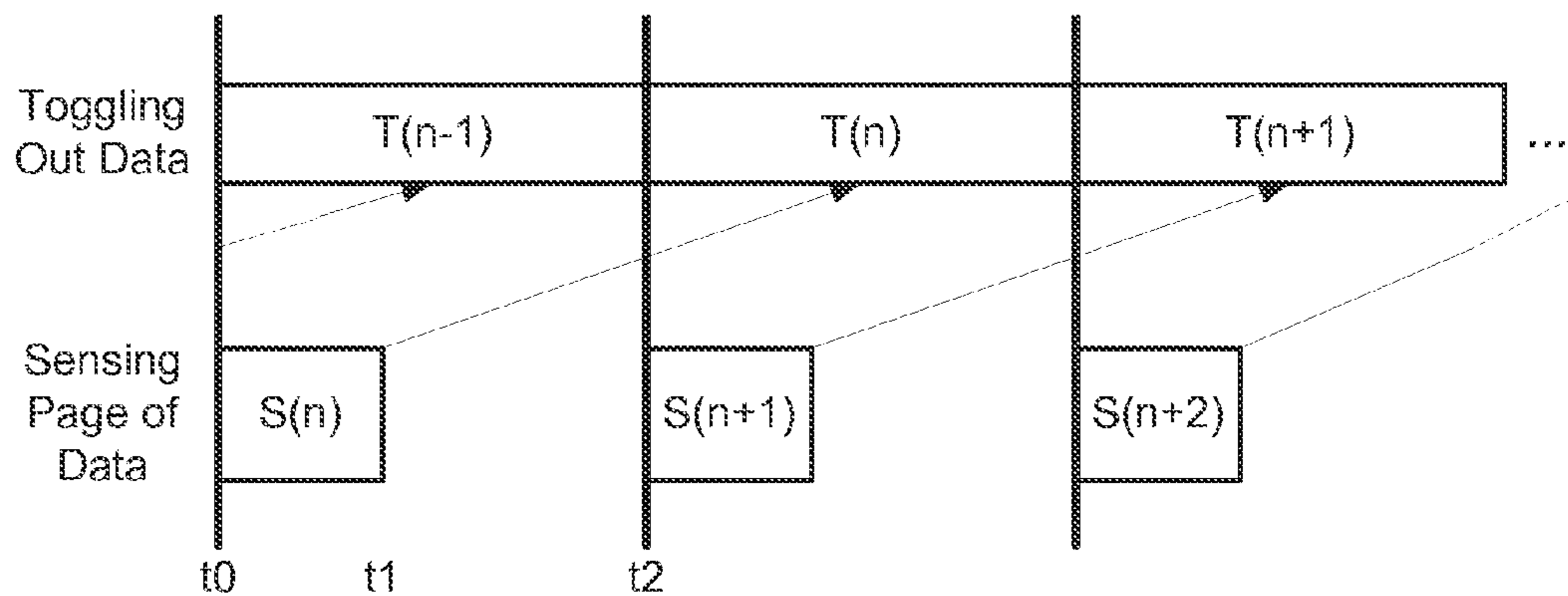
Conventional Read Caching
