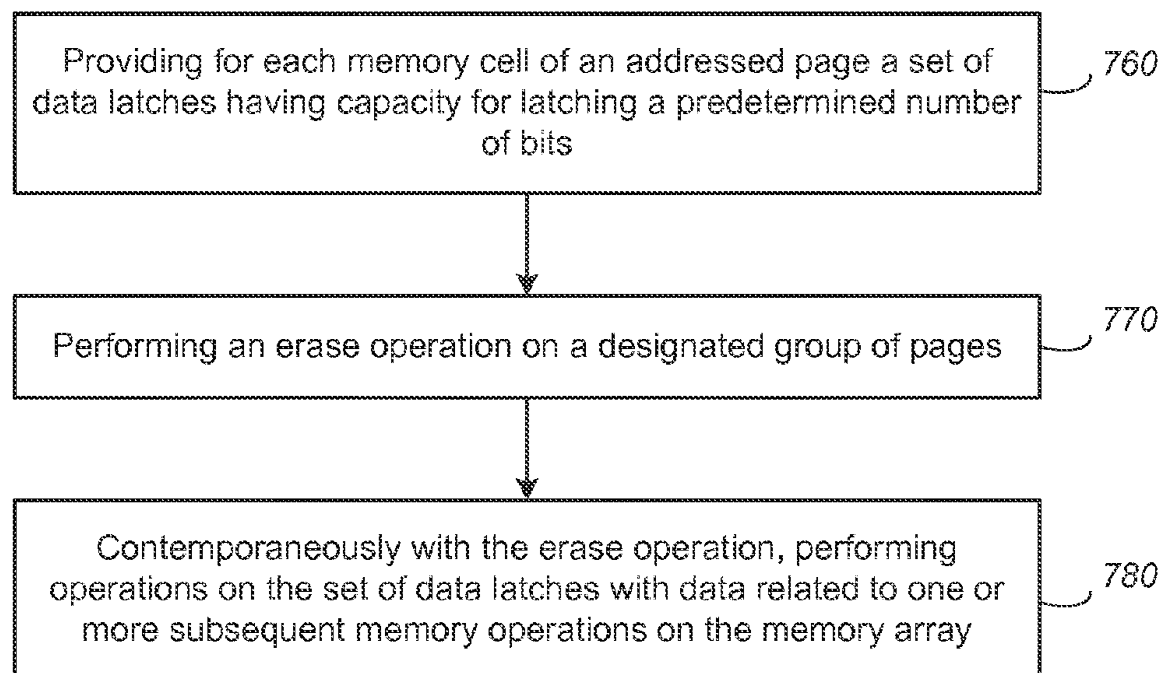
Cache Operation During Erase Operation
