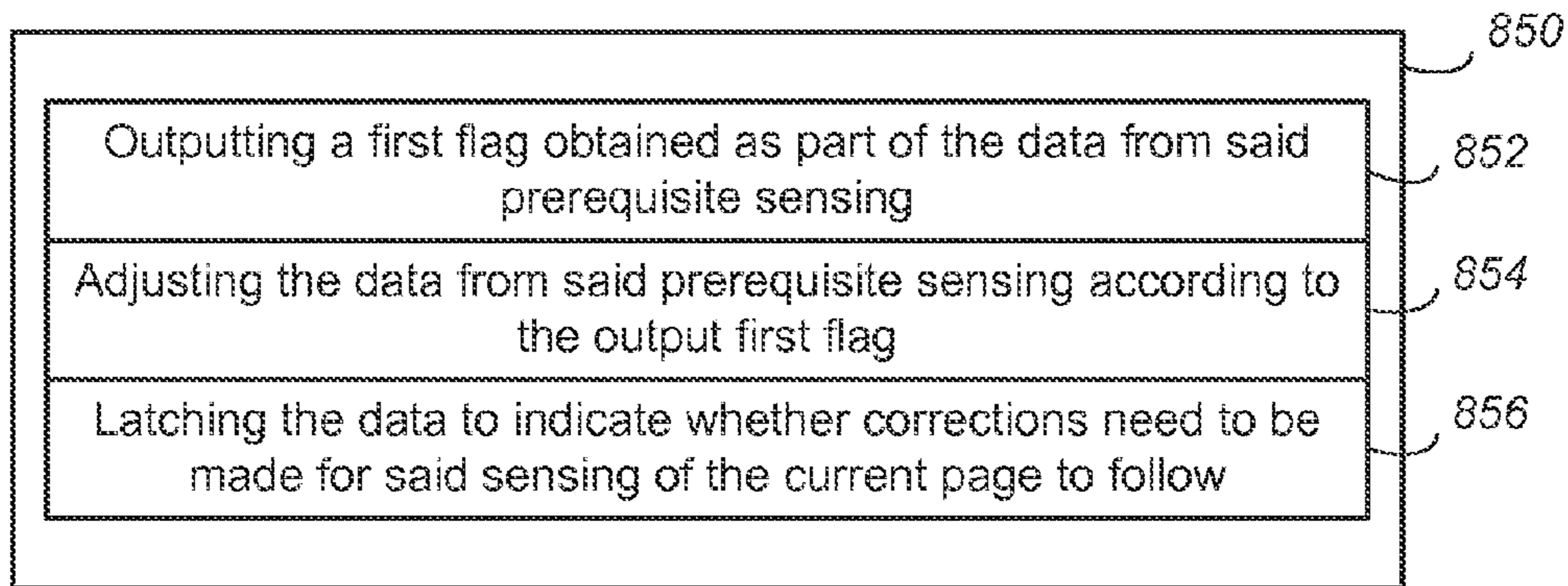
Operation of the Prerequisite Lookahead Sensing
