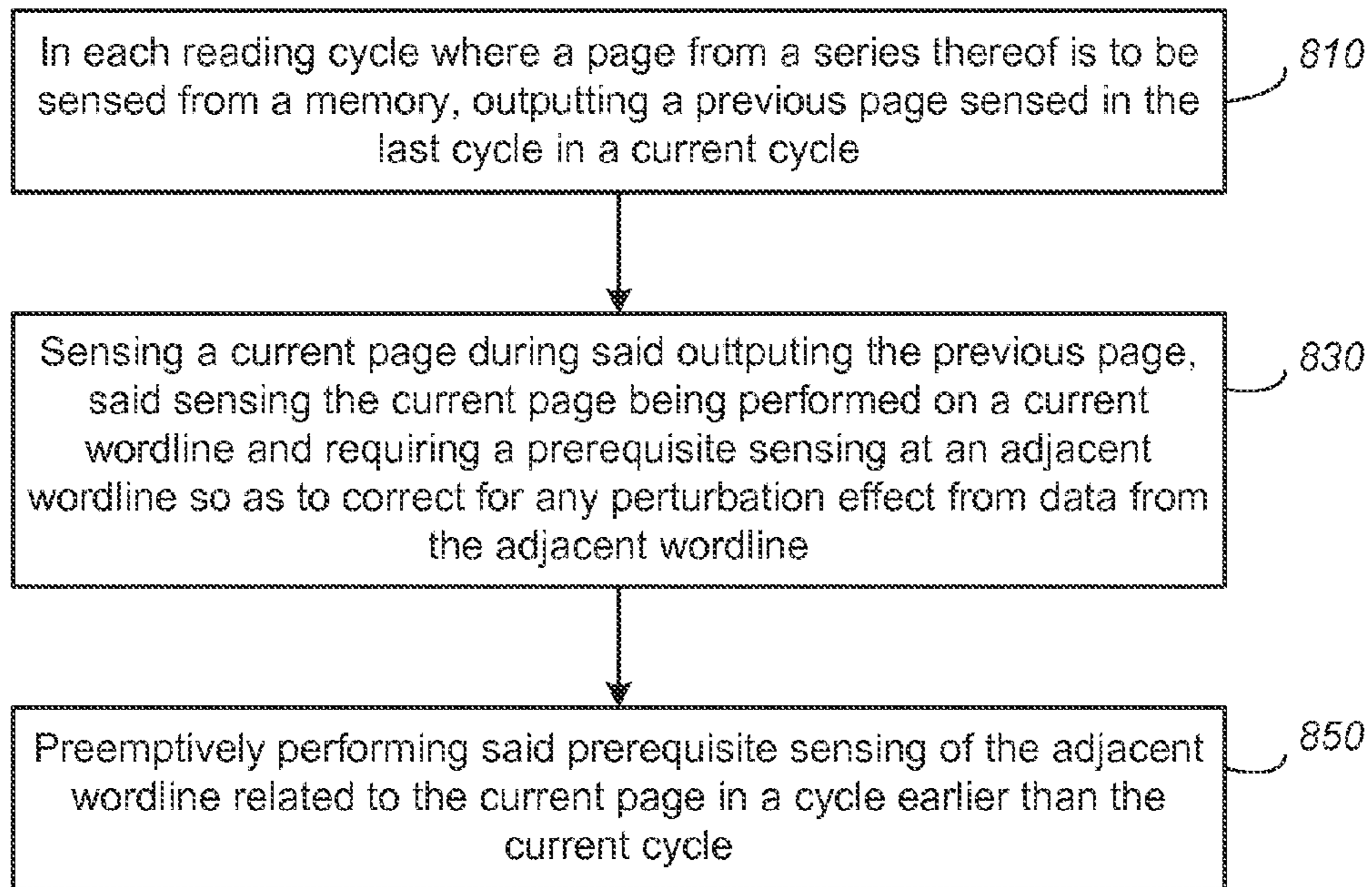
Improved Read Caching with Lookahead Correction
