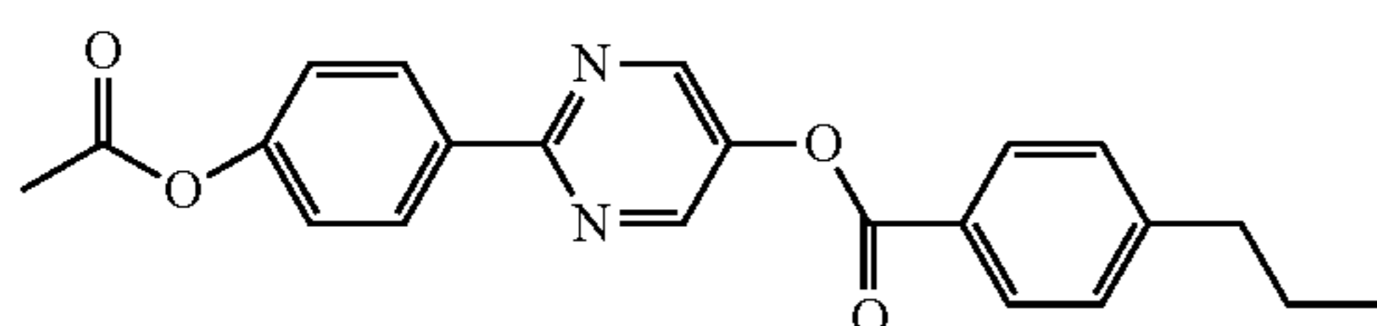
{4-[5-(4-propyl-benzoyloxy)pyrimidin-2-yl]phenyl} acetate
