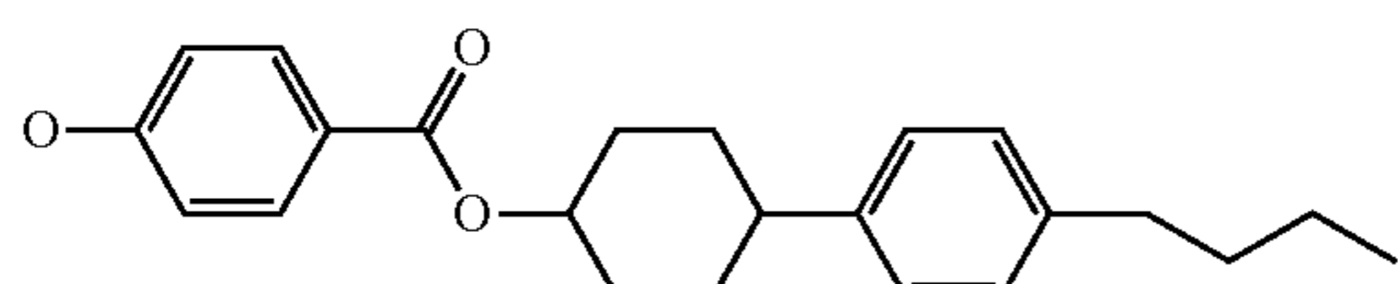
4-[4-(4-butyl-phenyl)-cyclohexyloxy]benzoic acid
