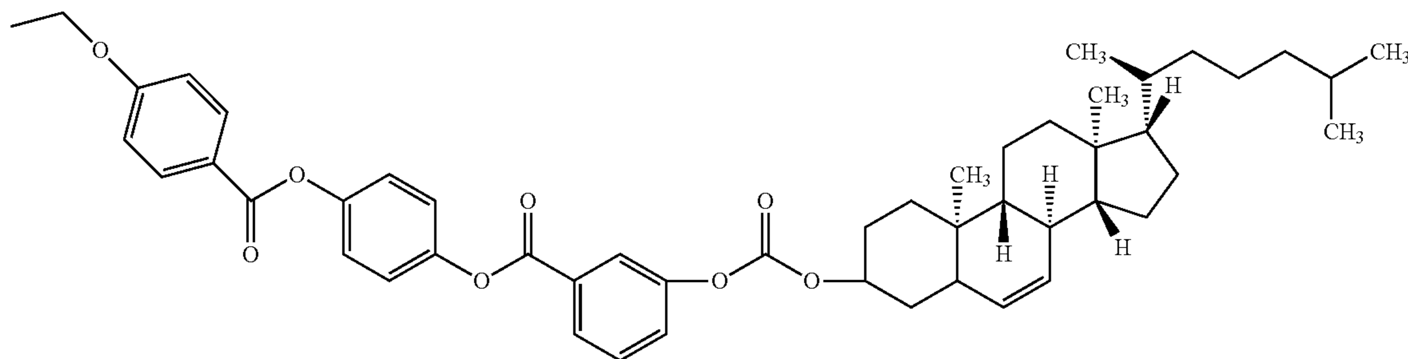
4-(4-{4-[17-(1,5-dimethyl-hexyl)-10,13-dimethyl-2,3,4,7,8,9,10,11,12,13,14,15,16,17-tetradecahydro-1H-cyclopenta[a]phenanthren-3-yloxy-carboxyloxy]-benzoyloxy}-phenoxy-carboxyl)-phenoxy-methyl
