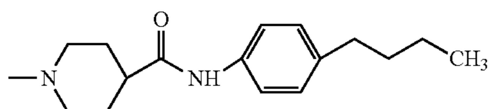
4-(4-butyl-phenylcarbamoyl)-piperidin-1-yl
