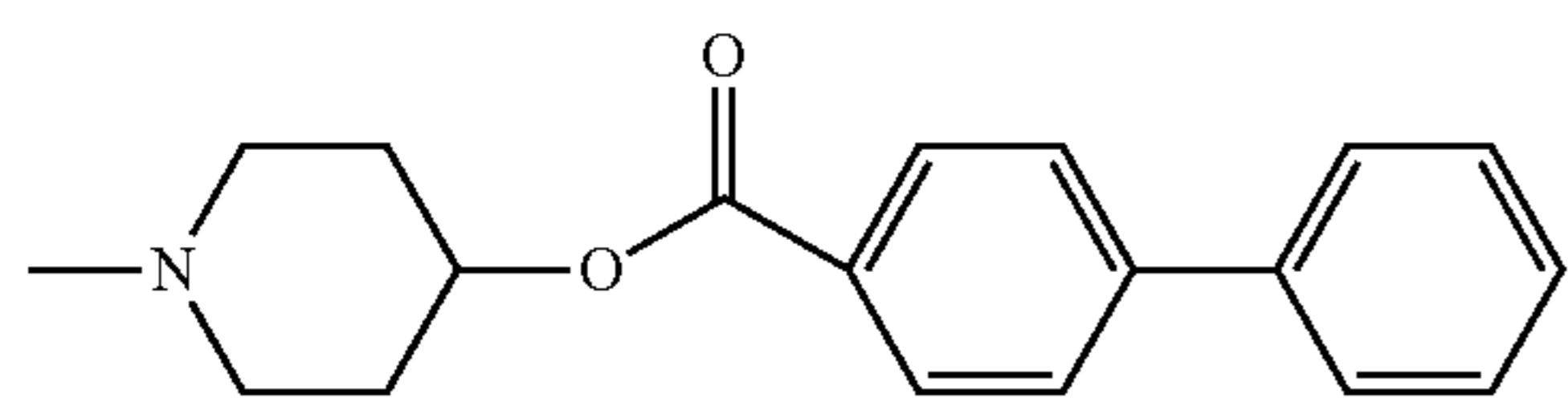
4-(biphenyl-4-carboxyloxy)-piperidin-1-yl
