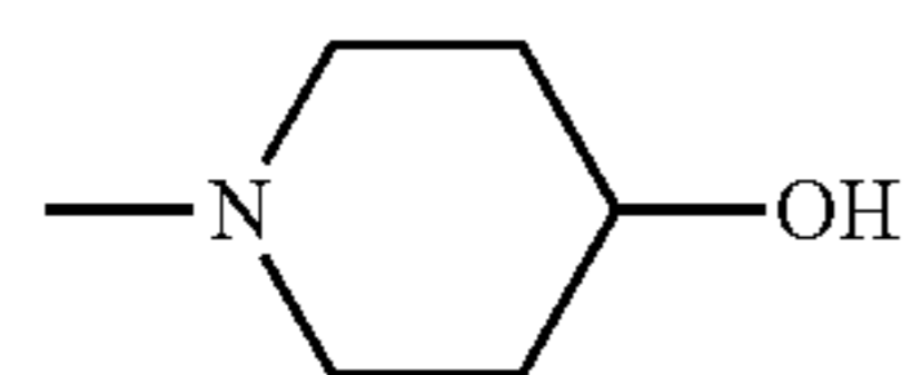
4-hydroxy-piperidin-1-yl
