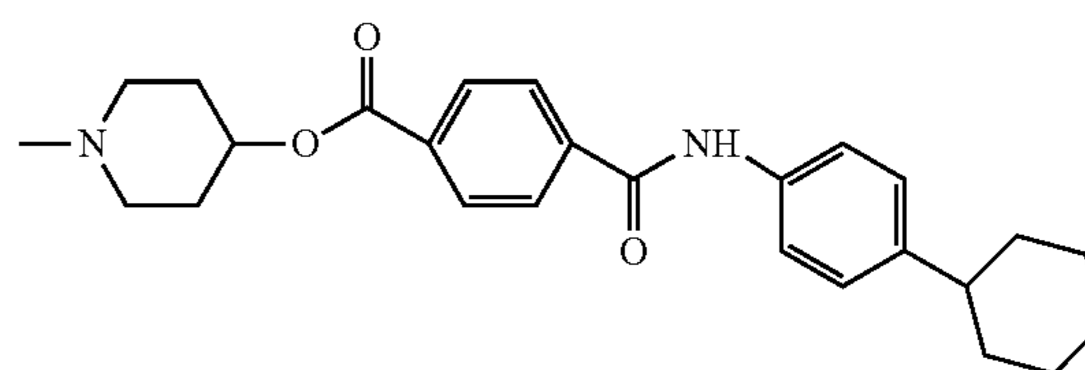
4-[4-(4-cyclohexyl-phenylcarbamoyl)-benzyloxy]-piperidin-1-yl
