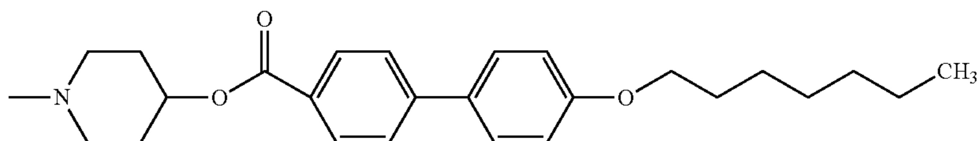
4-(4'-hexyloxy-biphenyl-4-carbonyloxy)-piperidin-1-yl
