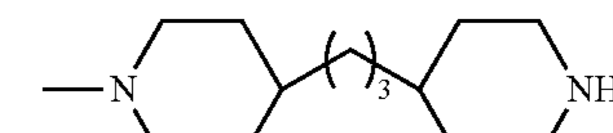
4-(3-piperidin-4-yl-propyl)-piperidin-1-yl
