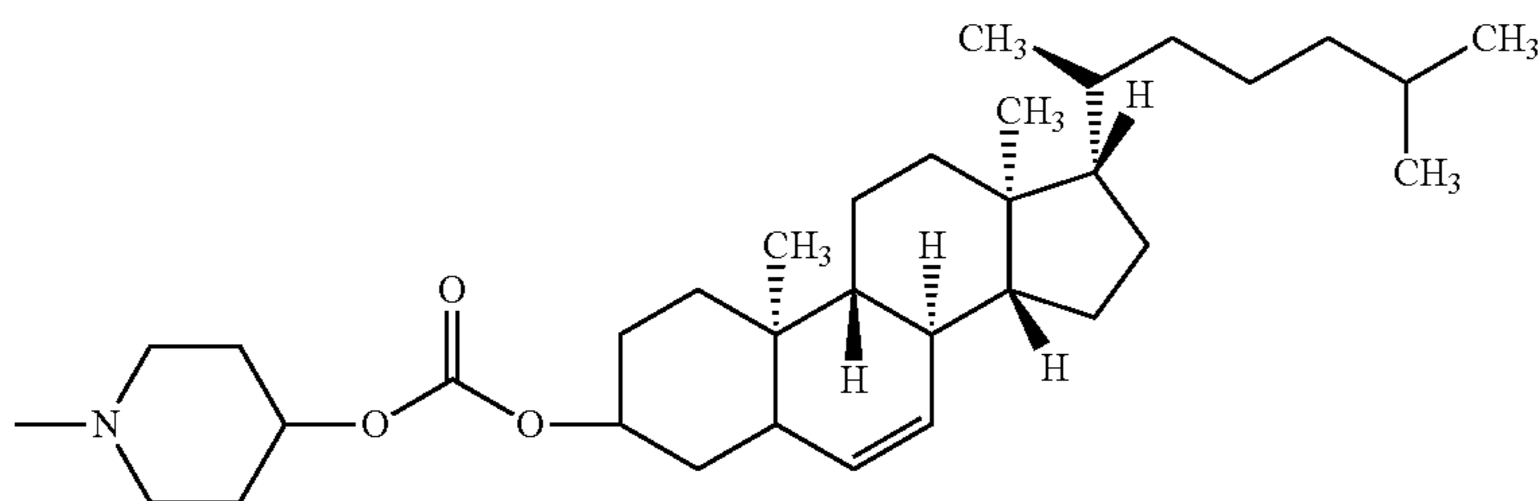
4-[17-(1,5-dimethyl-hexyl)-10,13-dimethyl-2,3,4,7,8,9,10,11,12,13,14,15,16,17-tetradecahydro-1H-cyclopenta[a]phenanthren-3-yloxy-carbonyloxy]-piperidin-1-yl
