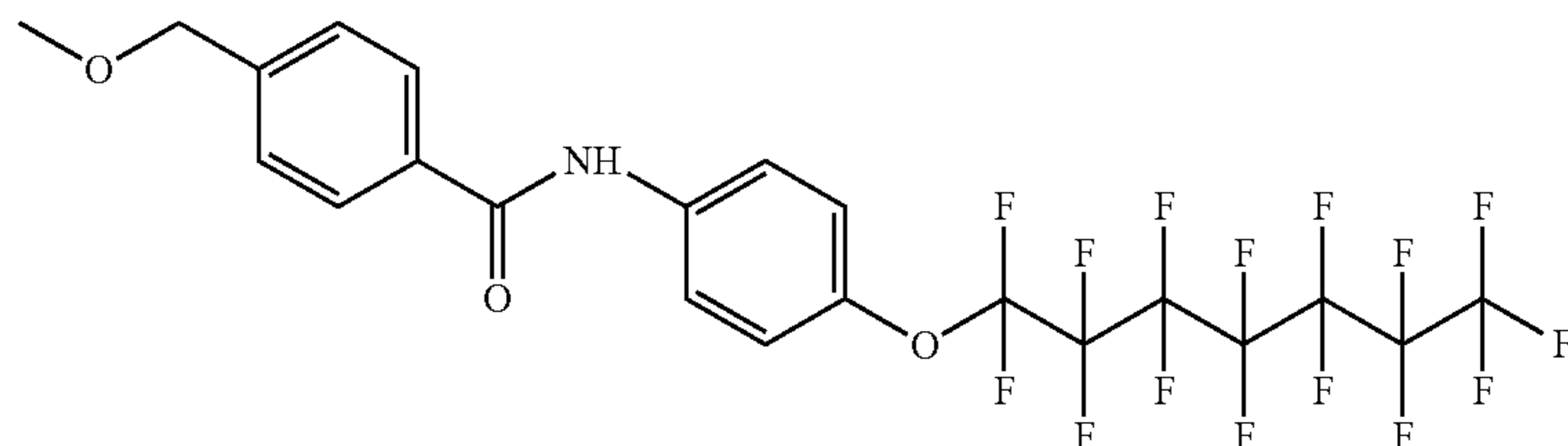
4-(4-pentadecafluoroheptyloxy-phenylcarbamoyl)-benzyloxy
