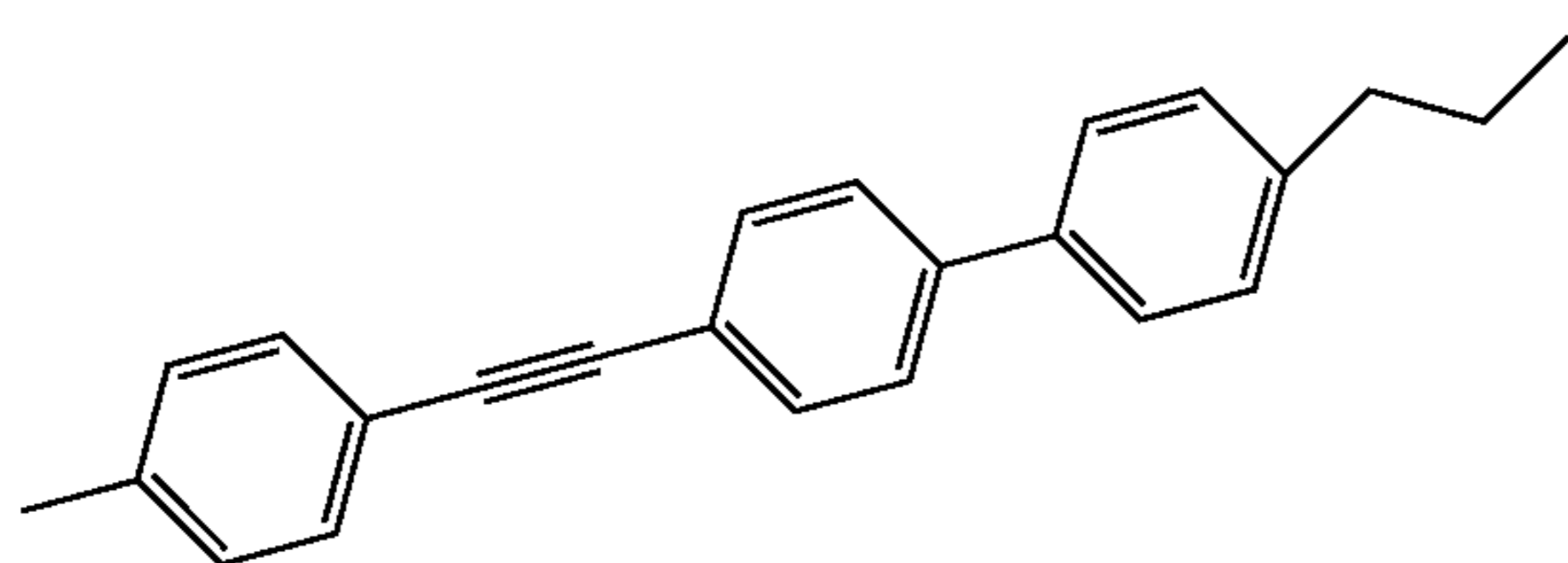
4-(4'-propyl-biphenyl-4-ylethynyl)-phenyl
