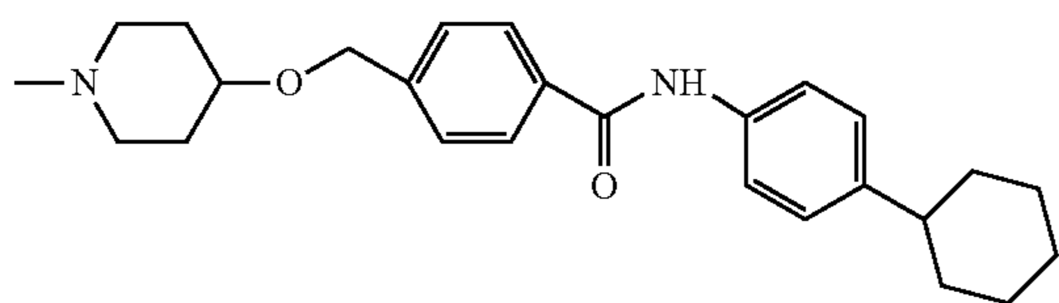
4-[4-(4-cyclohexyl-phenylcarbamoyl)-benzyloxy]-piperidin-1-yl
