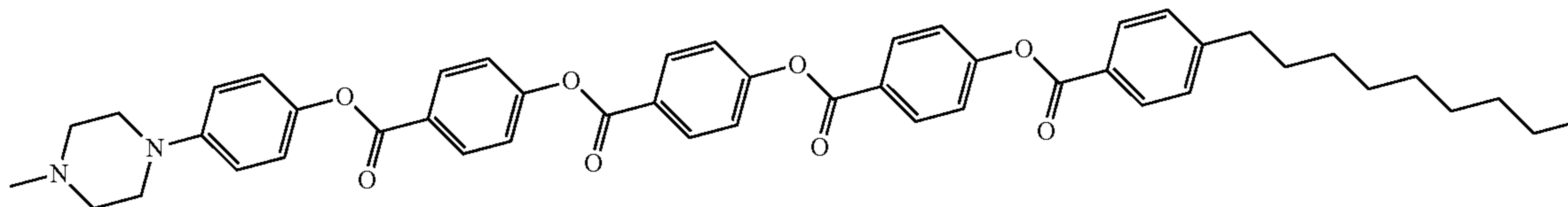
{4-[4-(4-(4-[4-(4-nonyl-benzoyloxy)-benzoyloxy]-benzoyloxy)-benzoyloxy)-phenyl]-piperazin-1-yl}
