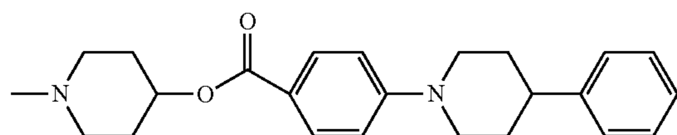
4-(4-(4-phenylpiperidin-1-yl)-benzoyloxy)-piperidin-1-yl
