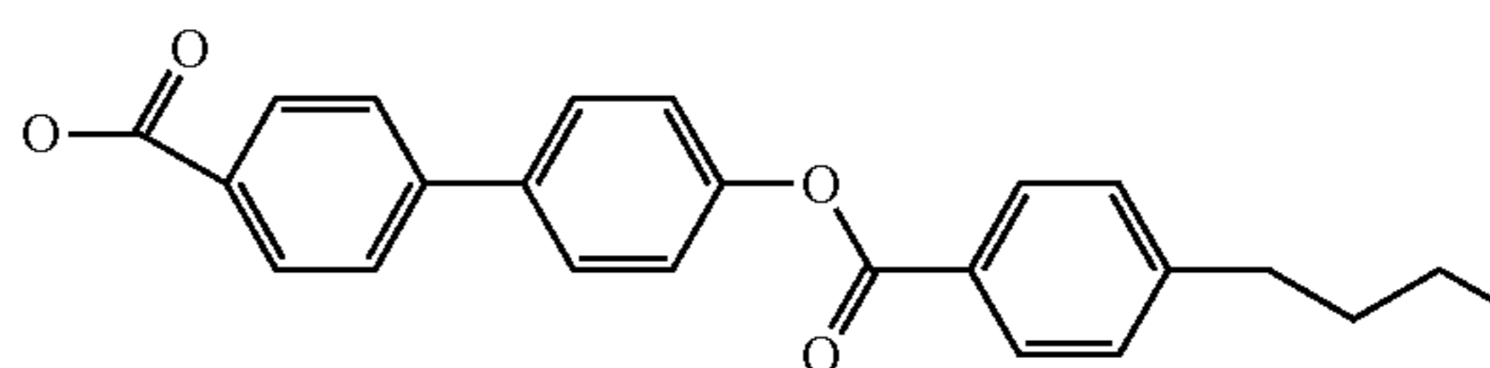
4'-[4-(4-butyl-phenyl)-benzoyloxy]biphenyl-4-carboxylic acid
