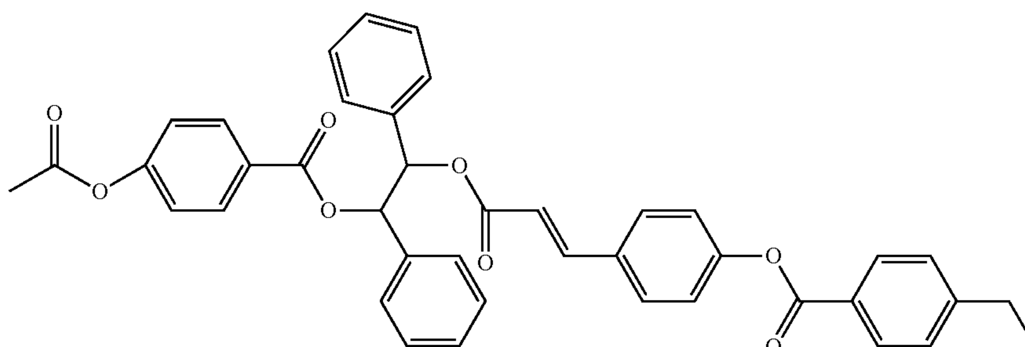
[4-(1,2-diphenyl-2-{3-[4-(4-propyl- benzoyloxy)-phenyl]-acryloyloxy}- ethoxycarbonyl)-phenyl] ester
