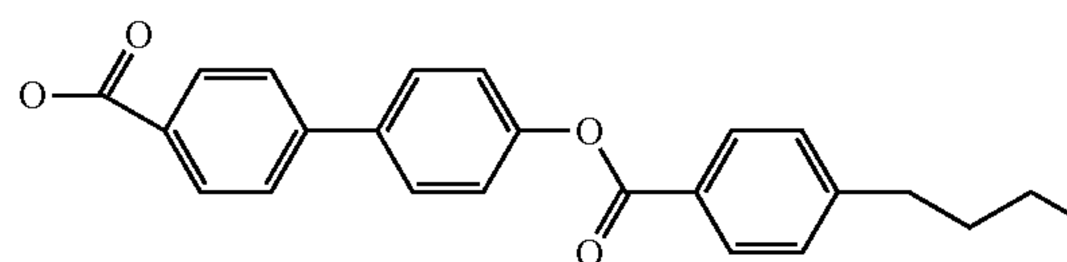
4'-[4-(4-butyl-benzoyloxy)]biphenyl-4- carboxylic acid
