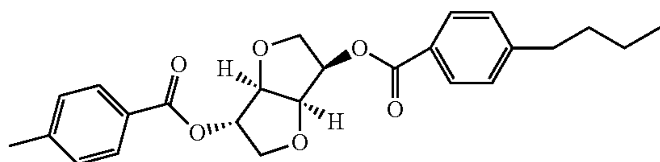
4-(6-(4-butylphenyl)carbonyloxy-(4,8-dioxabicyclo[3.3.0]oct-2-yl)oxycarbonyl)phenyl
