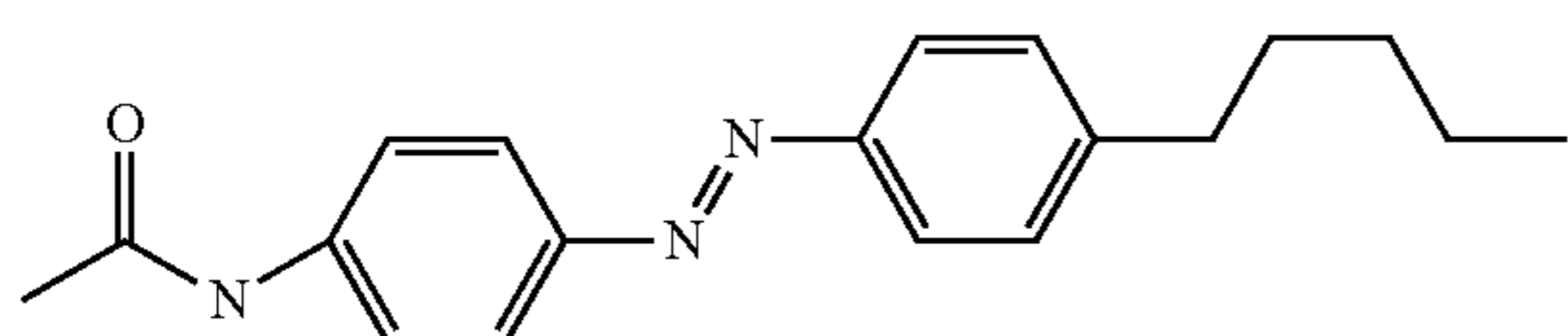
4-(4-pentyl-phenylazo)phenylacetamide
