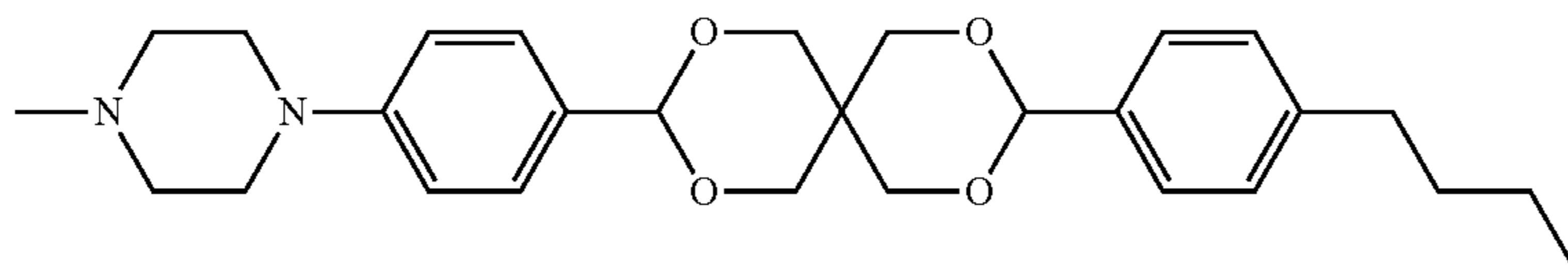
4-(4-(9-(4-butylphenyl)-2,4,8,10-tetraoxaspiro[5.5]undec-3-yl)phenyl)piperazin-1-yl
