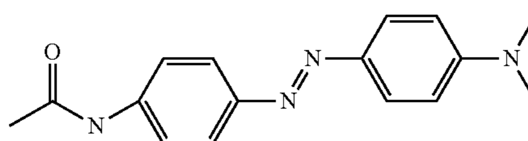
4-(4-dimethylamino-phenylazo)phenylacetamide
