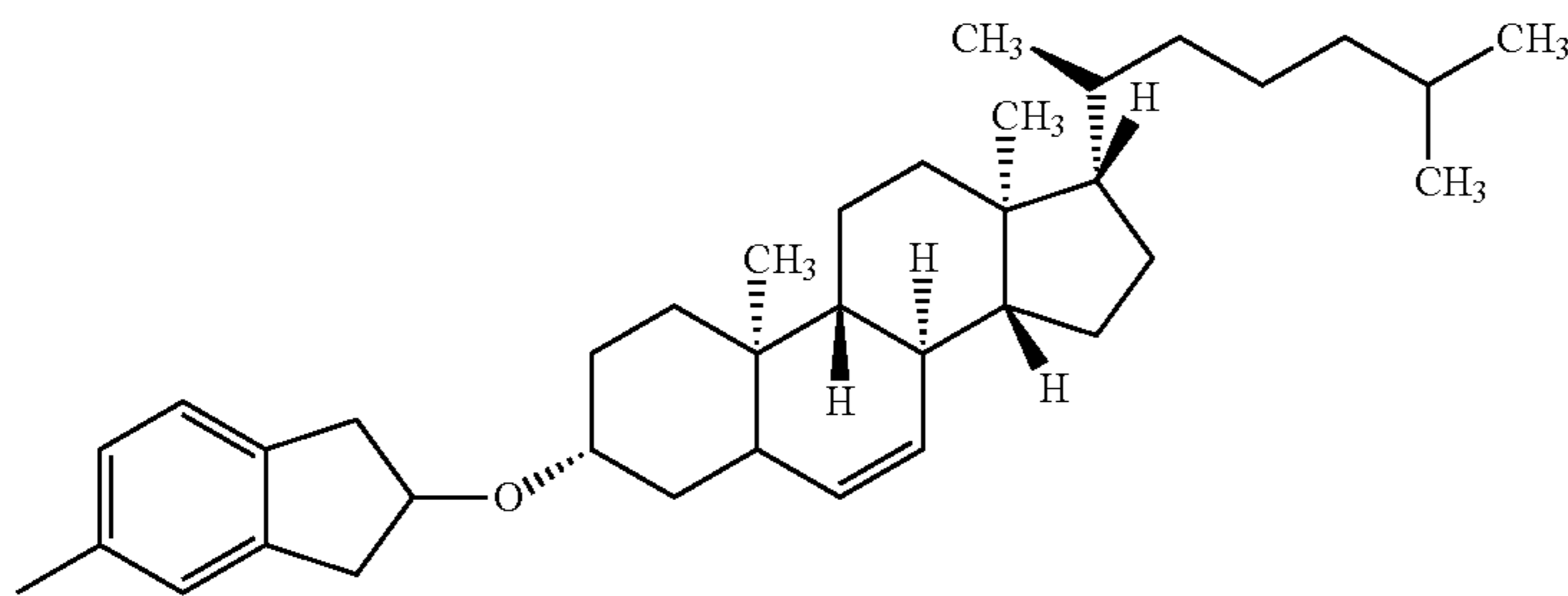
2-[17-(1,5-dimethyl-hexyl)-10,13-dimethyl-2,3,4,7,8,9,10,11,12,13,14,15,16,17-tetradecahydro-1H-cyclopenta[a]phenanthren-3-yloxy]-indan-5-yl
