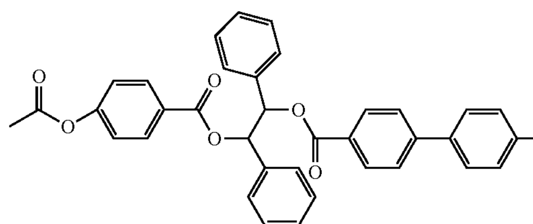
{4-[2-(4'-methyl-biphenyl-4-carboxyloxy)- 1,2-diphenyl-ethoxycarbonyl]-phenyl} ester
