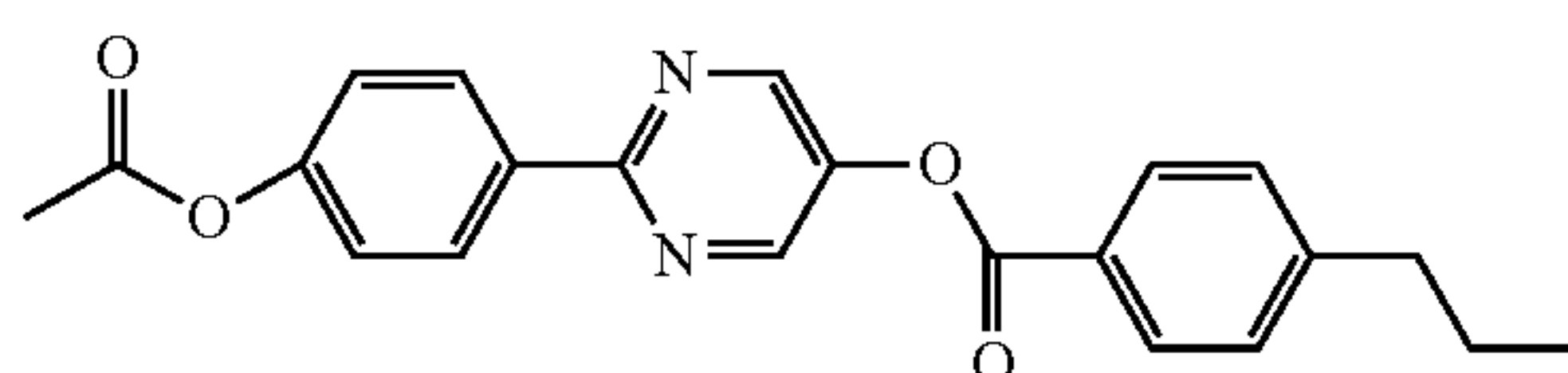
{4-[5-(4-propyl-benzoyloxy)-pyrimidin-2- yl]-phenyl} ester
