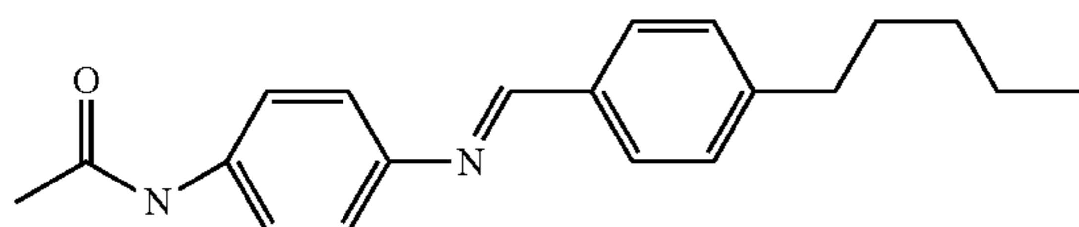
N-{4-[(4-pentyl-benzylidene)-amino]-phenyl}-acetamidyl
