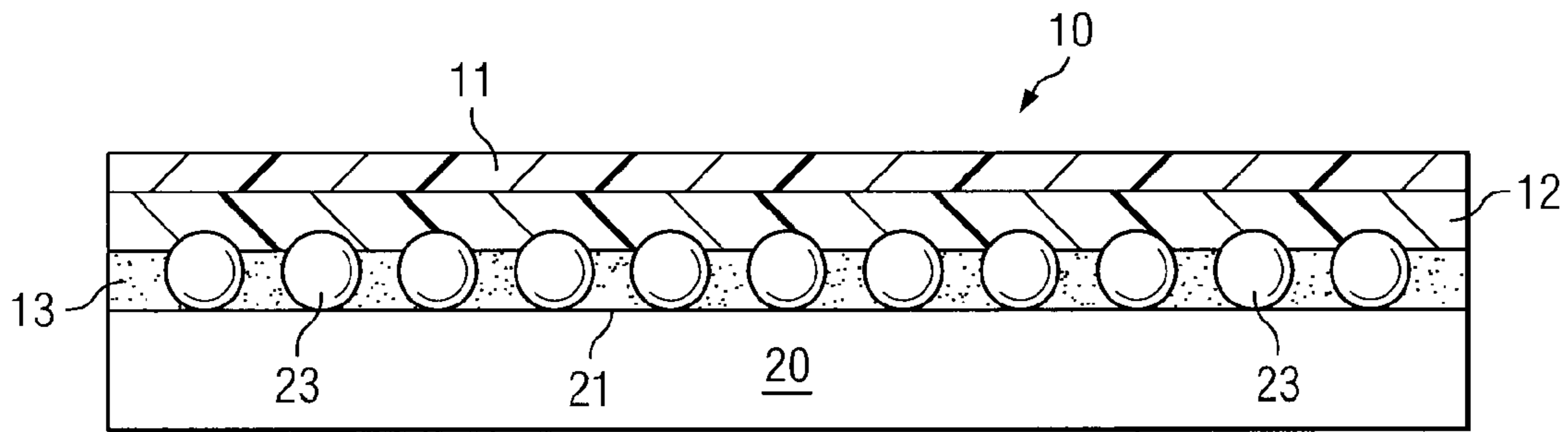
FIG. 1 (PRIOR ART)
