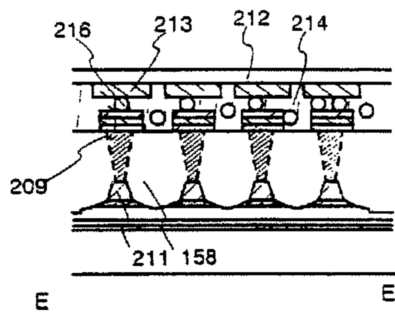
FIG. 7B cross sectional view of E-E'
