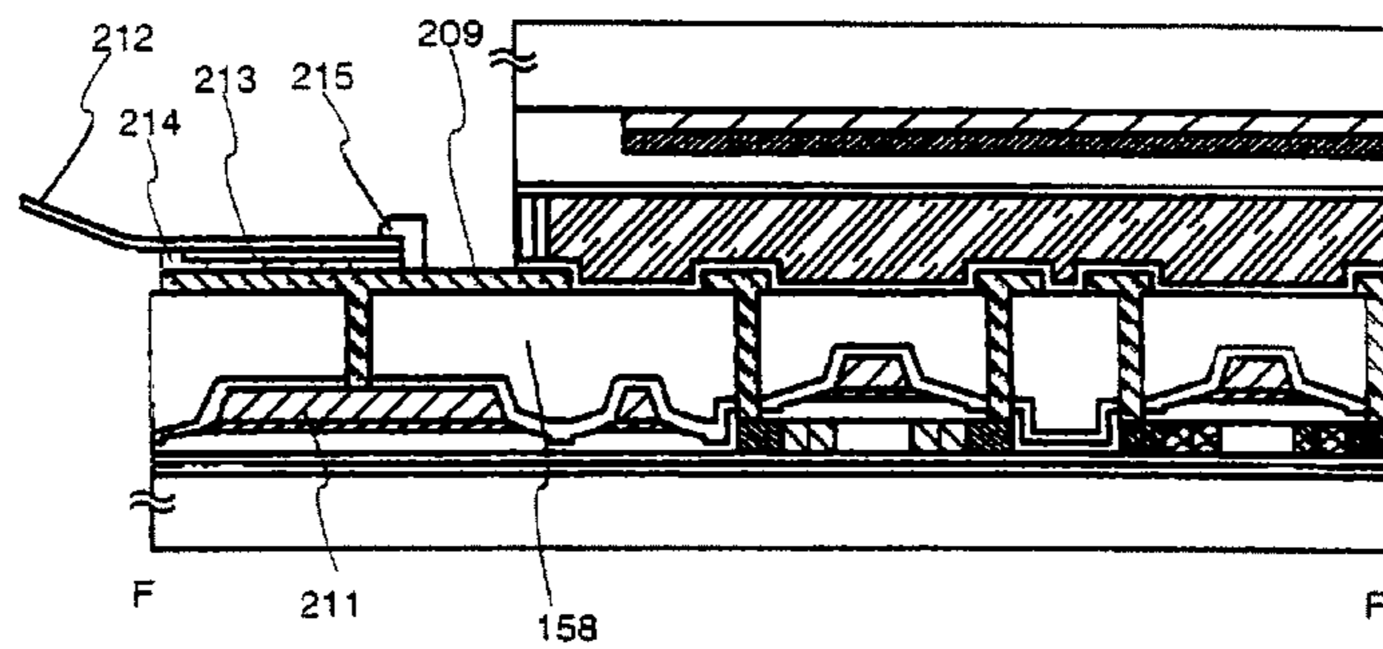
FIG. 8A cross sectional view of F-F'
