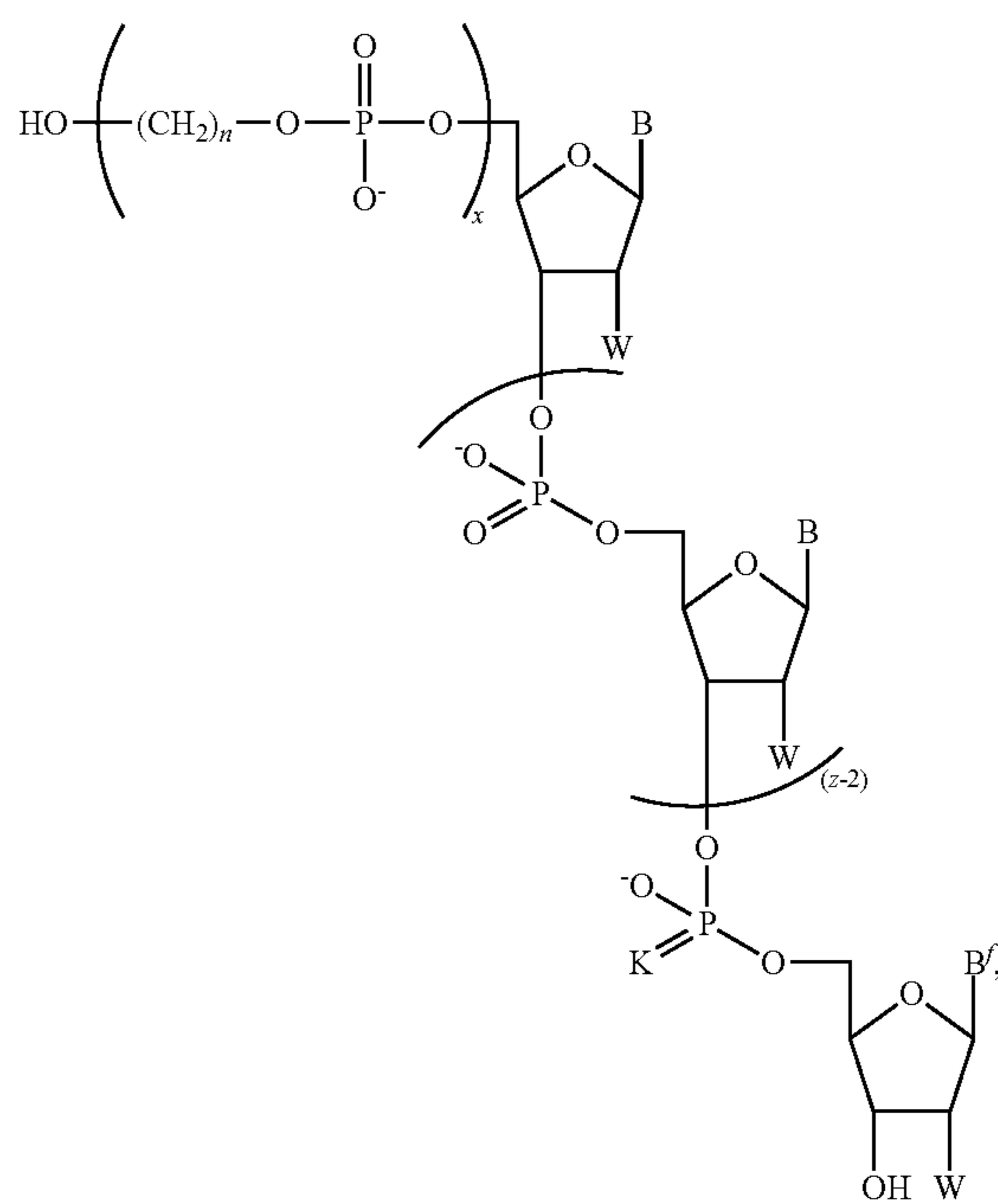
Formula I-F
