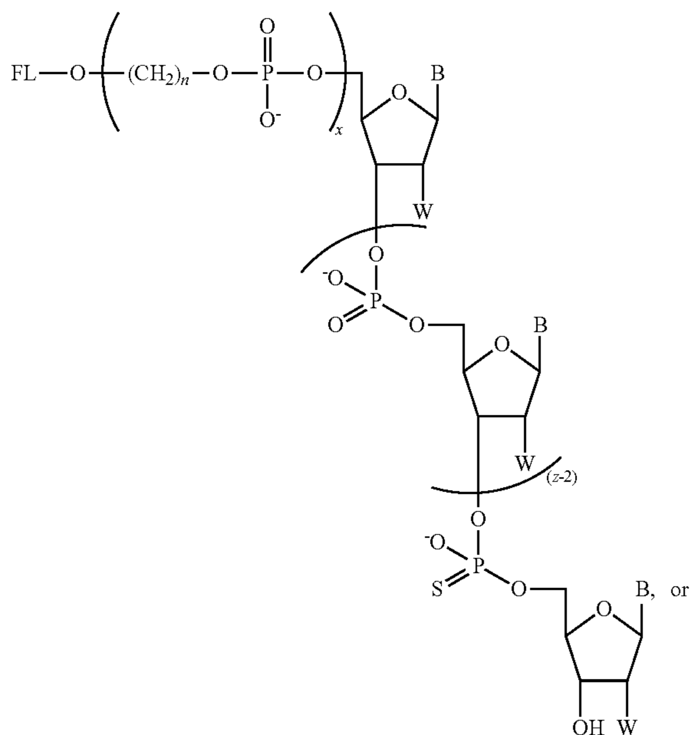
Formula I-J
