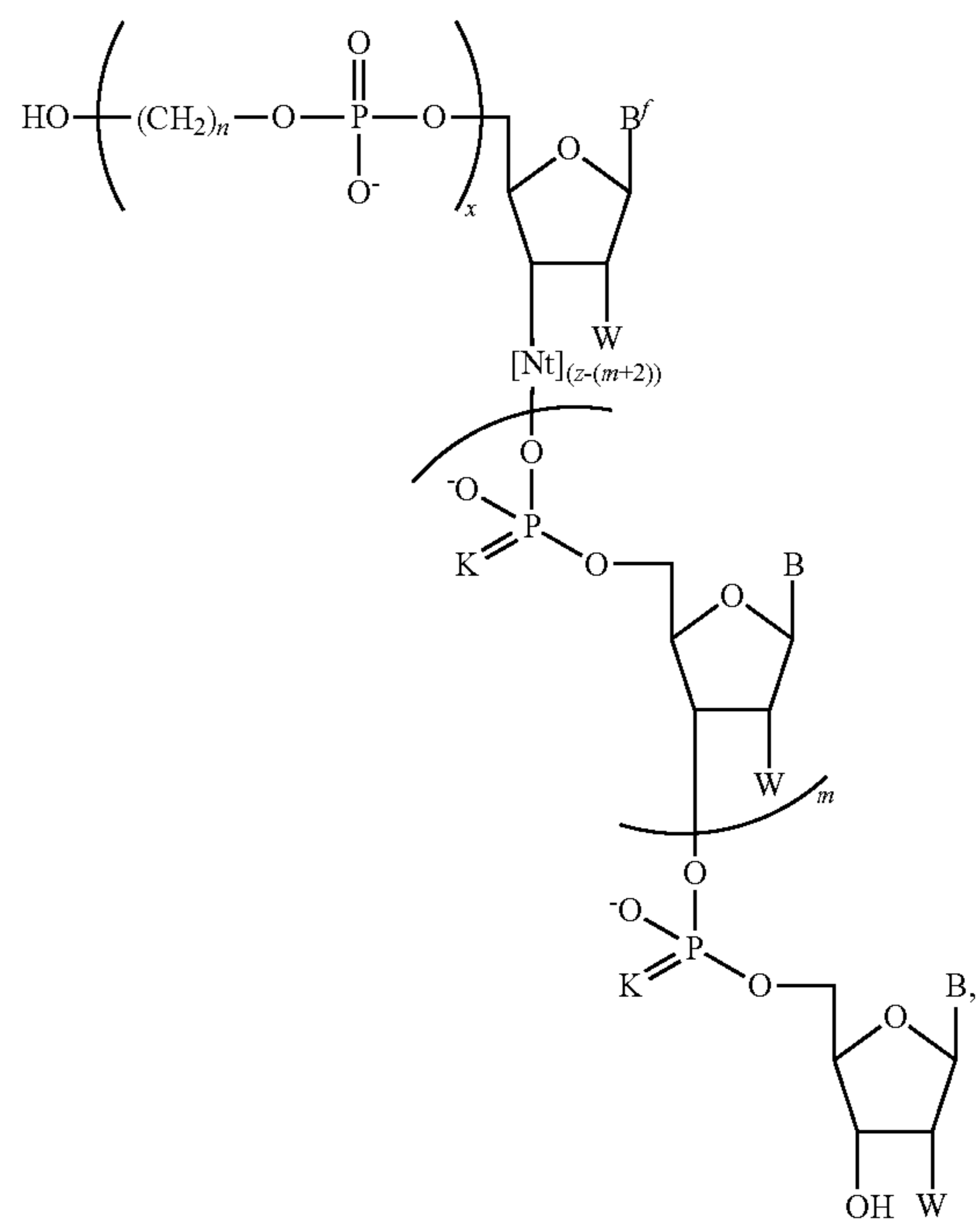
Formula I-C
