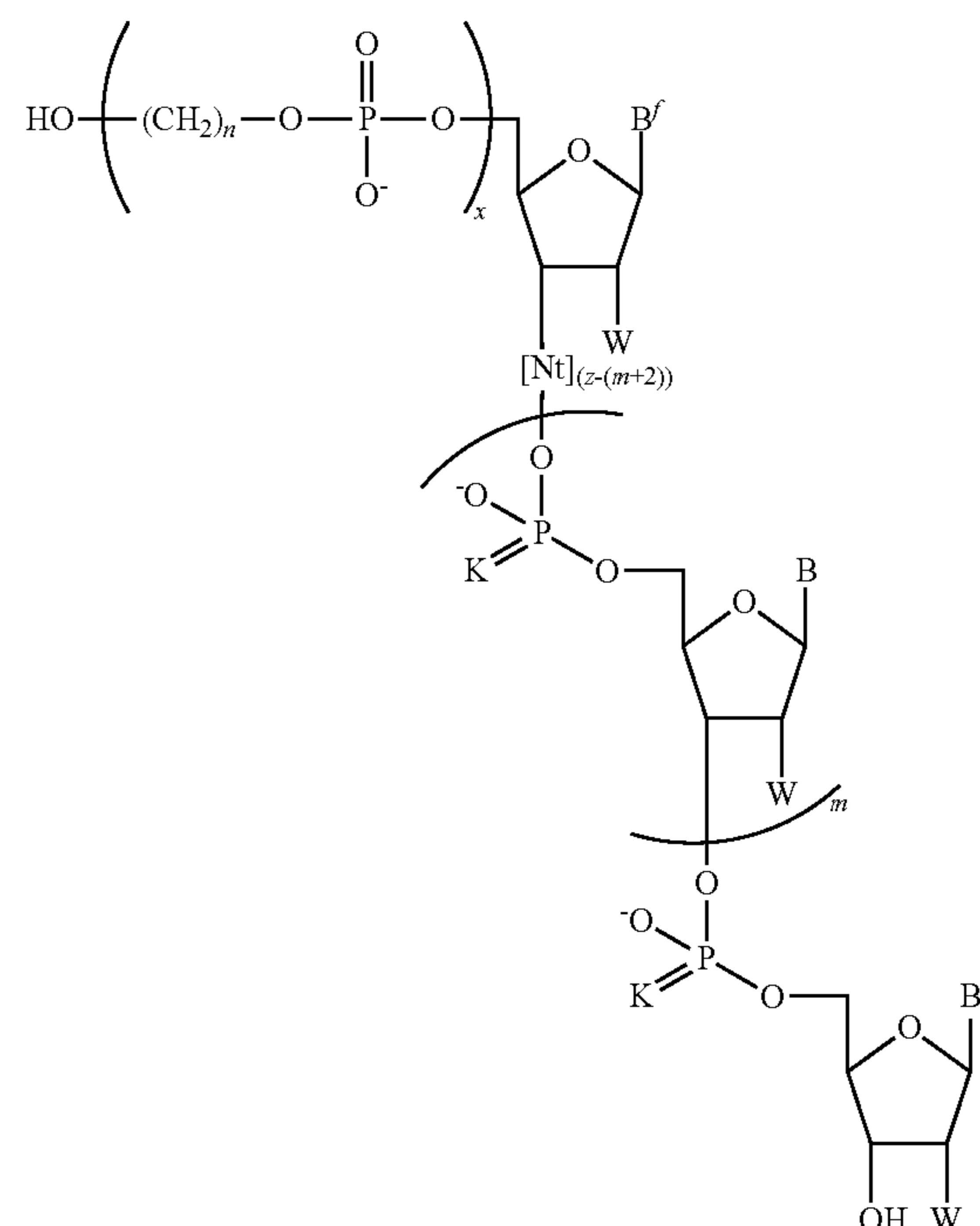
Formula I-C
