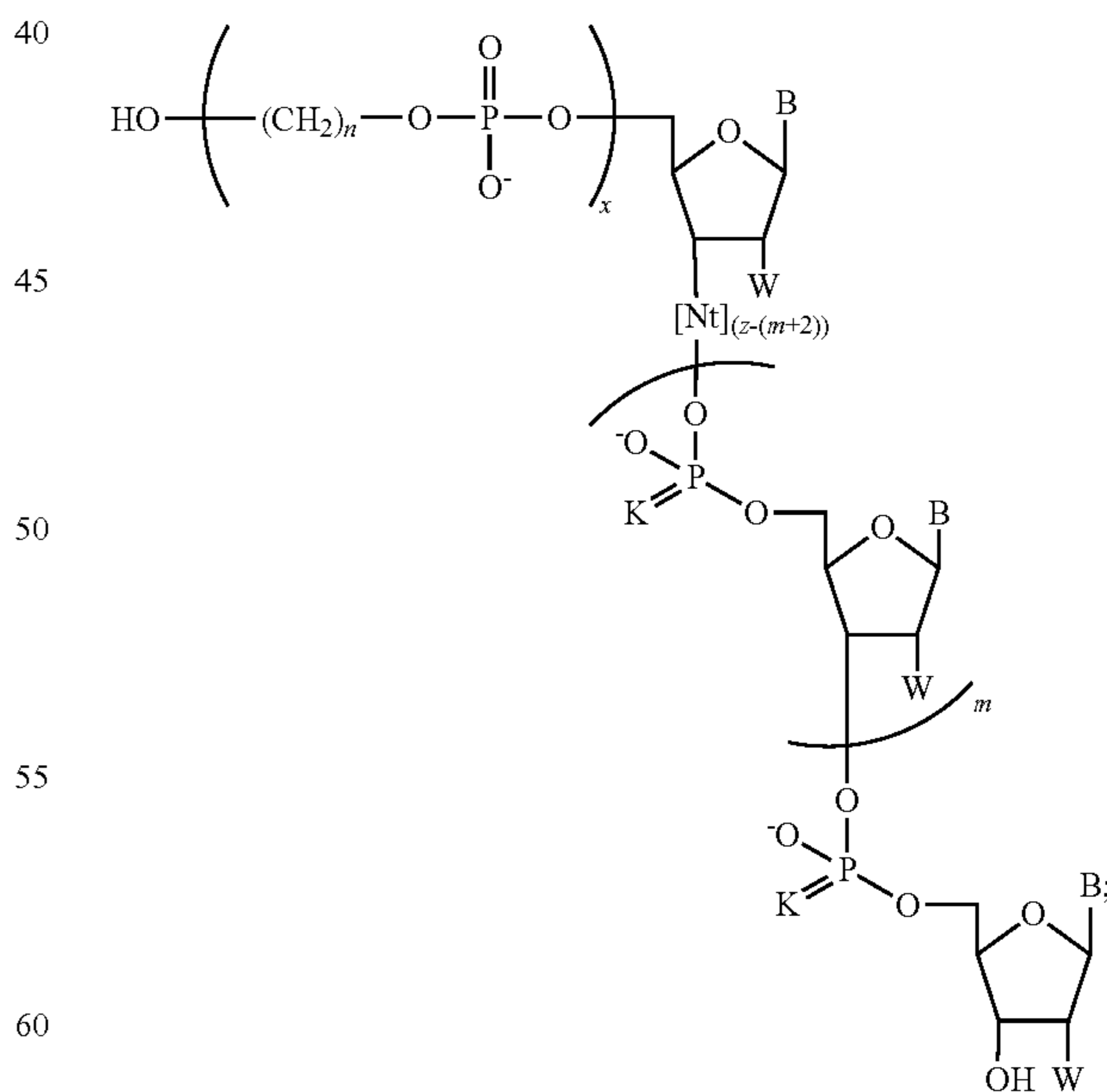
Formula I
