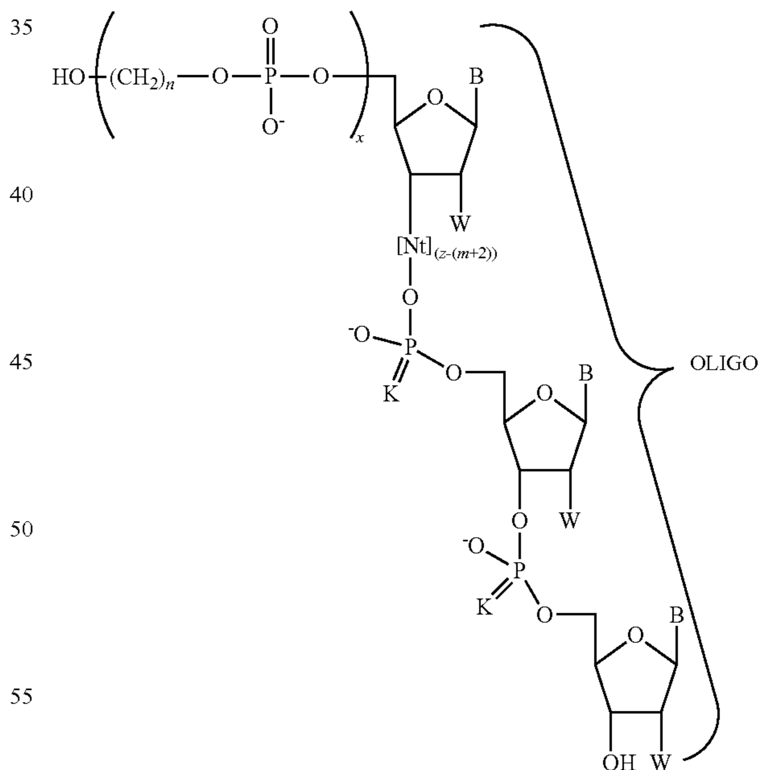
Formula I-J
