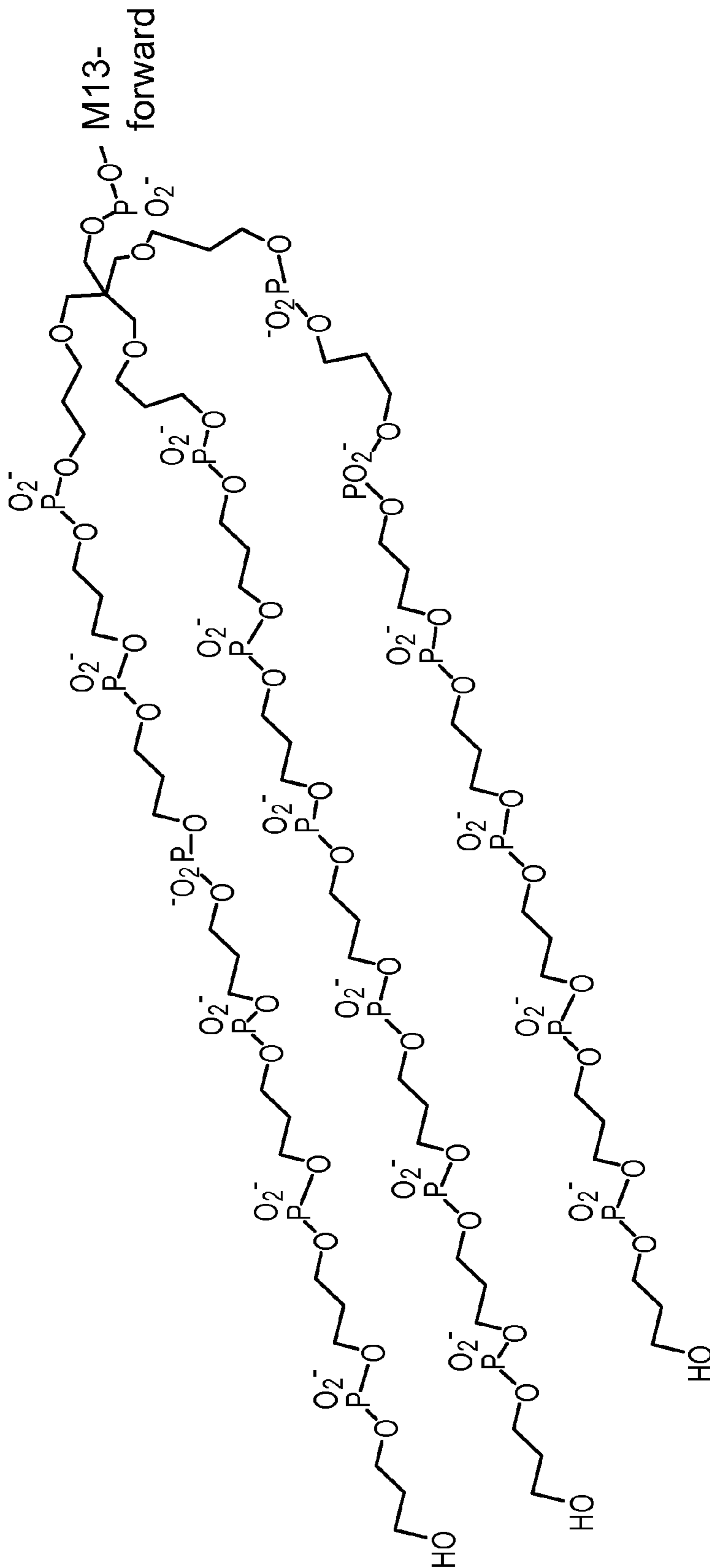
(C3) 6 -treb-M13-forward
