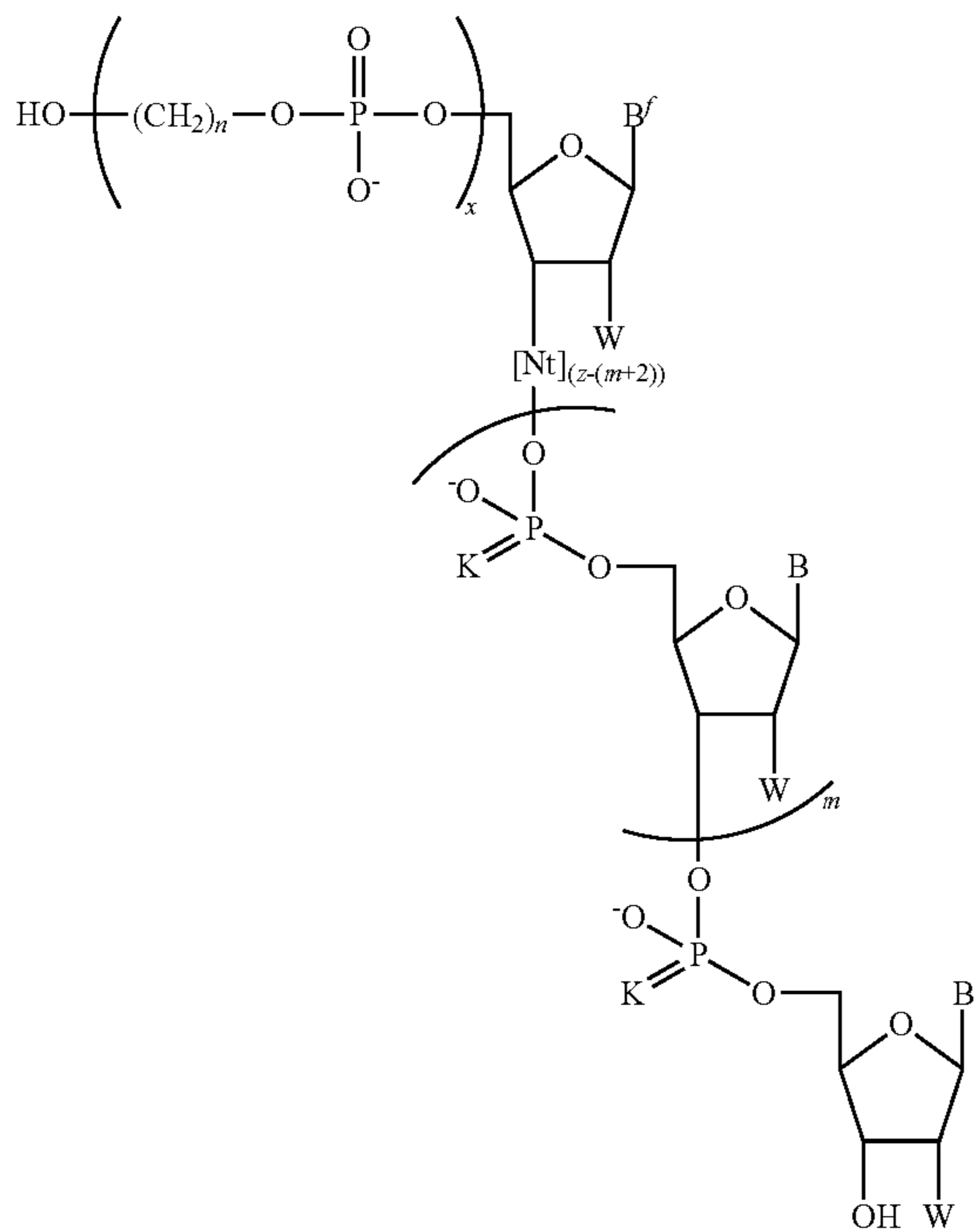
Formula I-C
