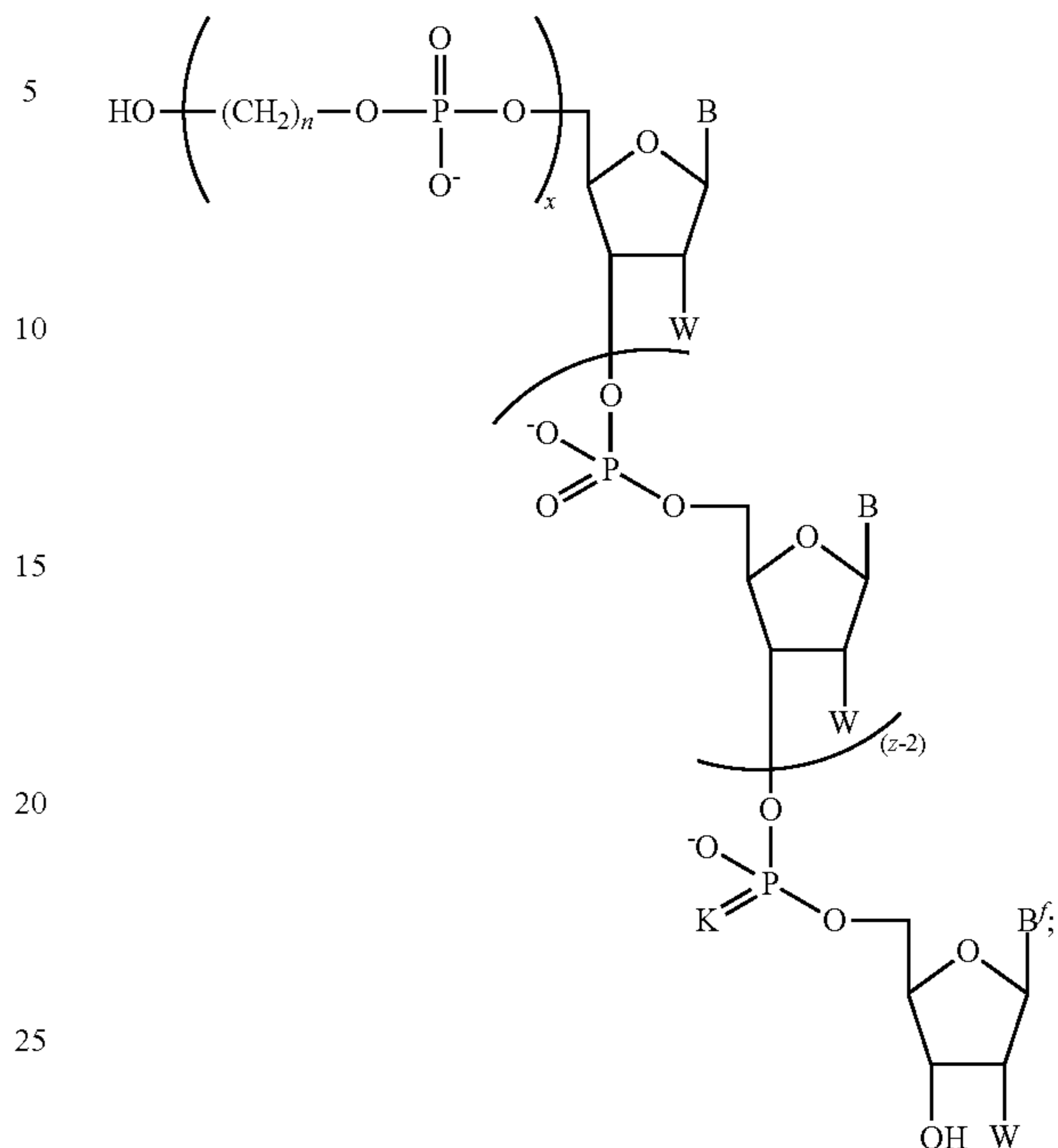
Formula I-H
