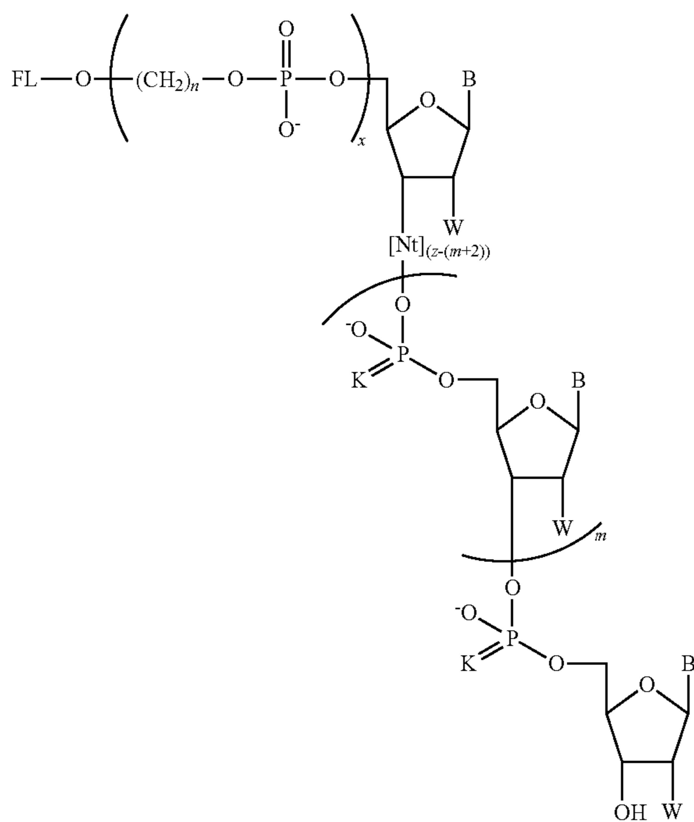
Formula I-D
