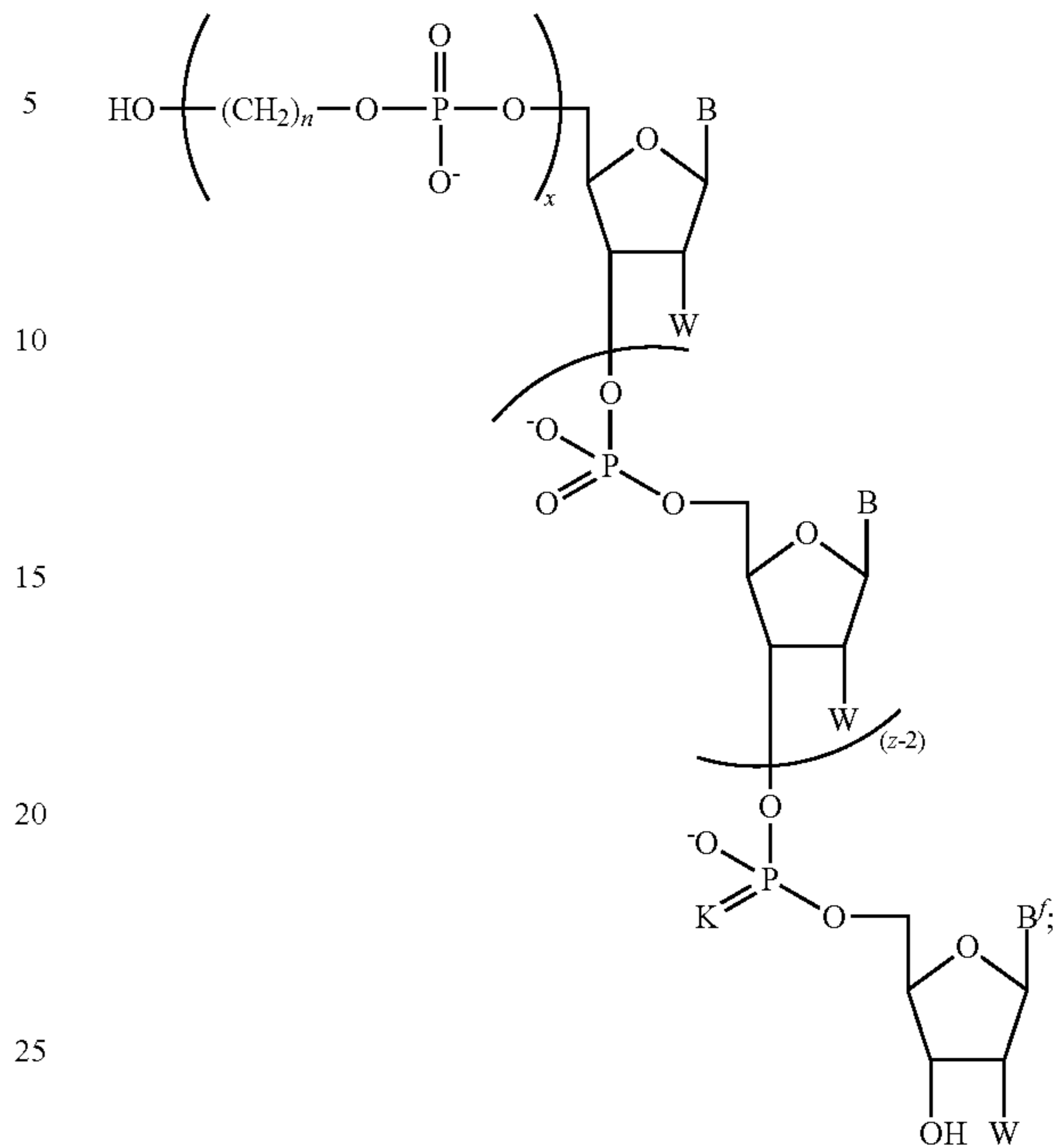
Formula I-H
