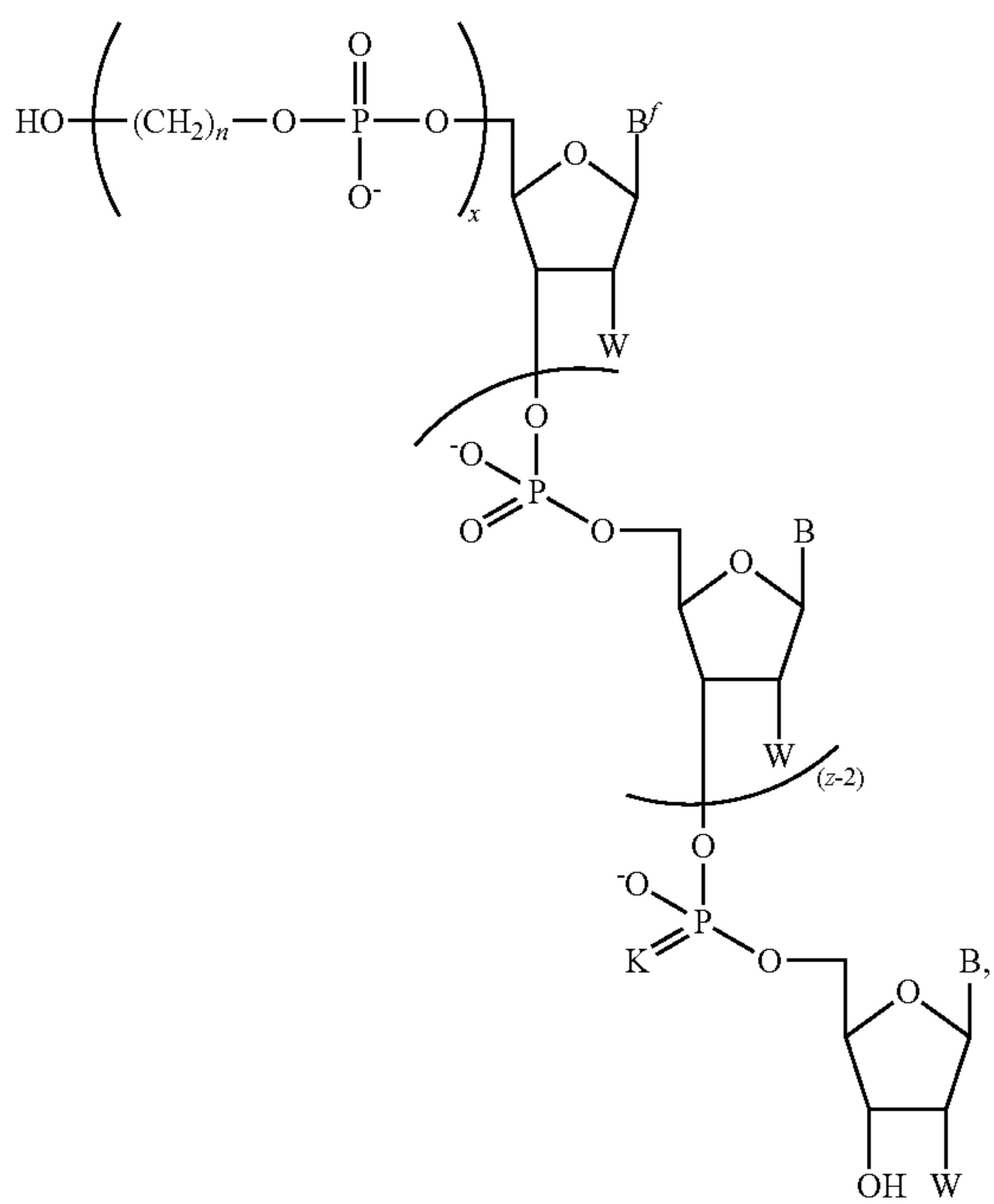
Formula I-E
