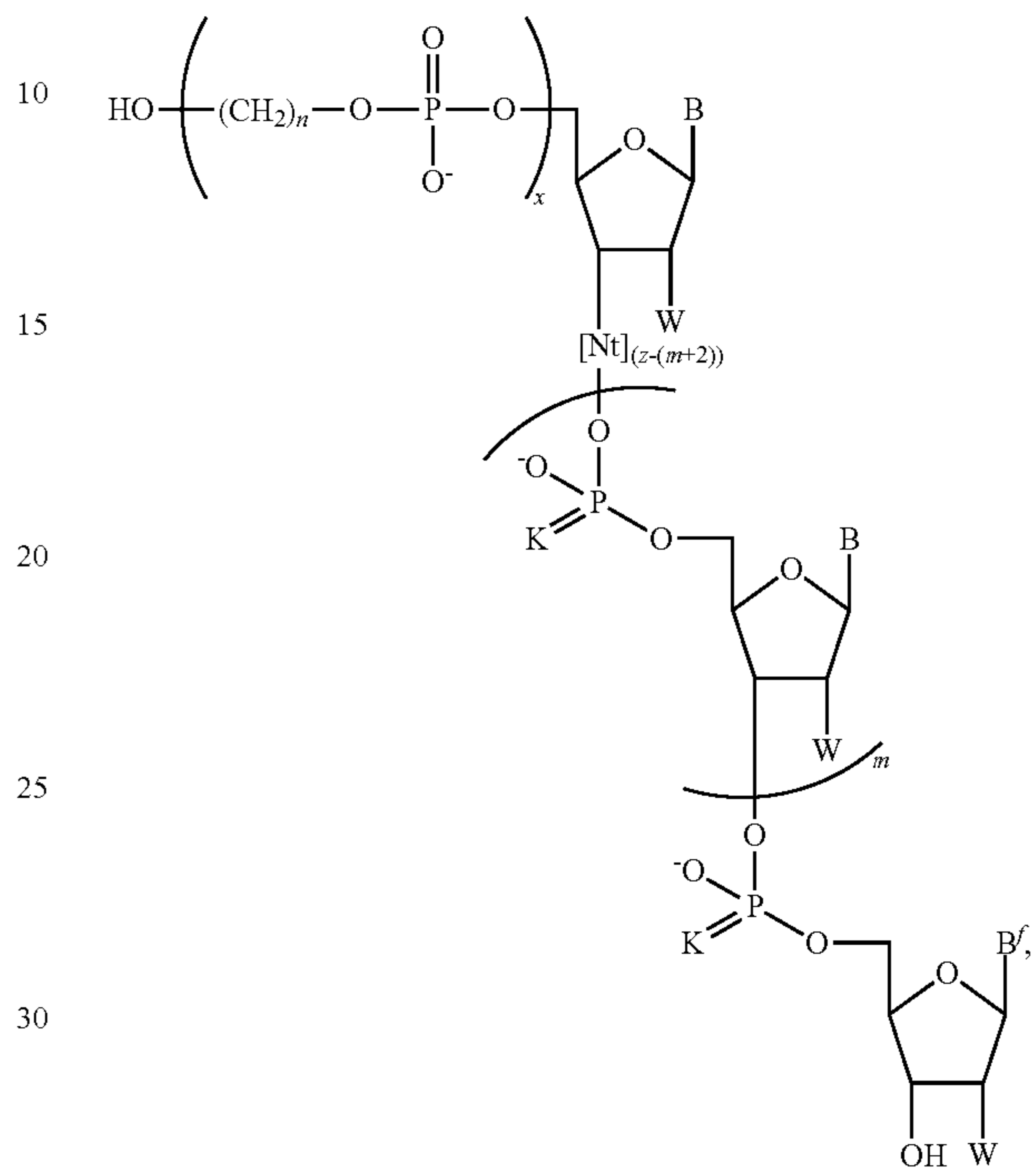
Formula I-B
