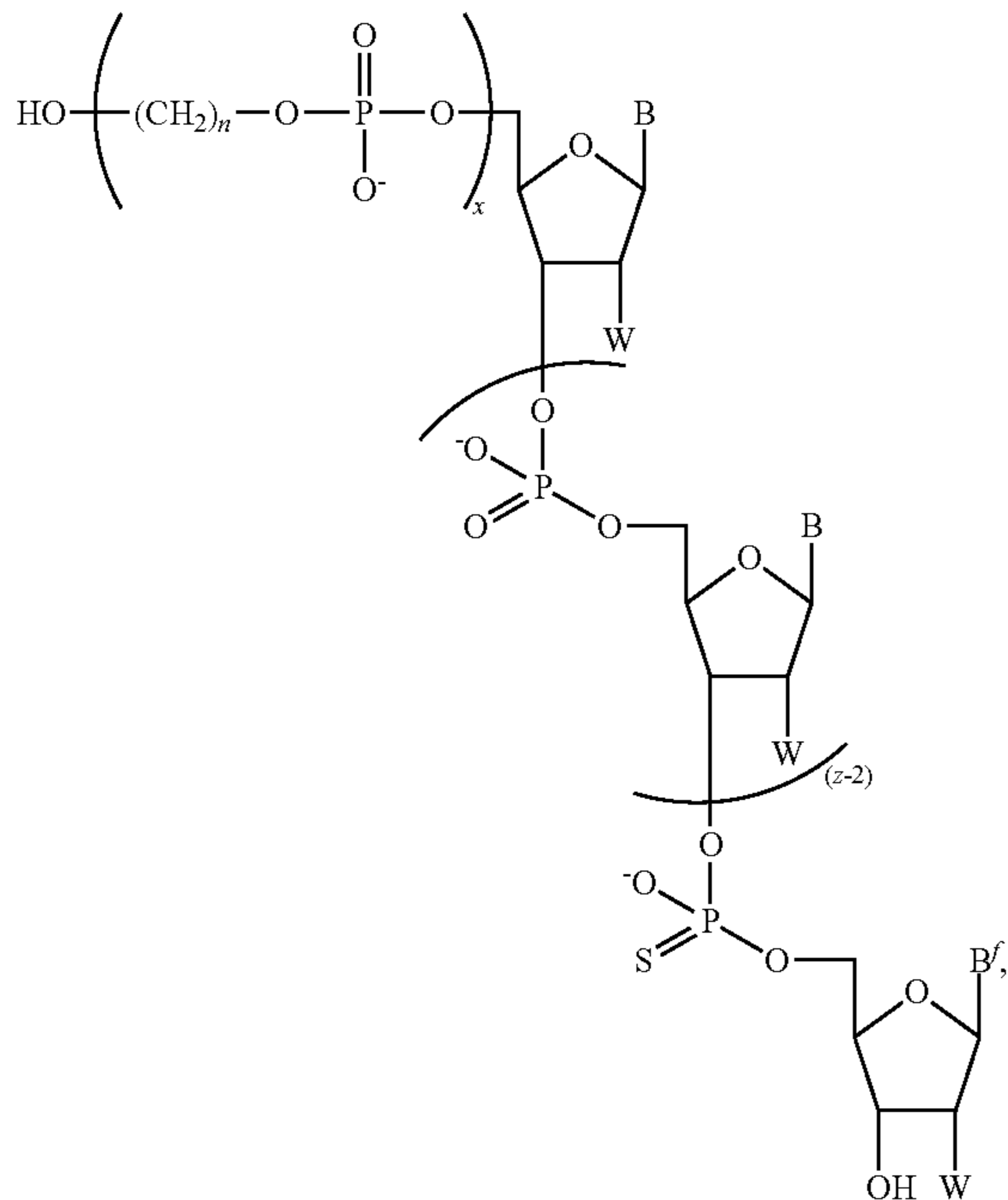
Formula I-H
