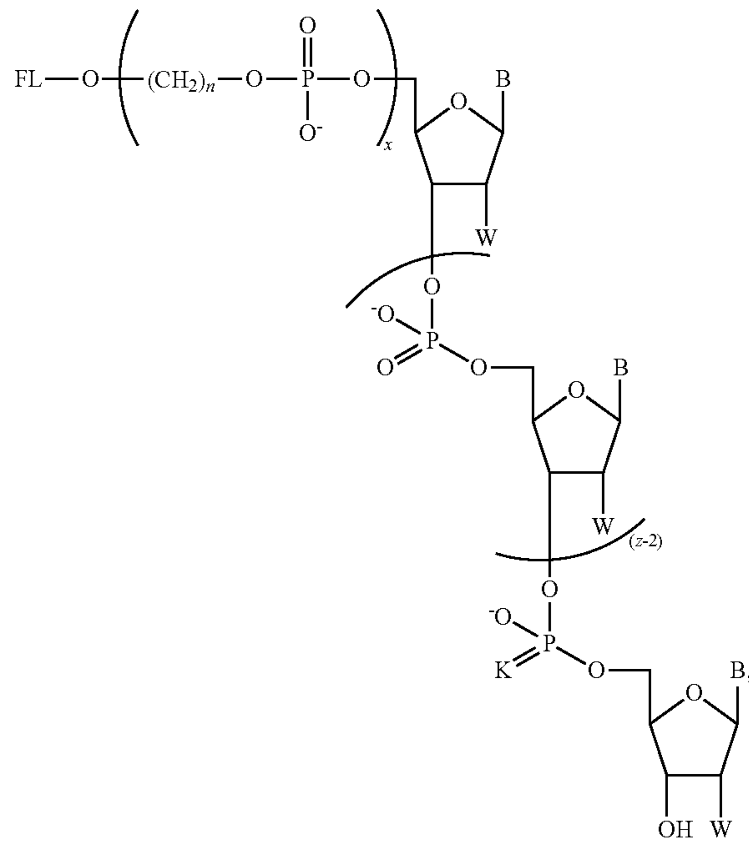
Formula I-G
