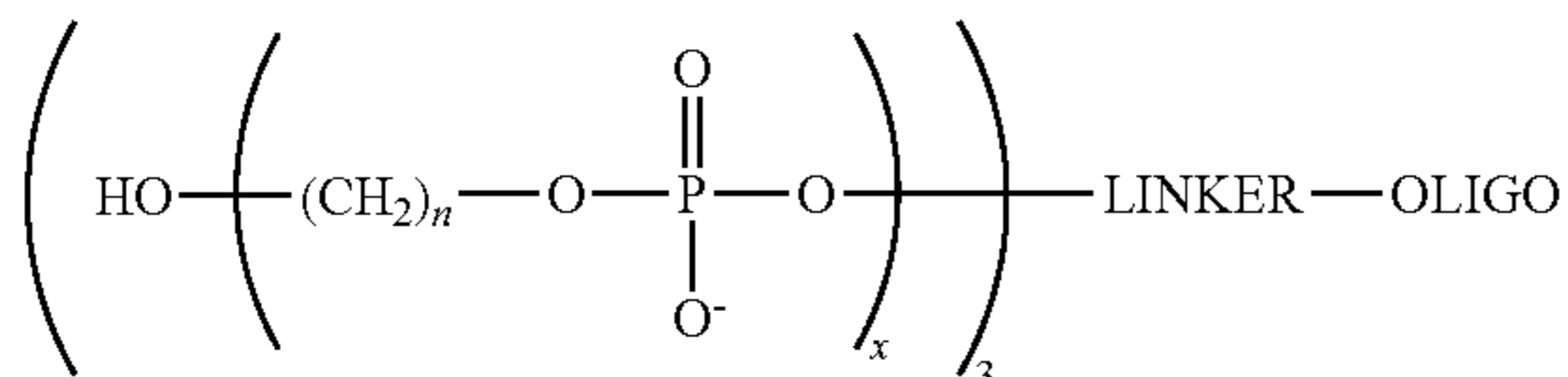
Formula VI
