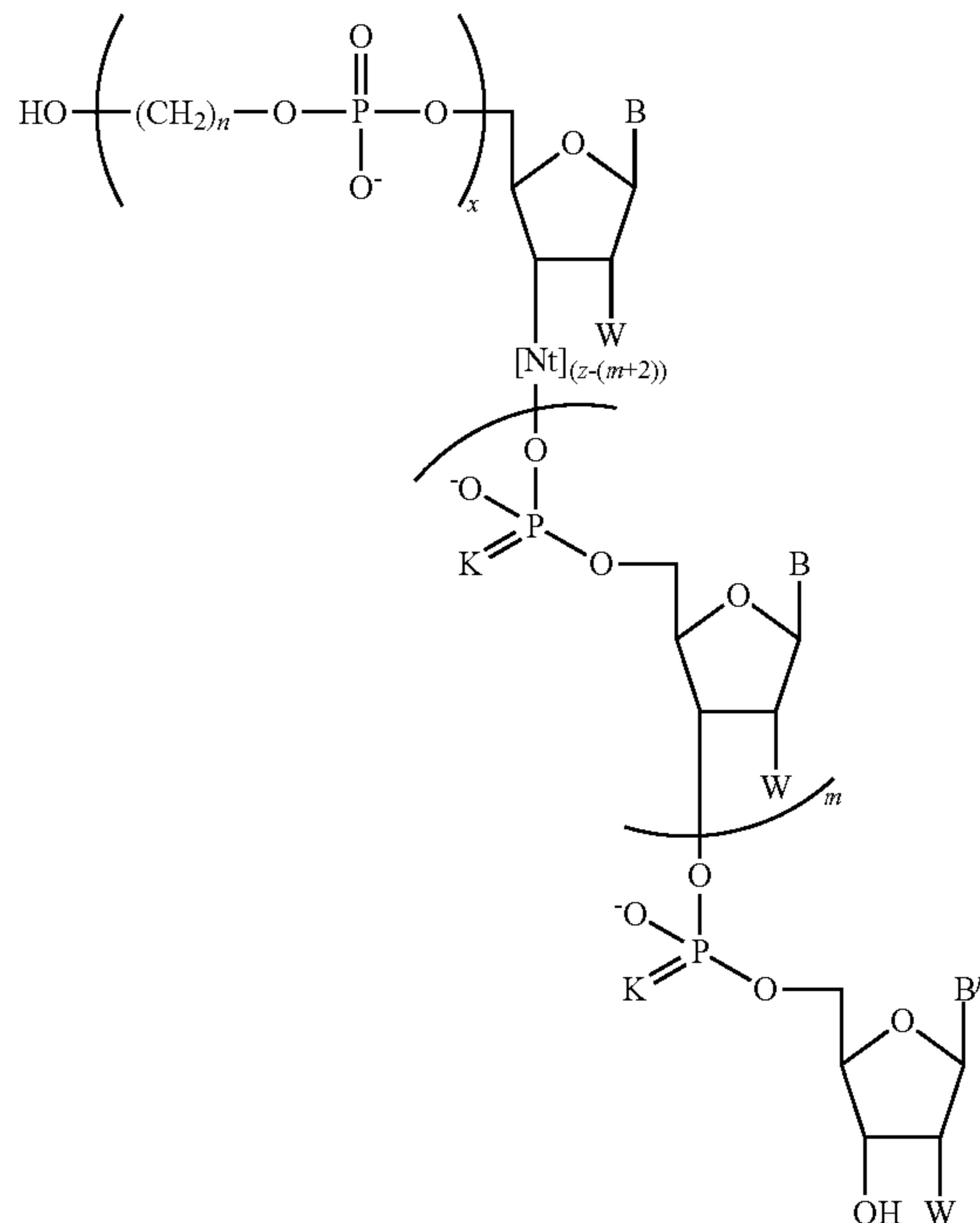
Formula I-B
