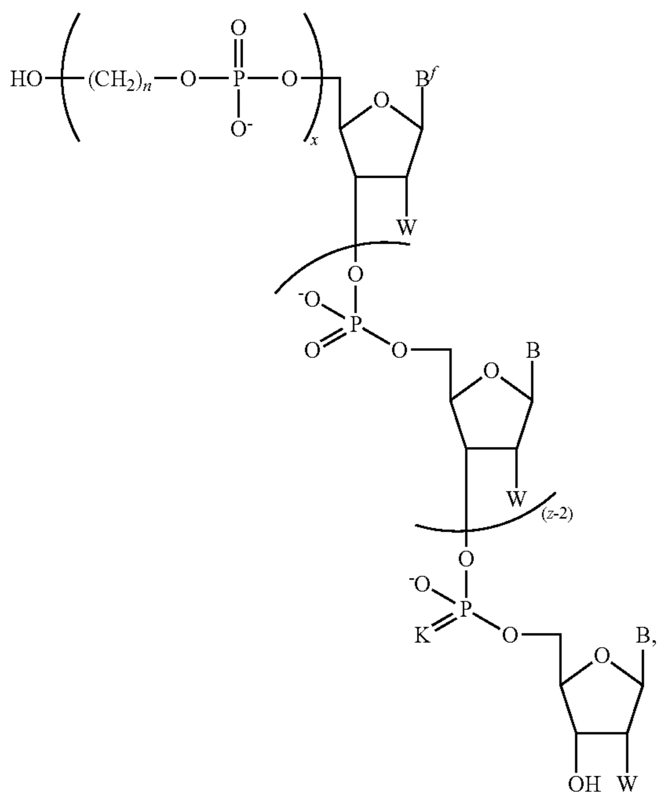
Formula I-E
