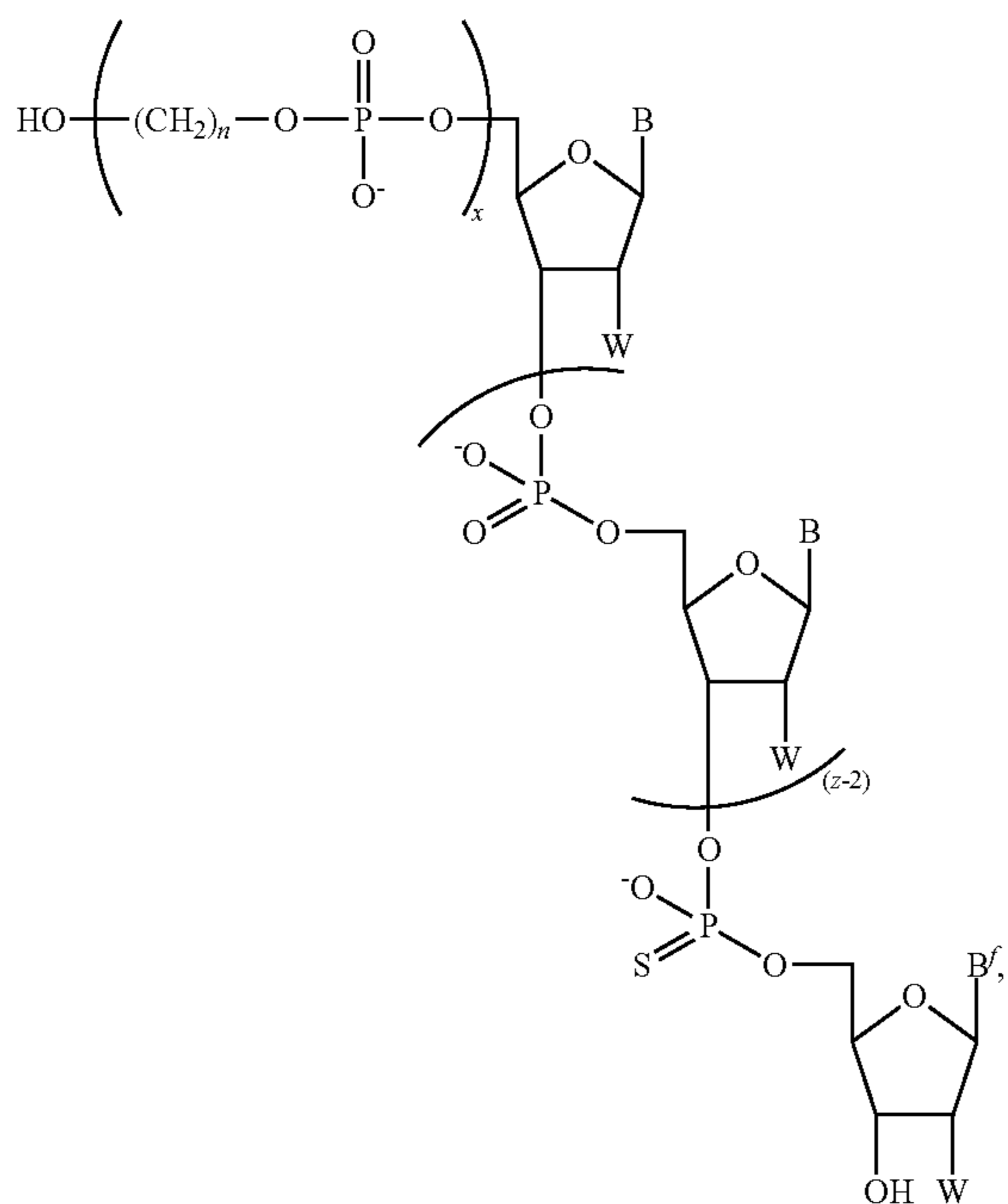
Formula I-H
