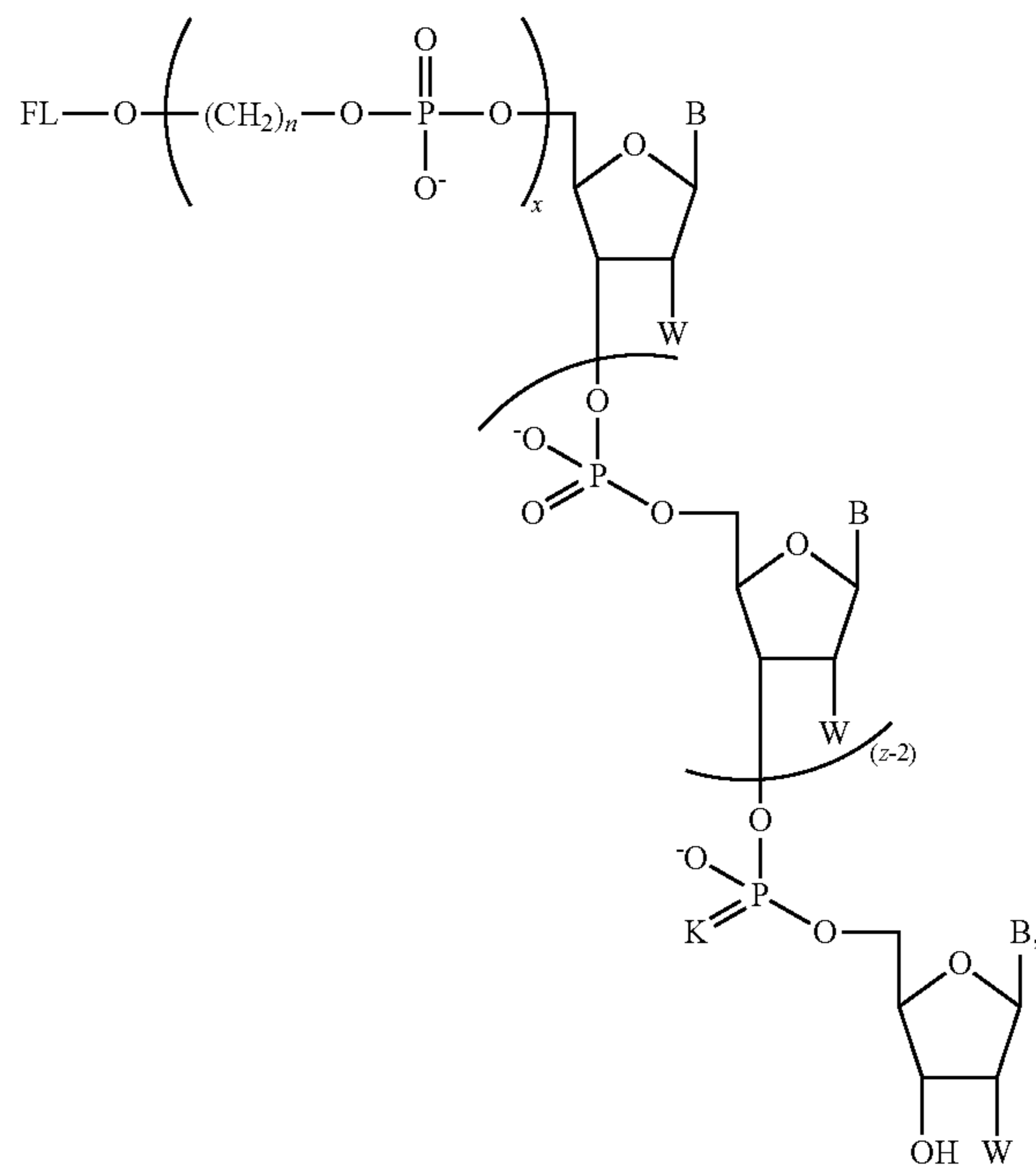
Formula I-G
