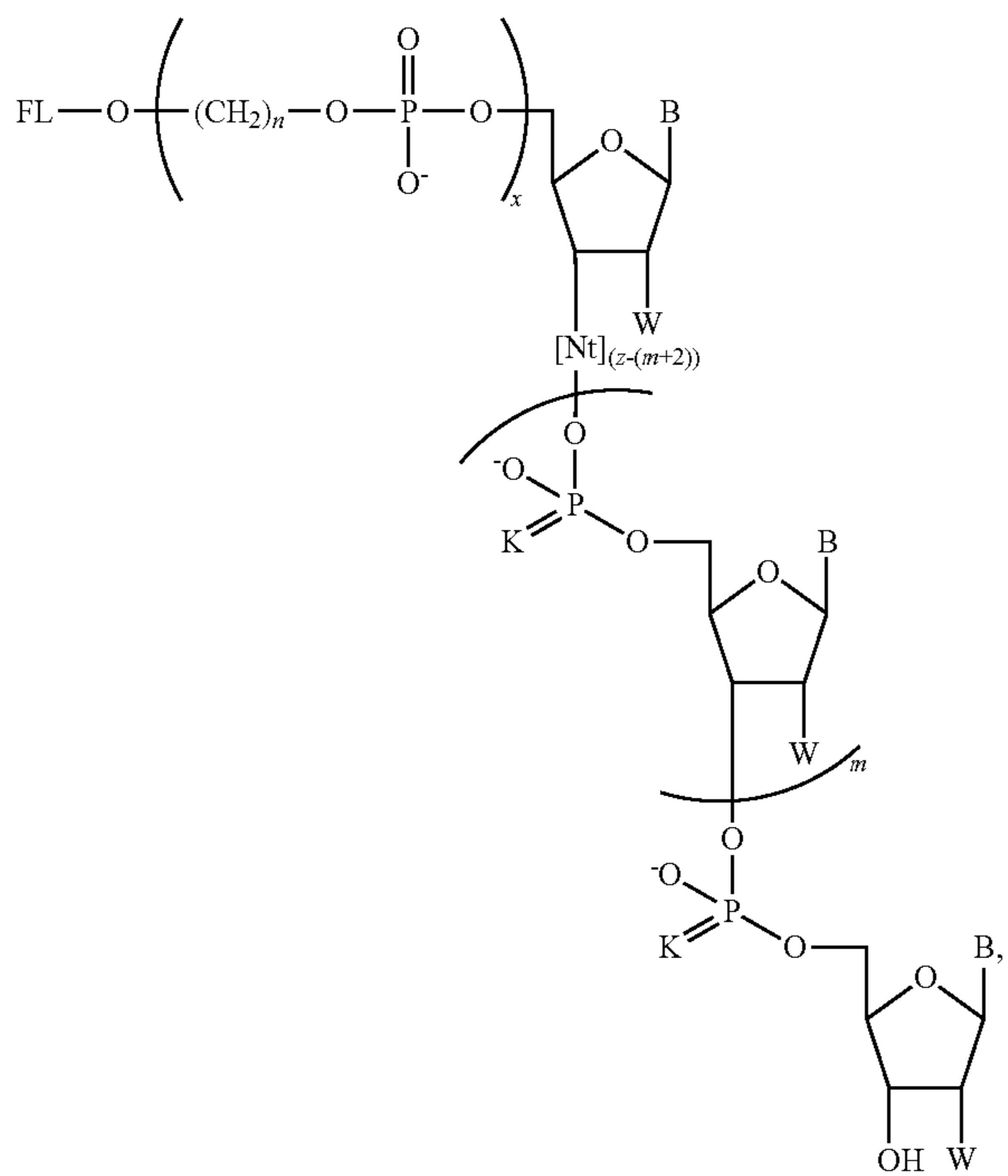
Formula I-D
