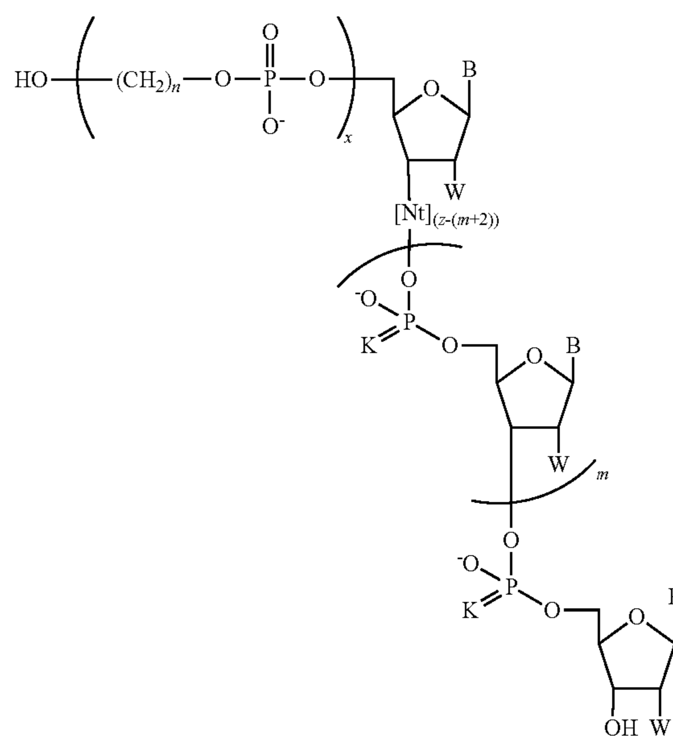
Formula I
