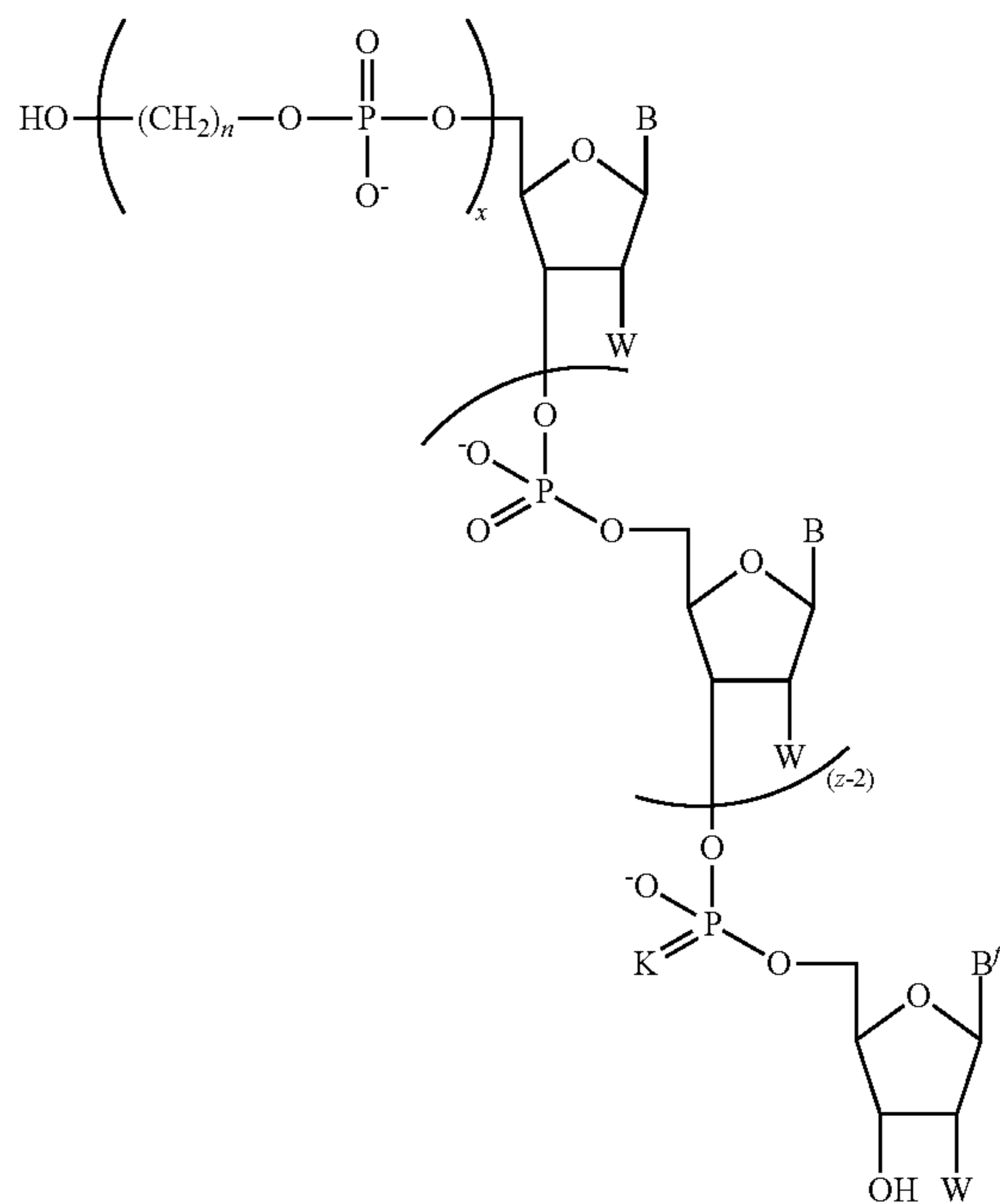
Formula I-F
