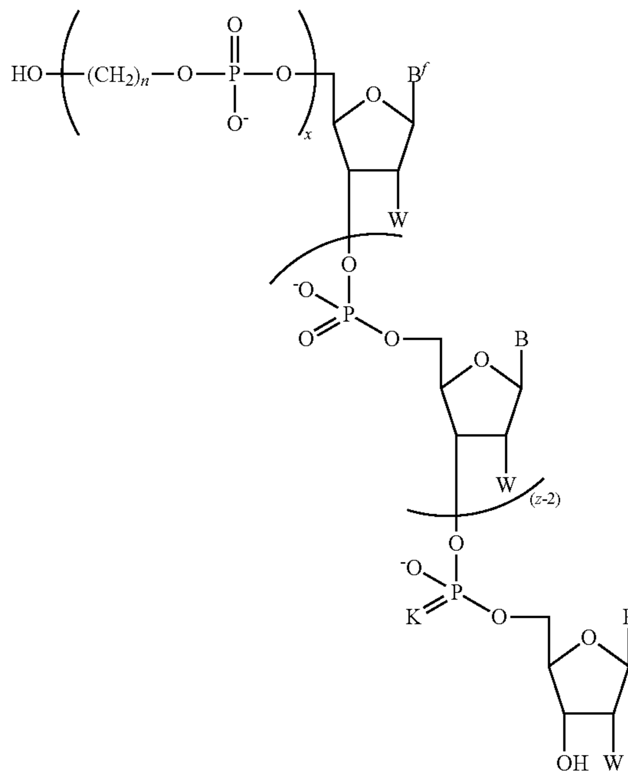
Formula I-E
