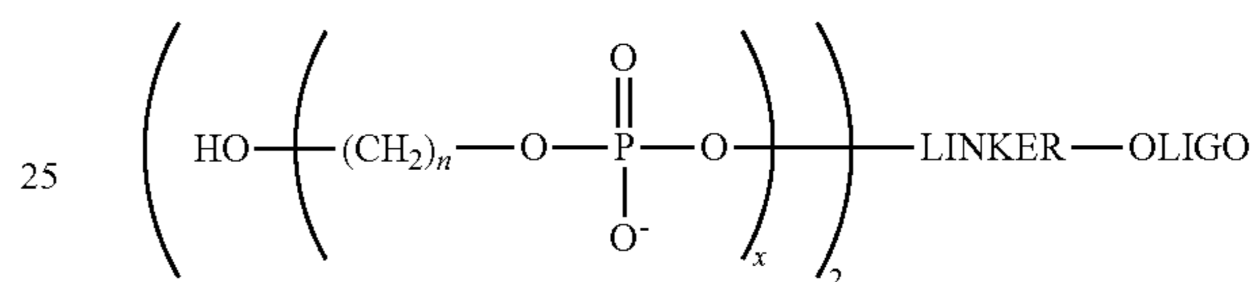
Formula V
