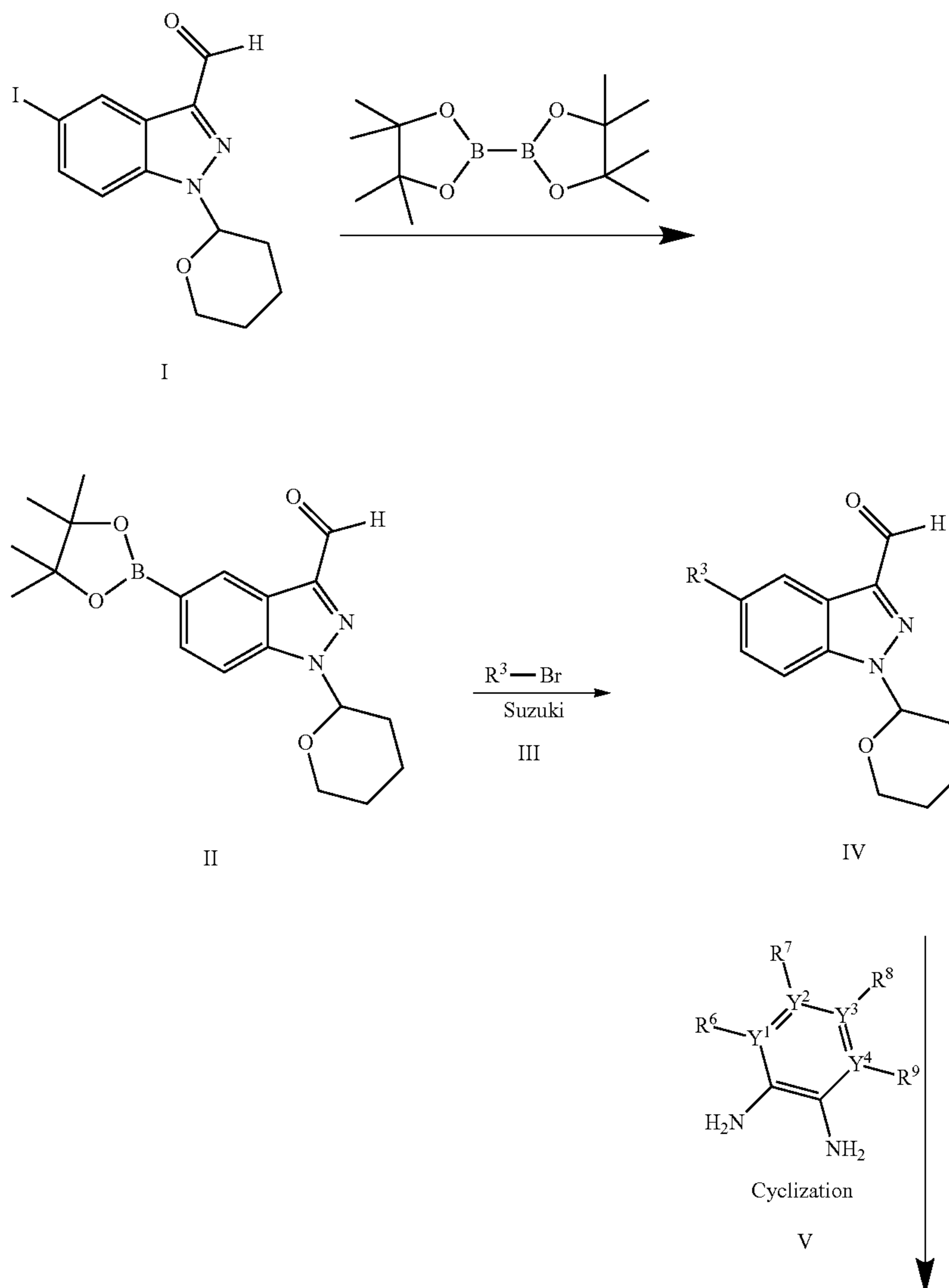
Scheme 1
