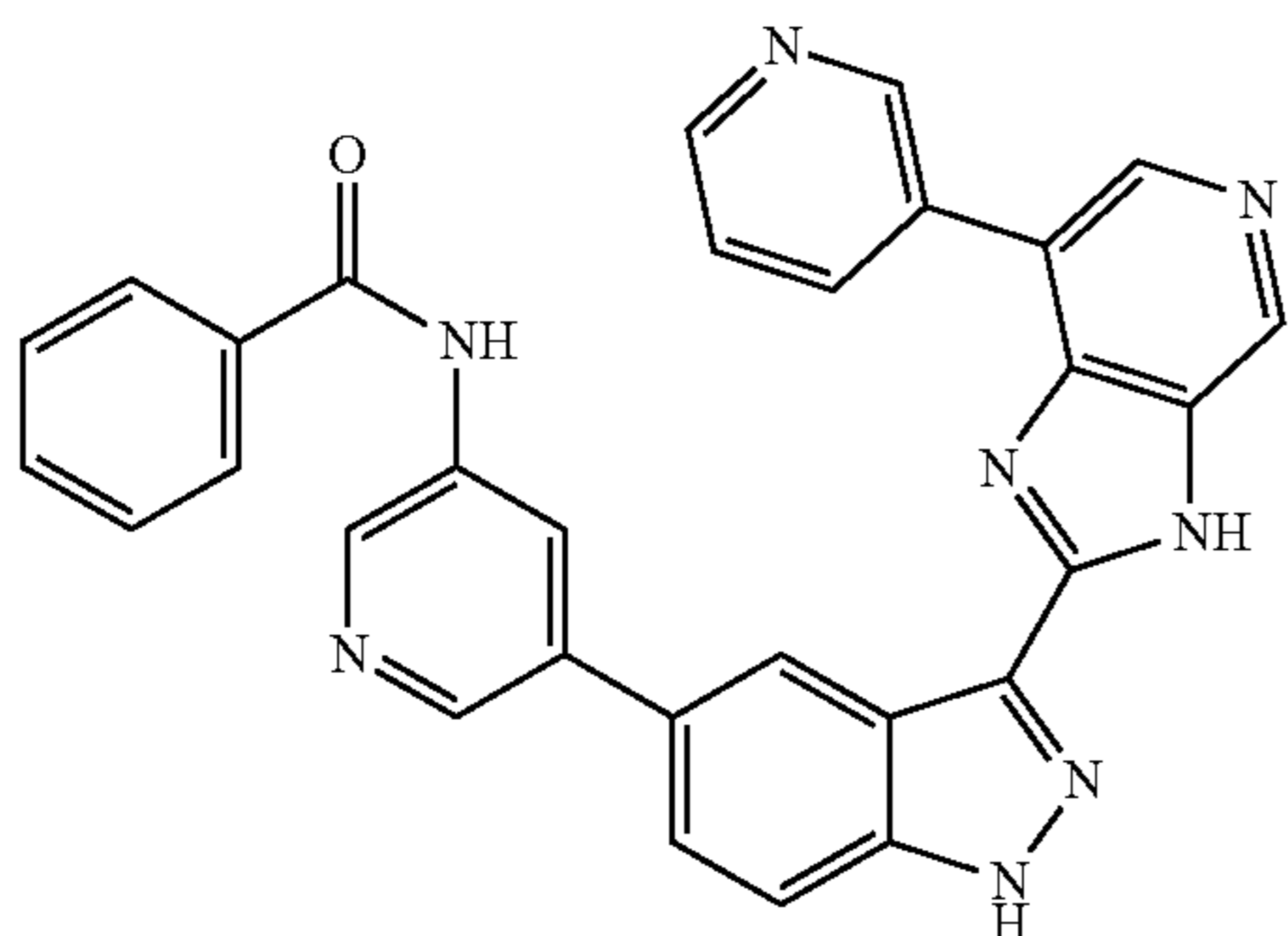
N-(5-(3-(7-(pyridin-3-yl)-3H-imidazo[4,5-c]pyridin-2-yl)-1H-indazol-5-yl)pyridin-3-yl)benzamide 16
