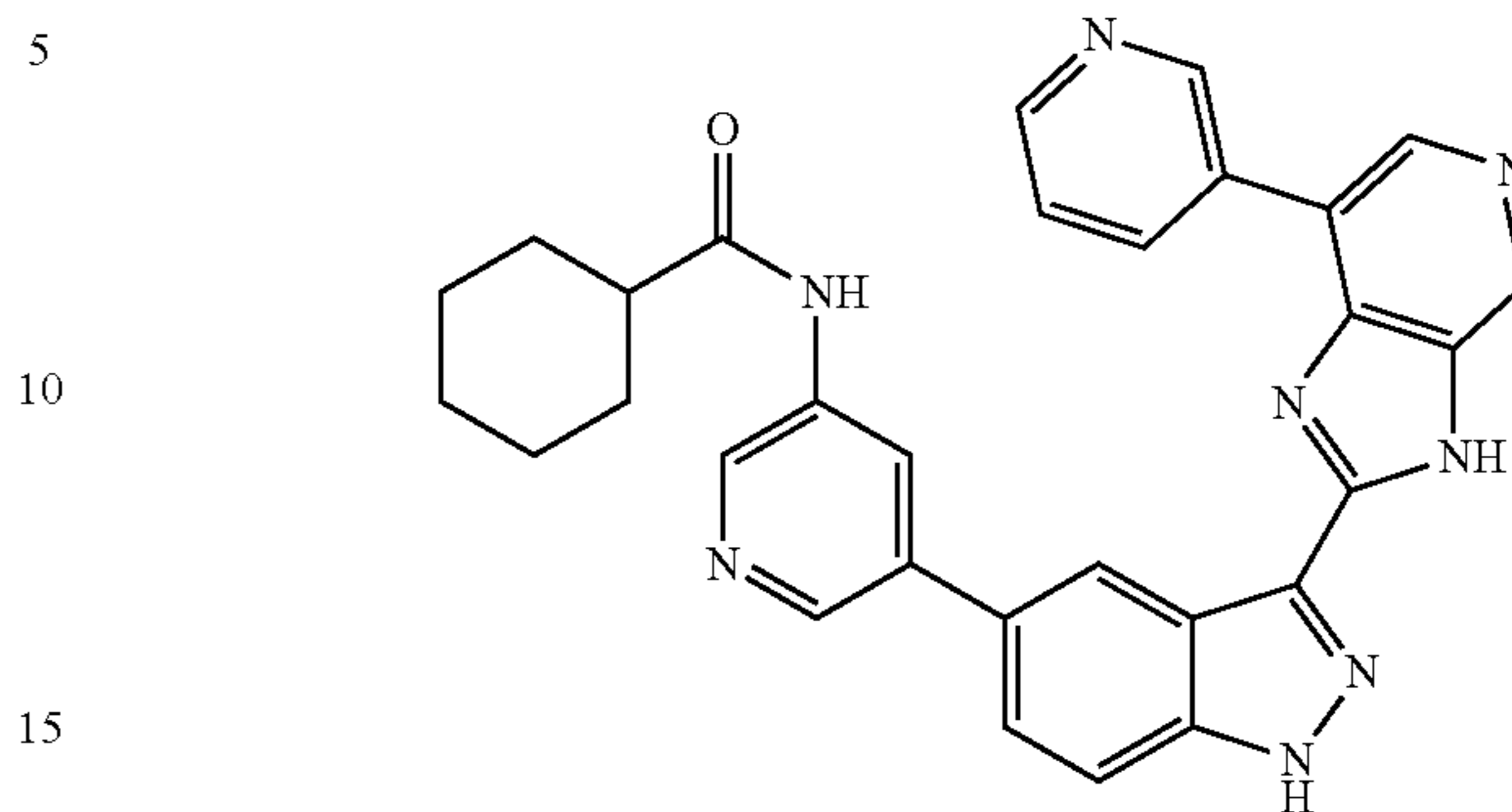
N-(5-(3-(7-(pyridin-3-yl)-3H-imidazo[4,5-c]pyridin-2-yl)-1H-indazol-5-yl)pyridin-3-yl)cyclohexanecarboxamide 19
