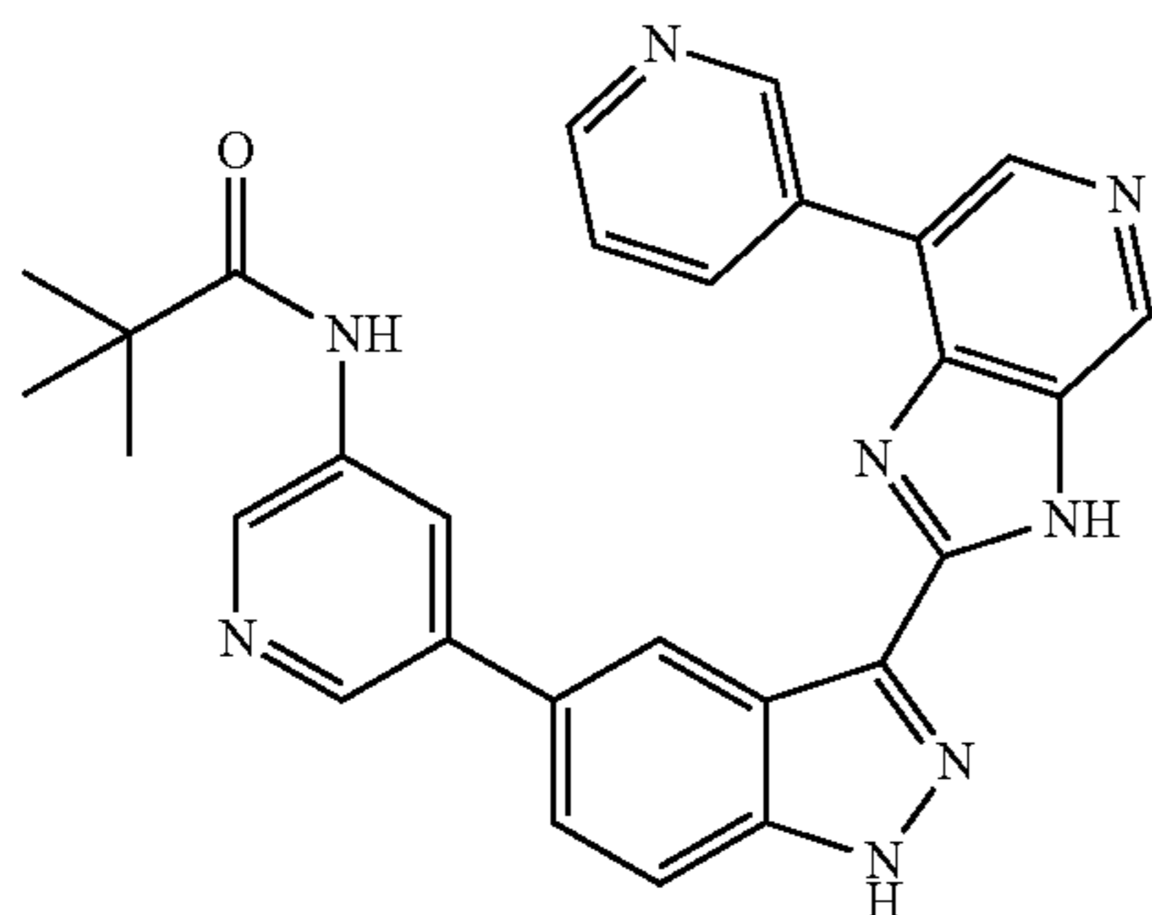
N-(5-(3-(7-(pyridin-3-yl)-3H-imidazo[4,5-c]pyridin-2-yl)-1H-indazol-5-yl)pyridin-3-yl)pivalamide 17
