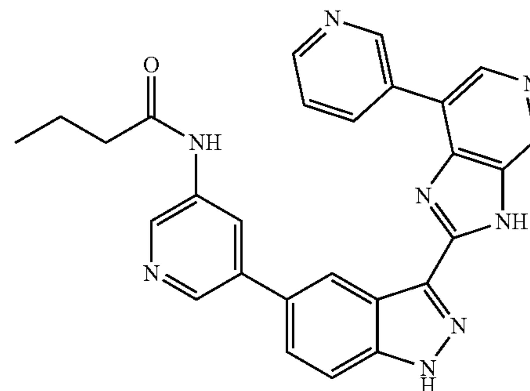
N-(5-(3-(7-(pyridin-3-yl)-3H-imidazo[4,5-c]pyridin-2-yl)-1H-indazol-5-yl)pyridin-3-yl)butyramide 20
