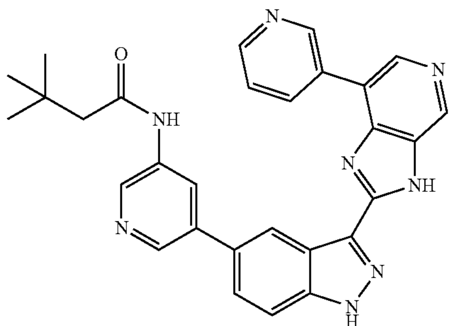
3,3-dimethyl-N-(5-(3-(7-(pyridin-3-yl)-3H-imidazo[4,5-c]pyridin-2-yl)-1H-indazol-5-yl)pyridin-3-yl)butanamide 18
