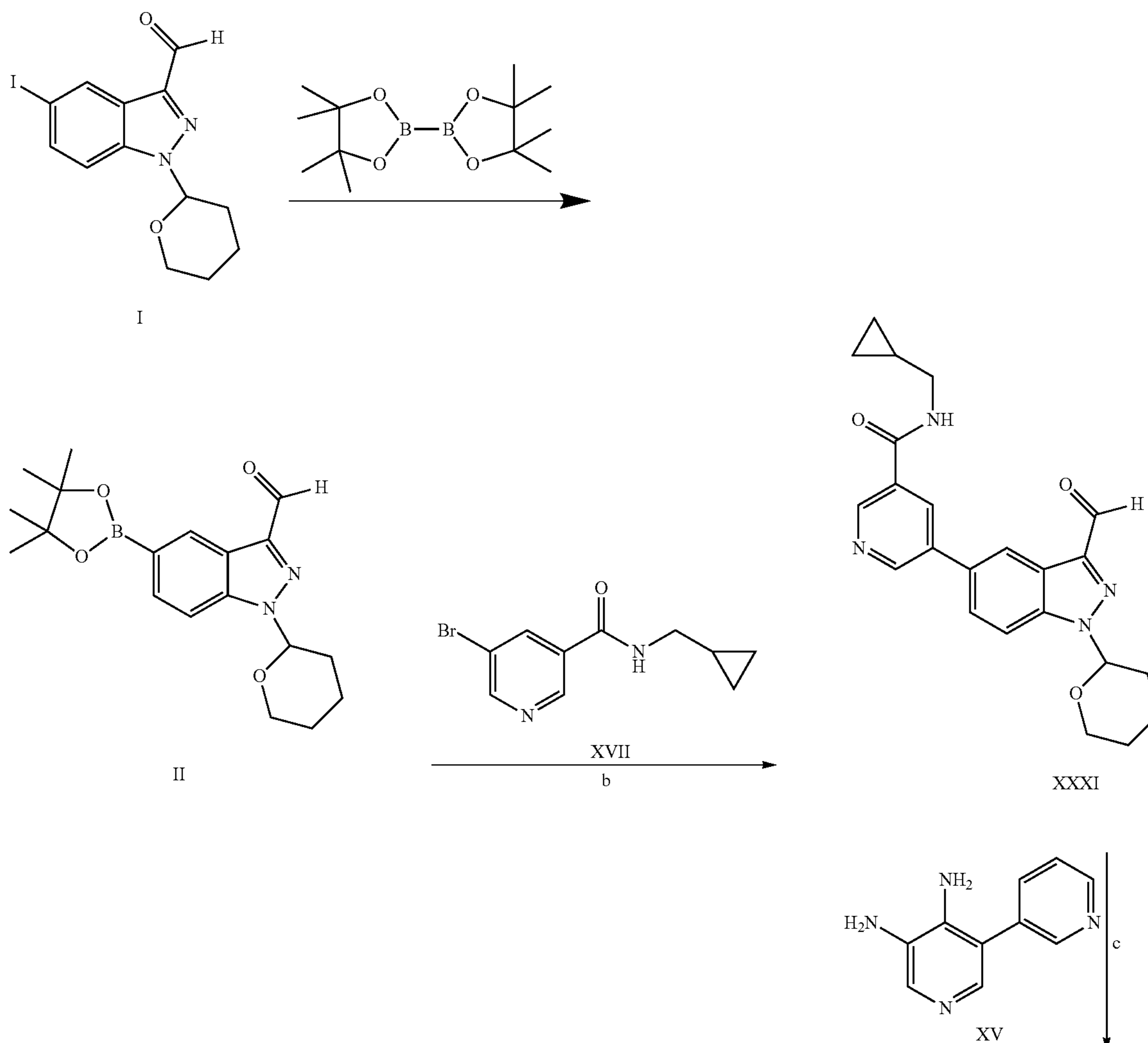
Scheme 6
