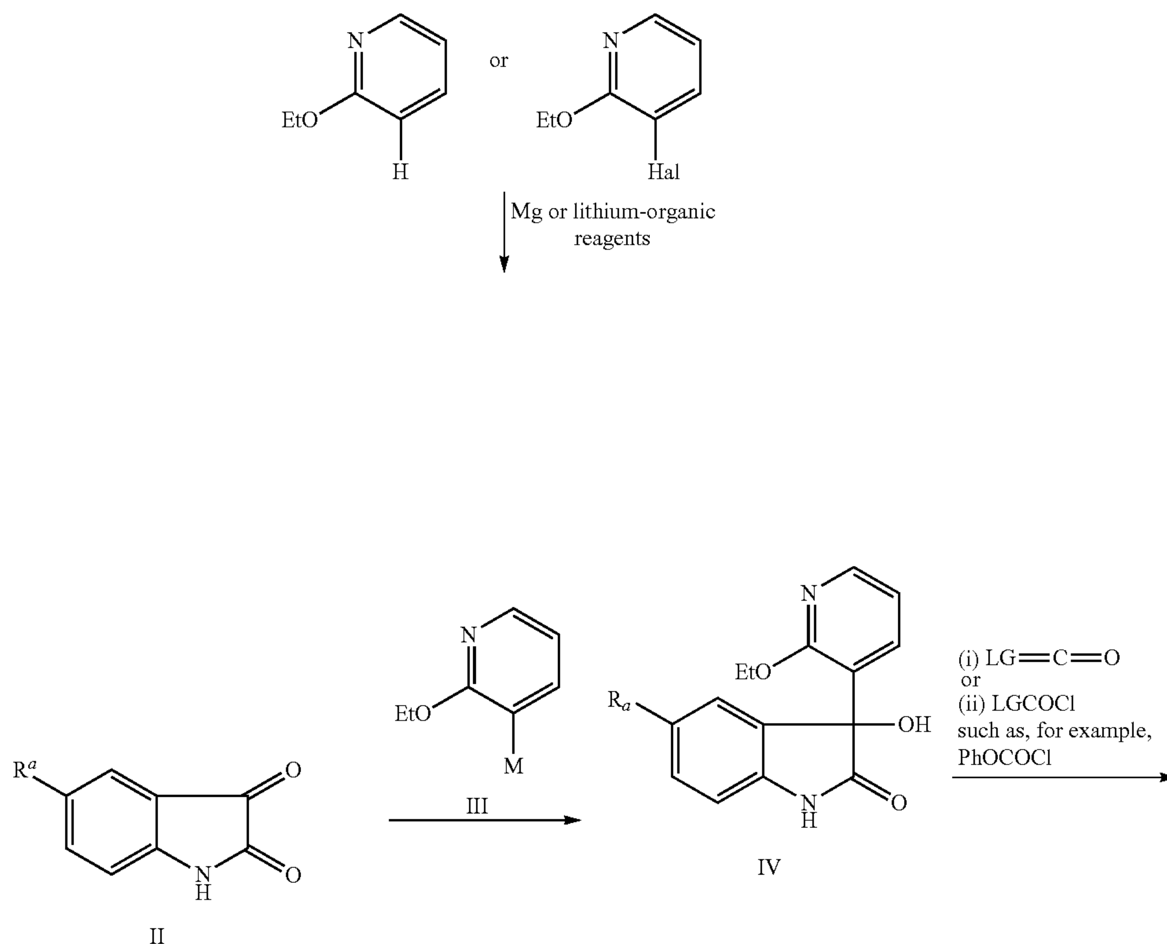
SYNTHESIS SCHEME 1
