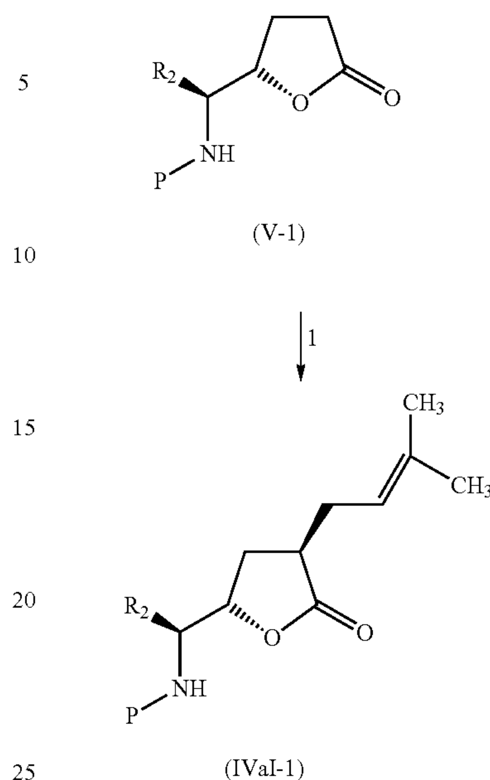
Scheme 3
