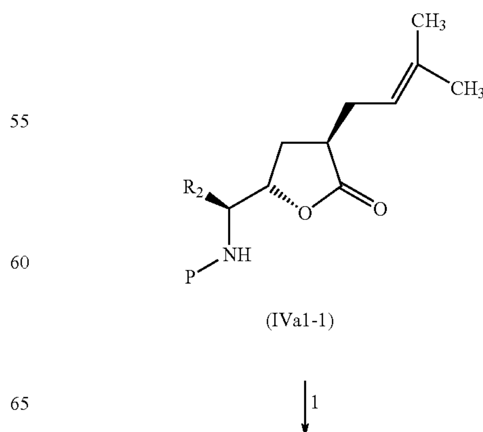
Scheme 4
