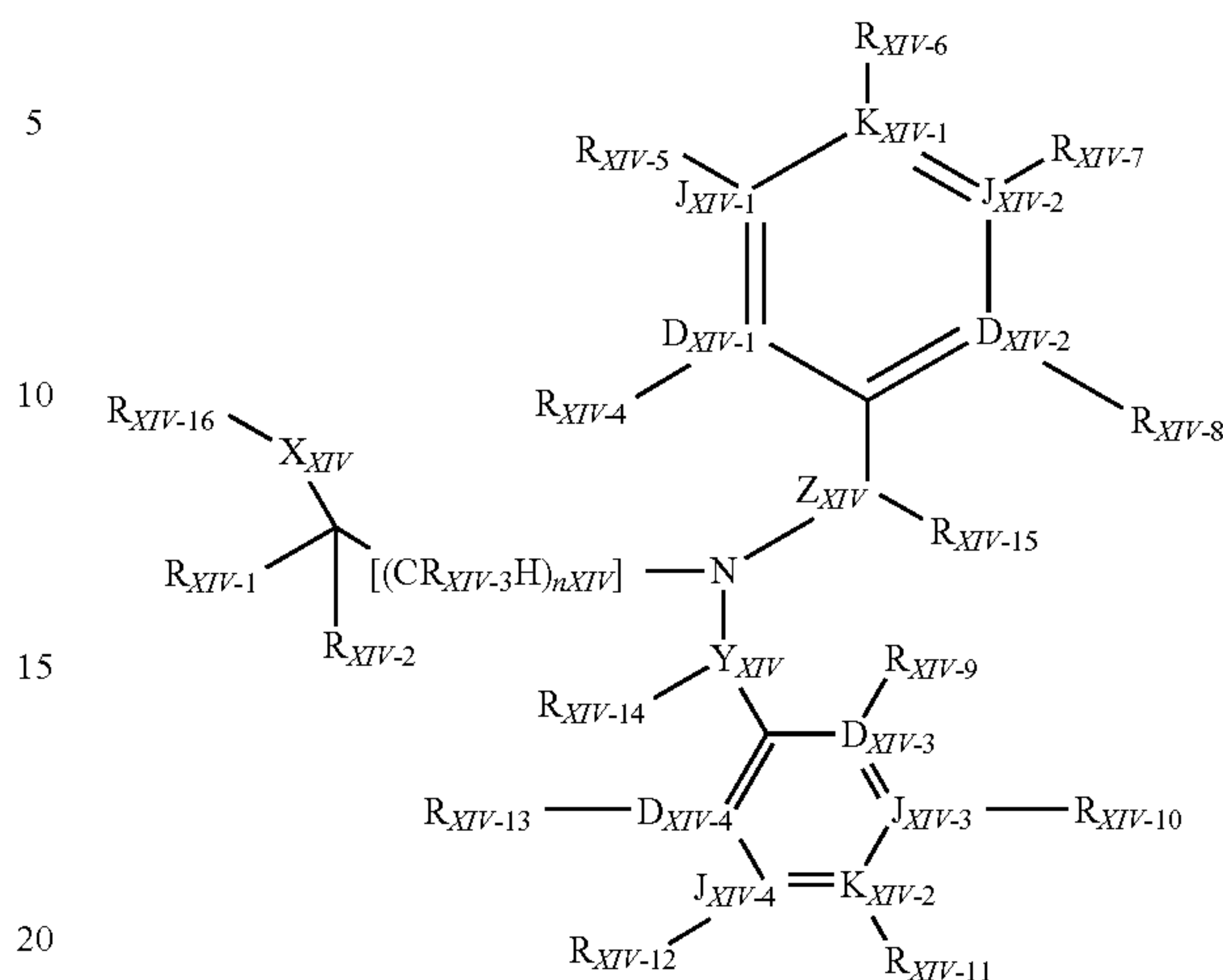
Formula XIV
