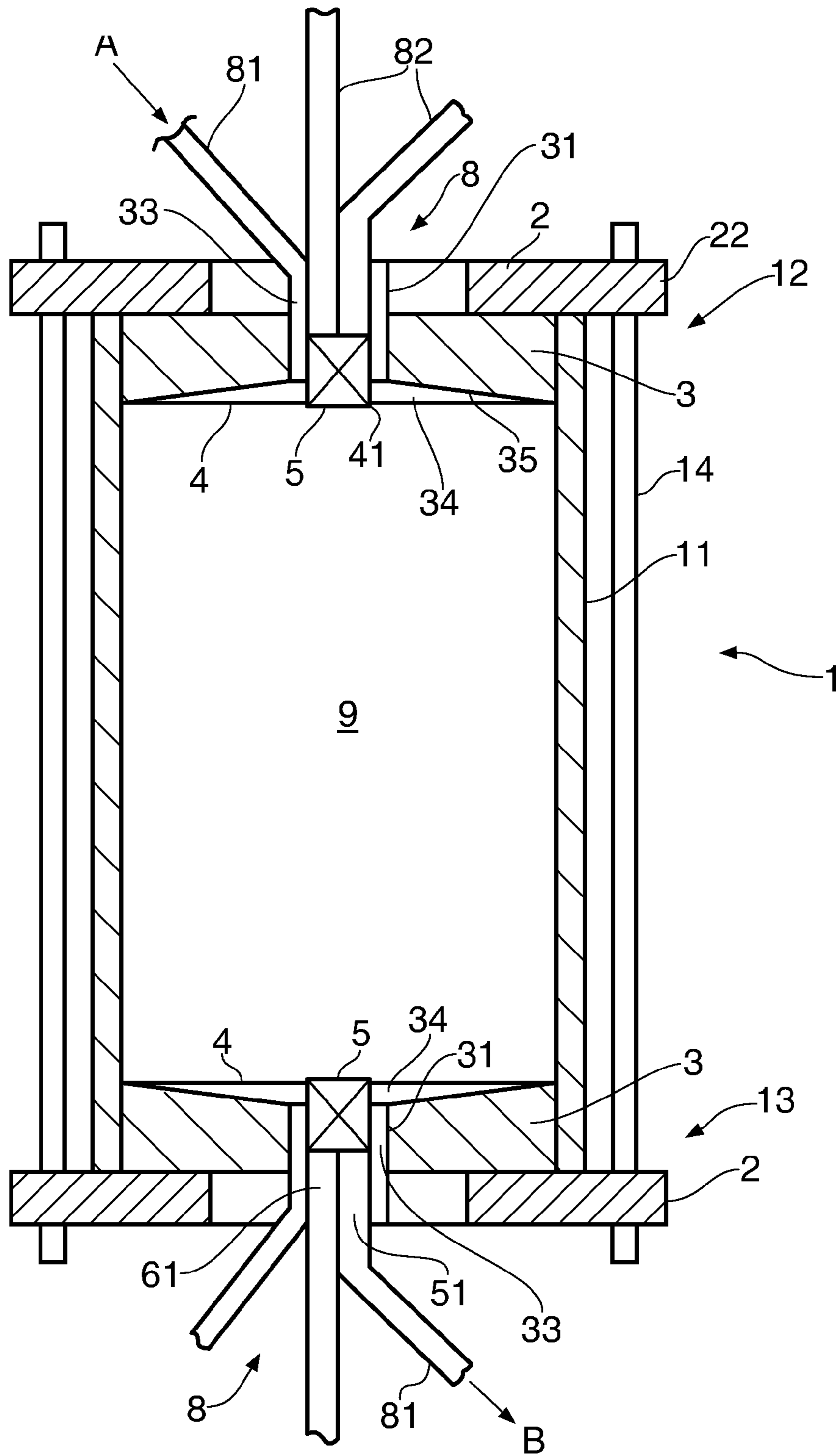
Fig. 1 Prior Art
