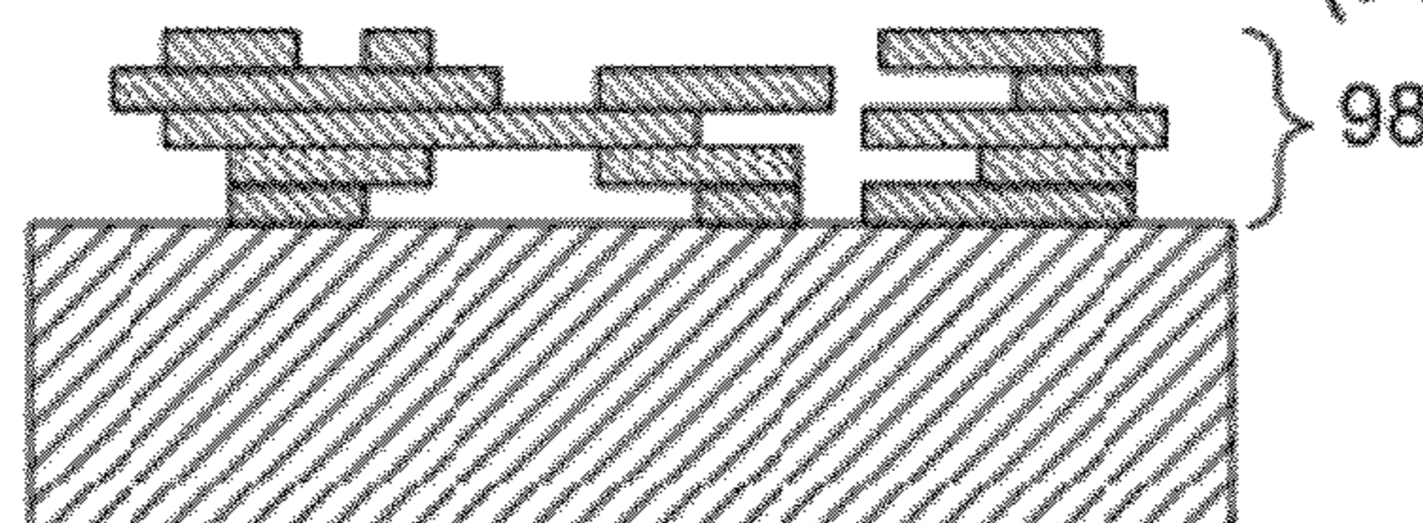
FIG. 4I (PRIOR ART)
