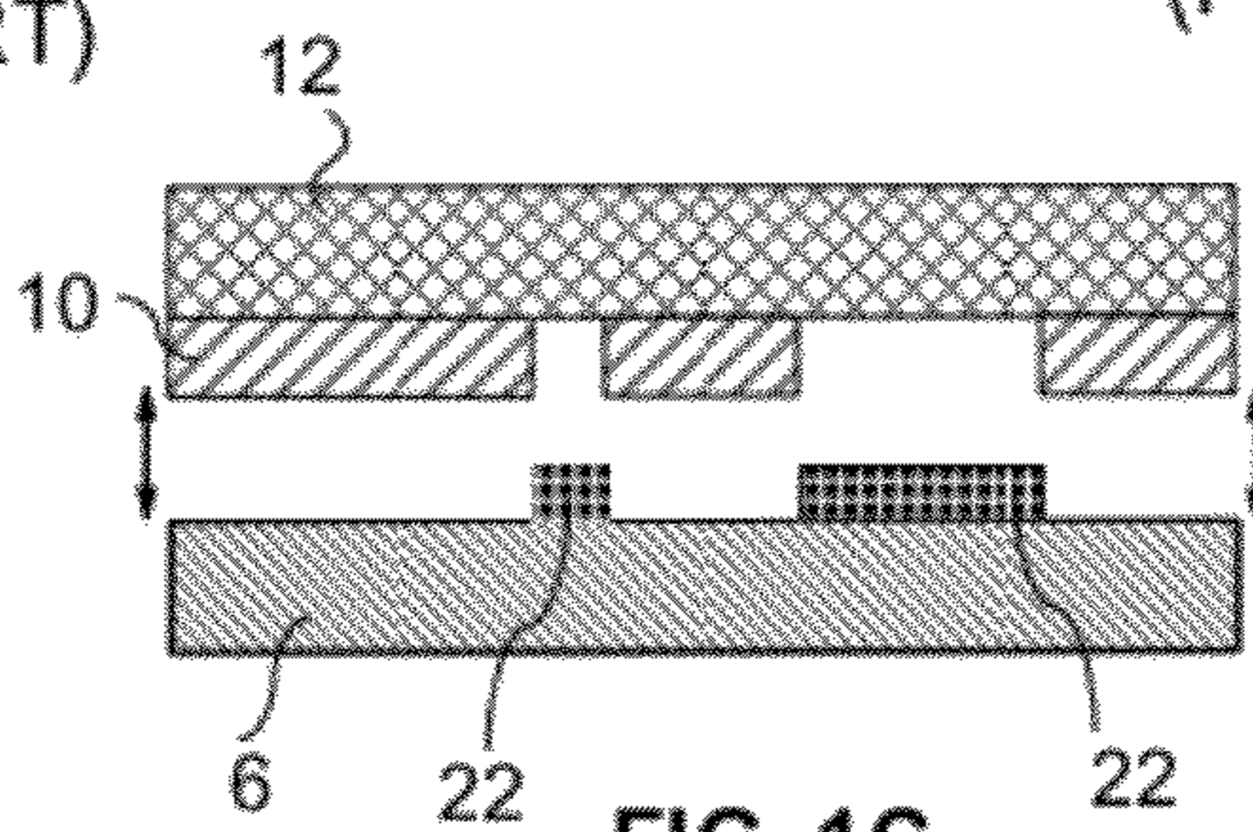
FIG. 1C (PRIOR ART)
