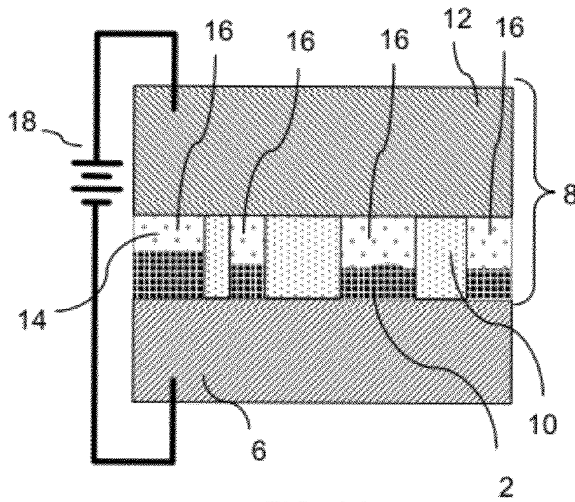
FIG. 2A (PRIOR ART) 4
