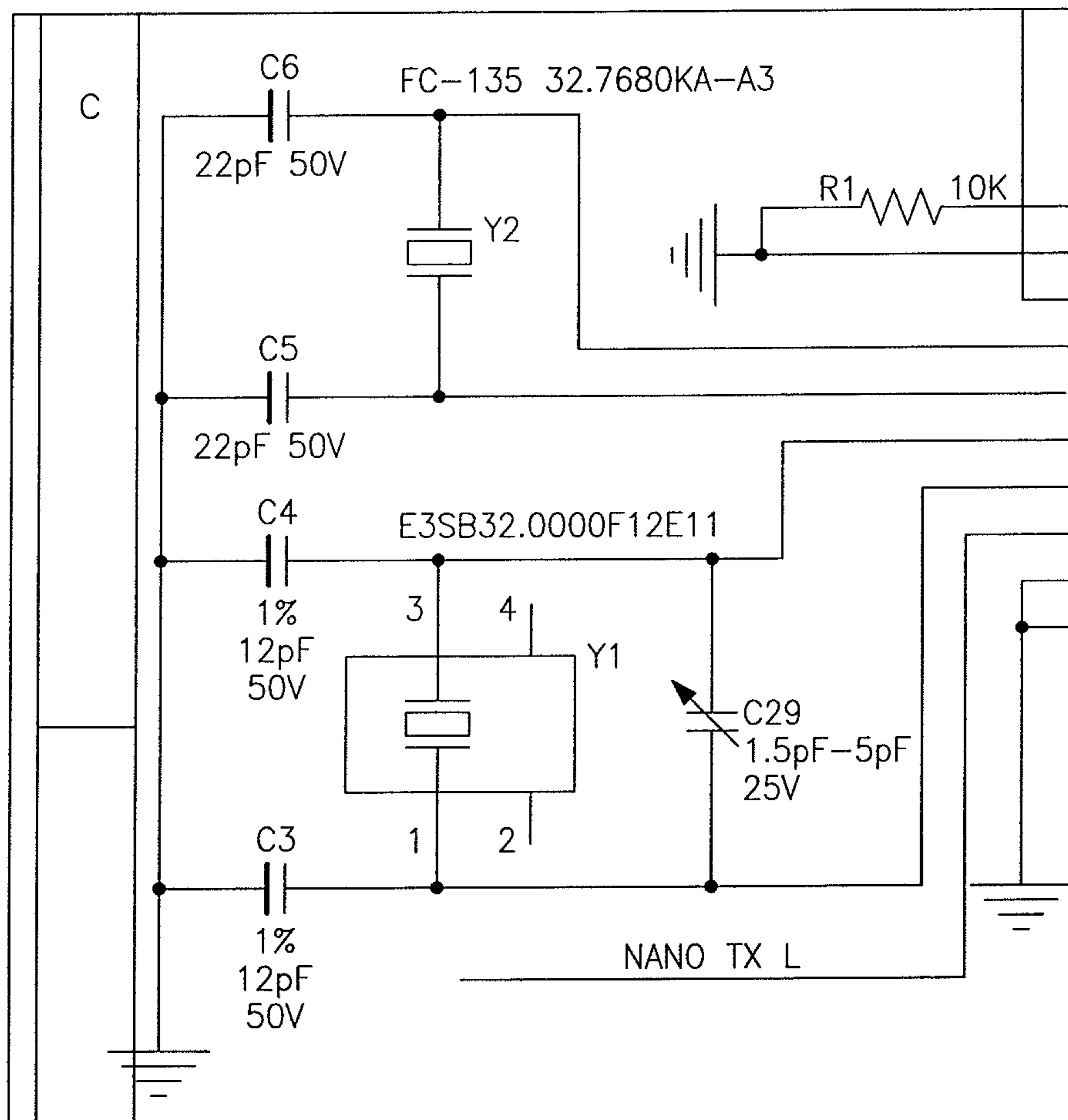
Trimmer Capacitor
