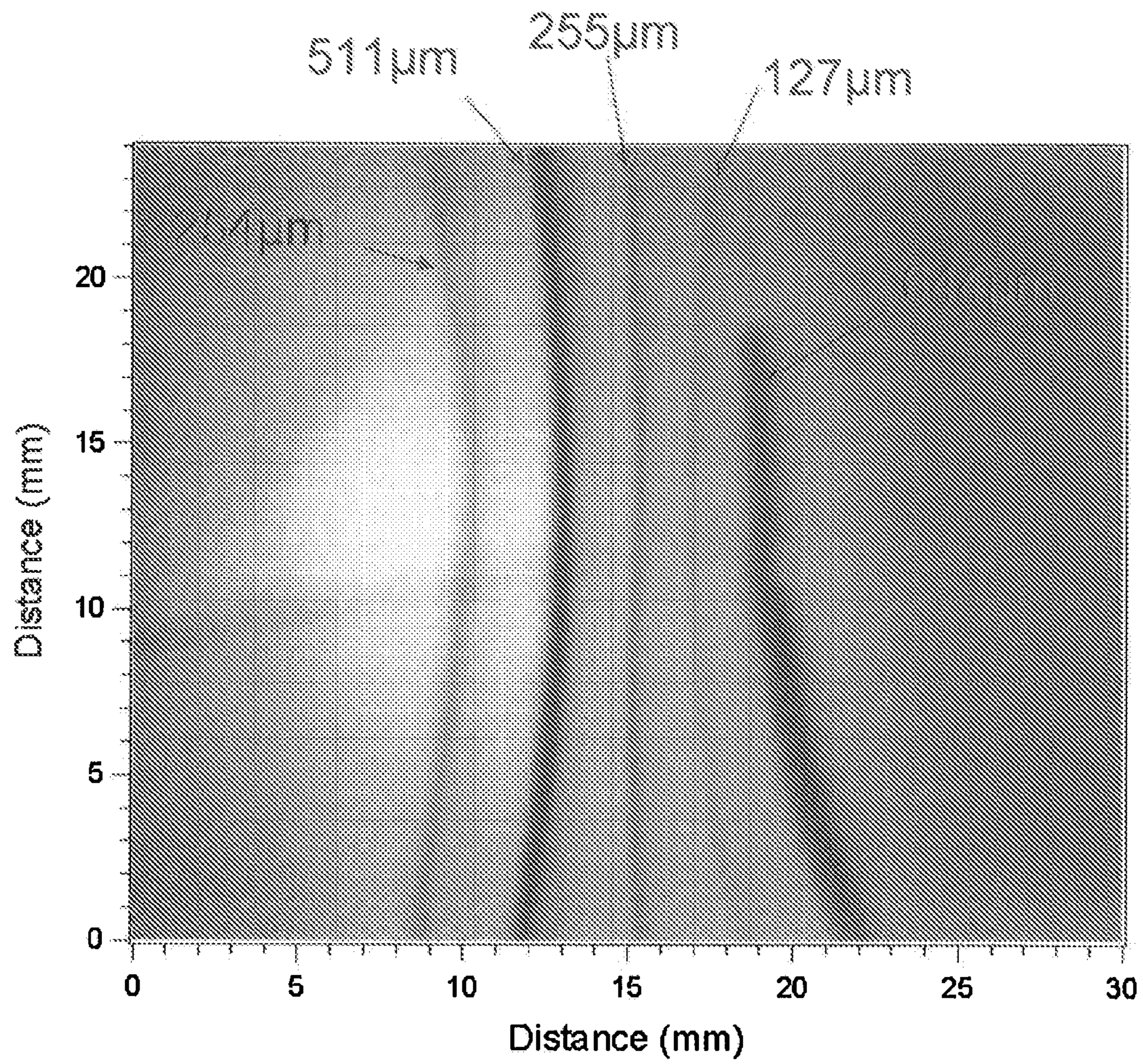
X-ray image of metal wires
