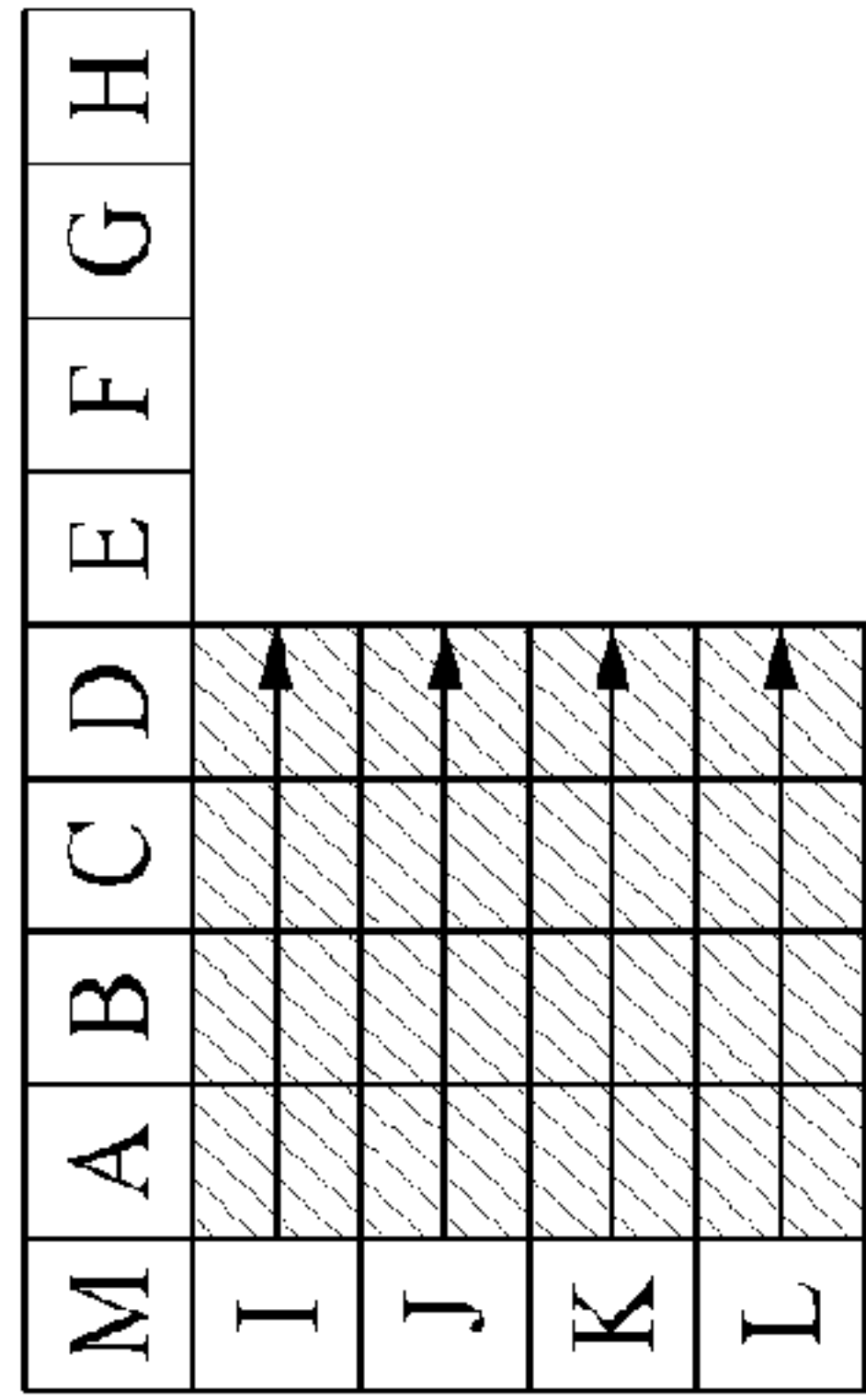
IMAGE PREDICTION MODE 1
