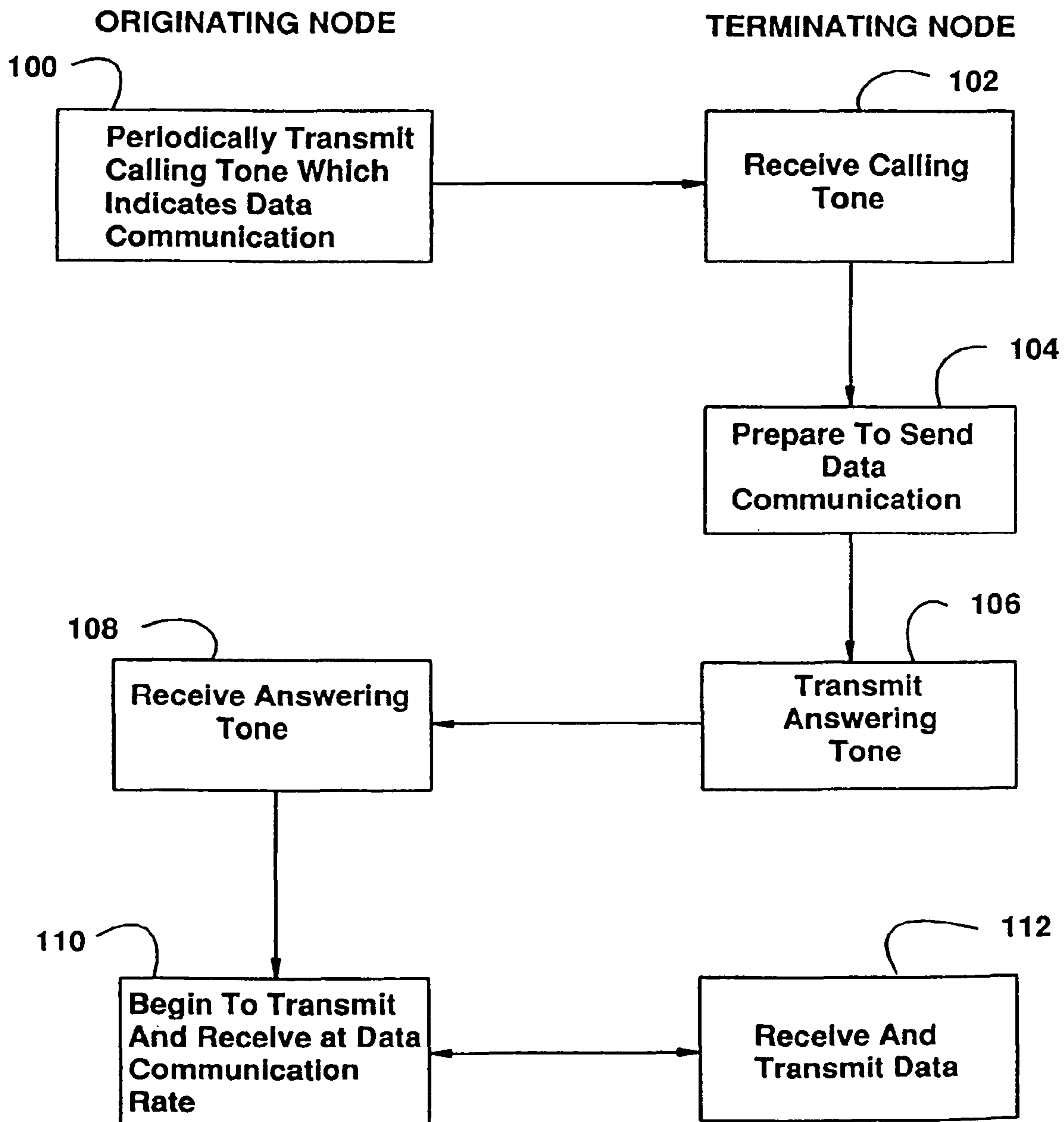
FIG.3 PRIOR ART
