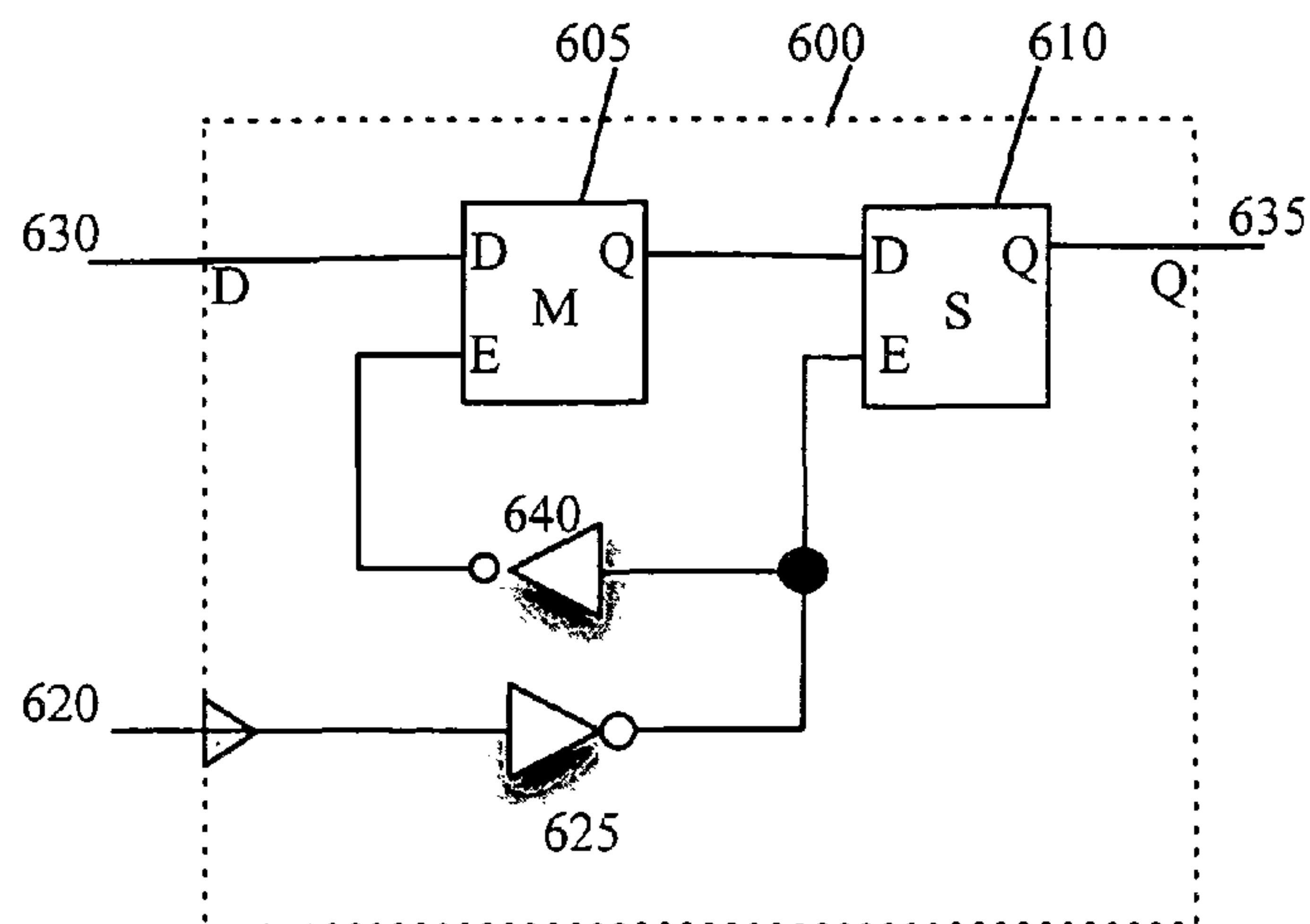
Figure 6 Prior Art
