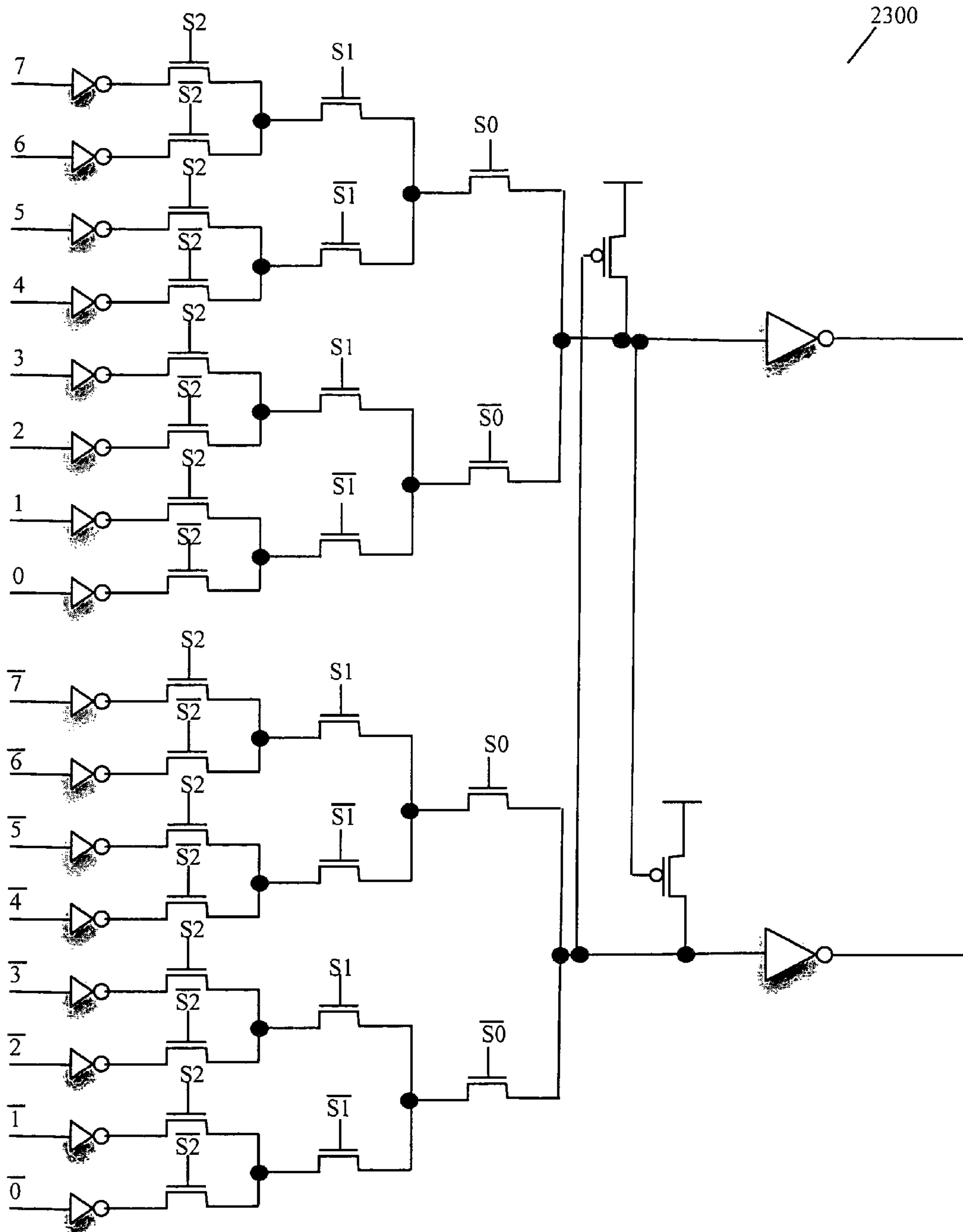
Figure 23 Prior Art
