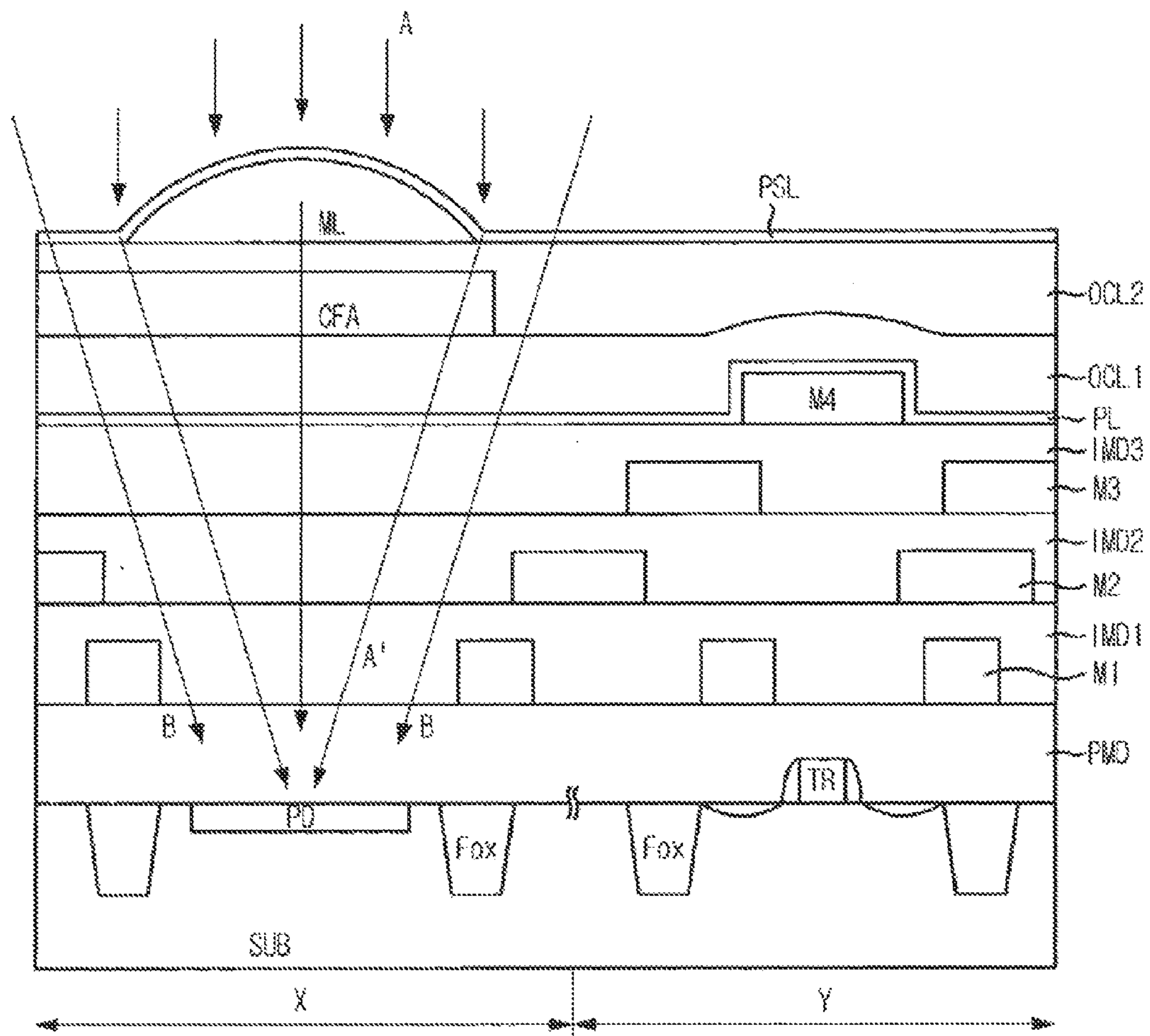
FIG. 2 (RELATED ART)
