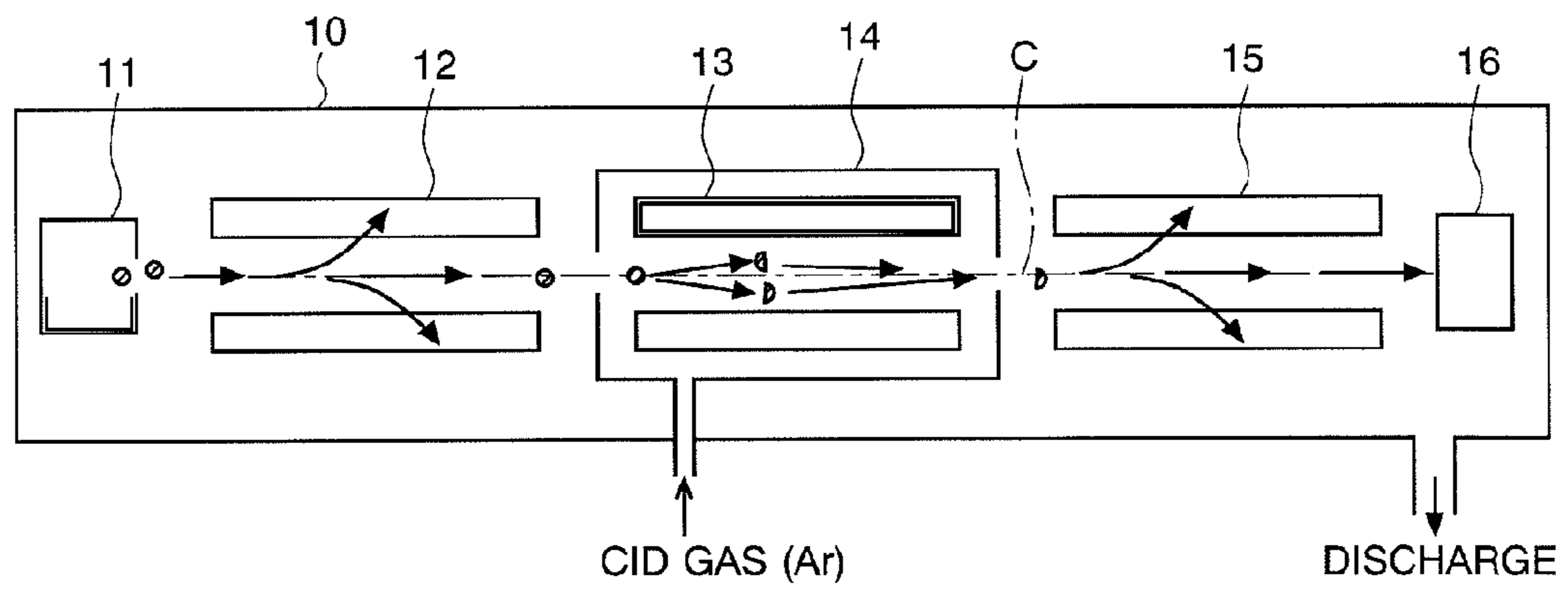
Fig. 14 (Prior Art)
