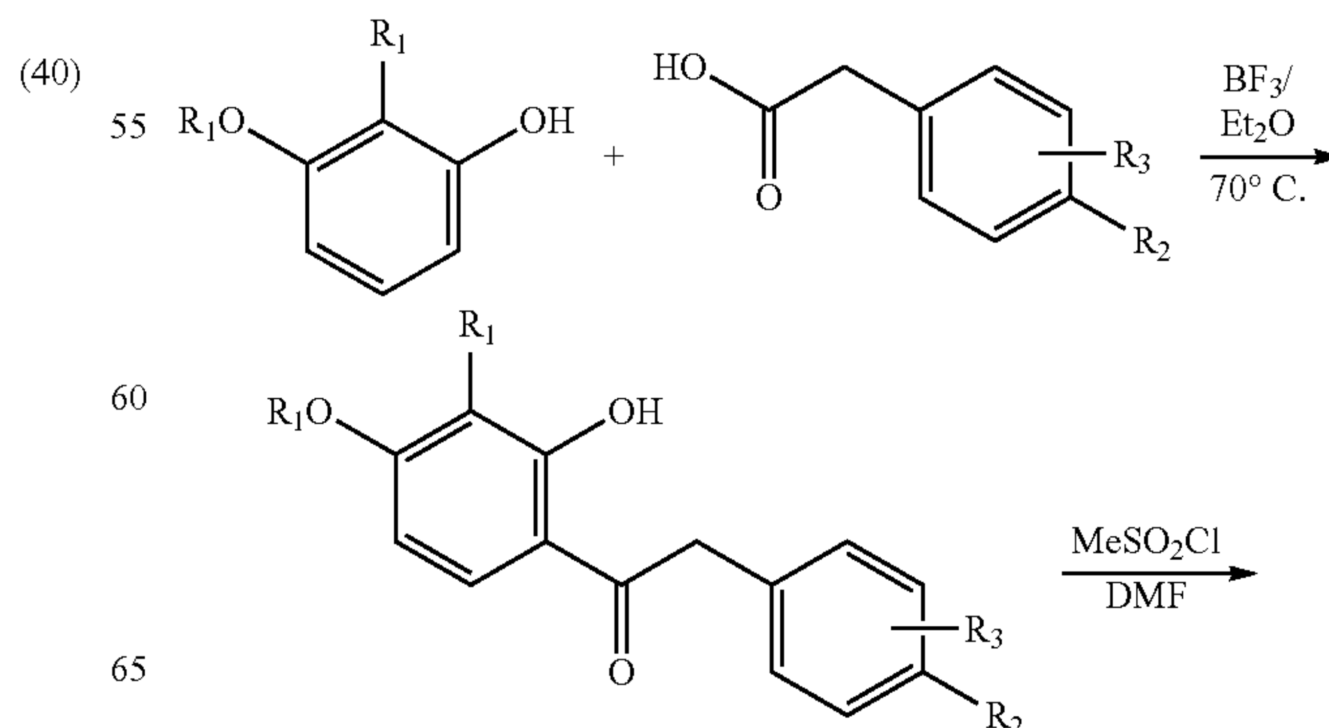
Scheme 1
