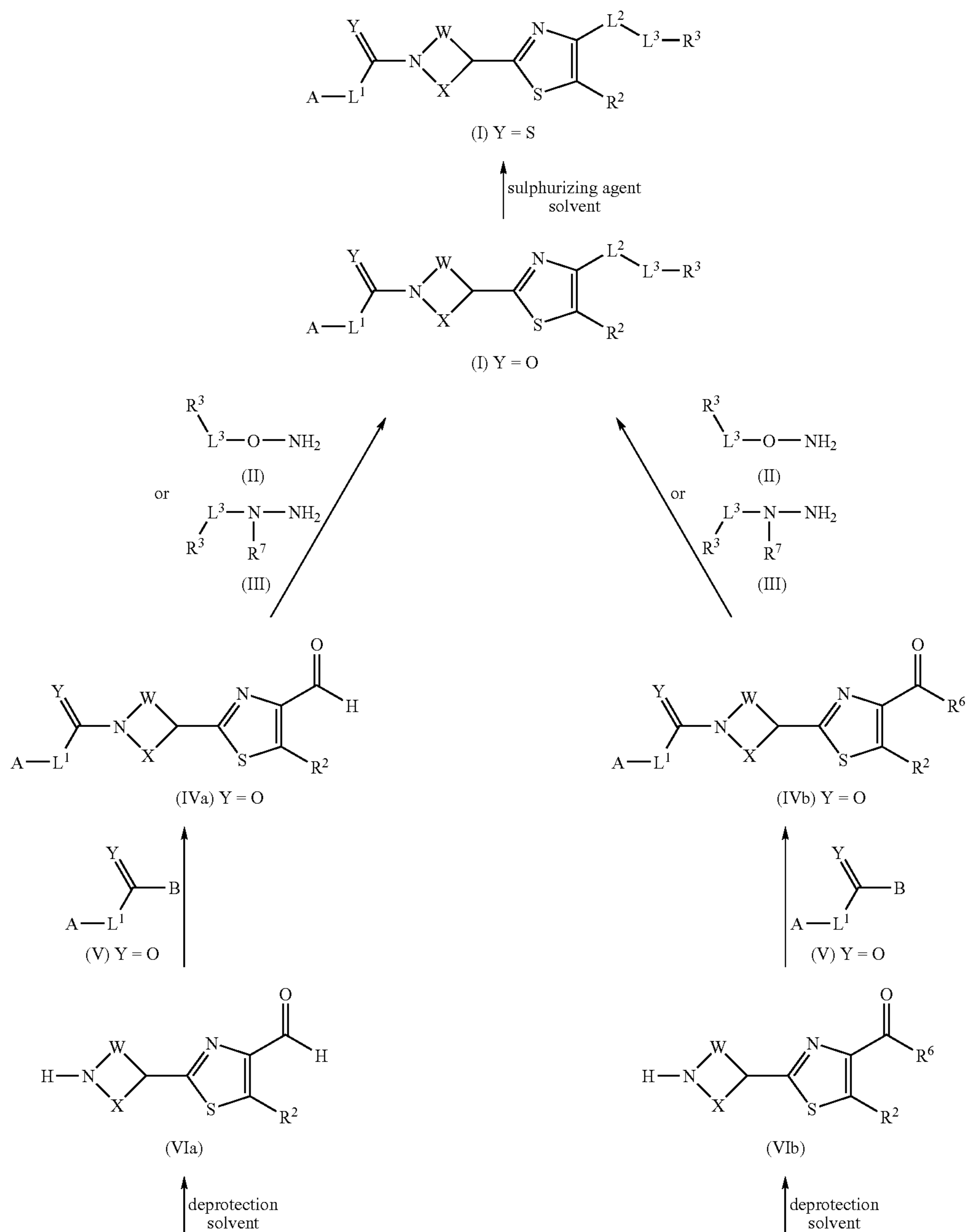
Scheme 8
