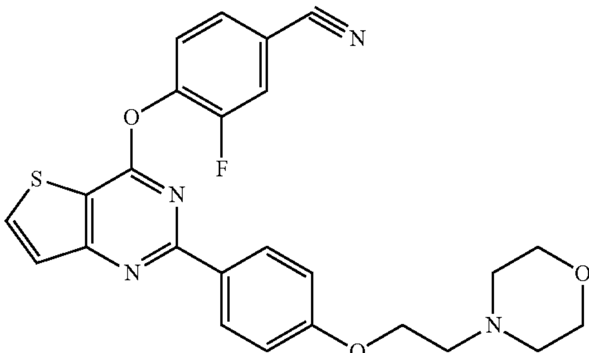
Compound 23
