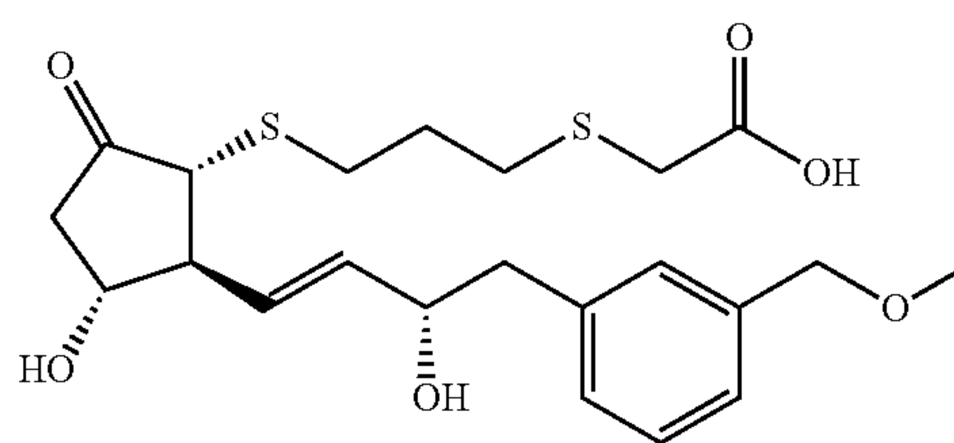
Compound 8
