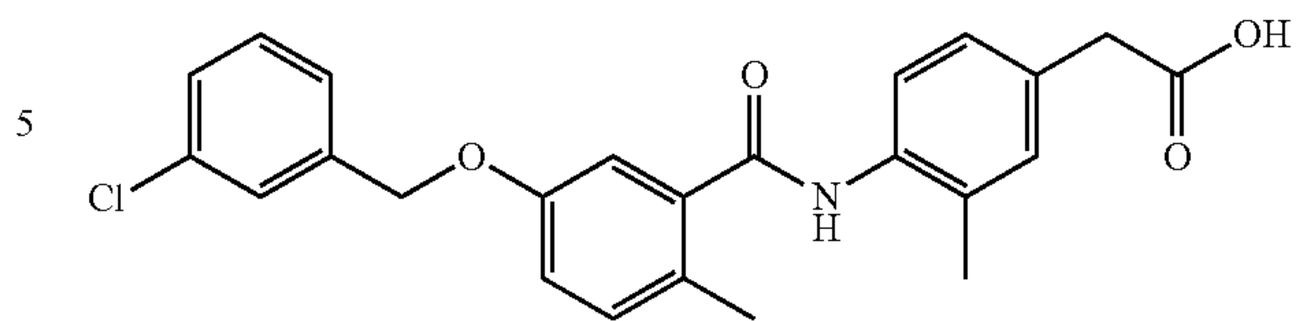
Compound 24
