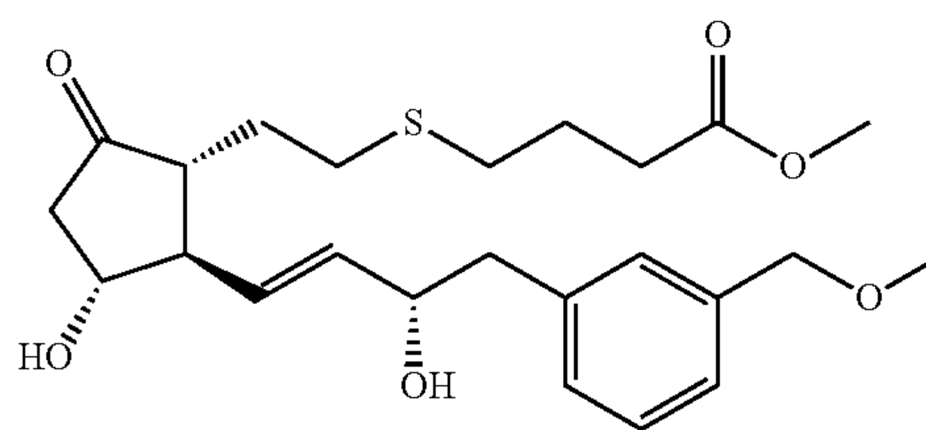
Compound 7
