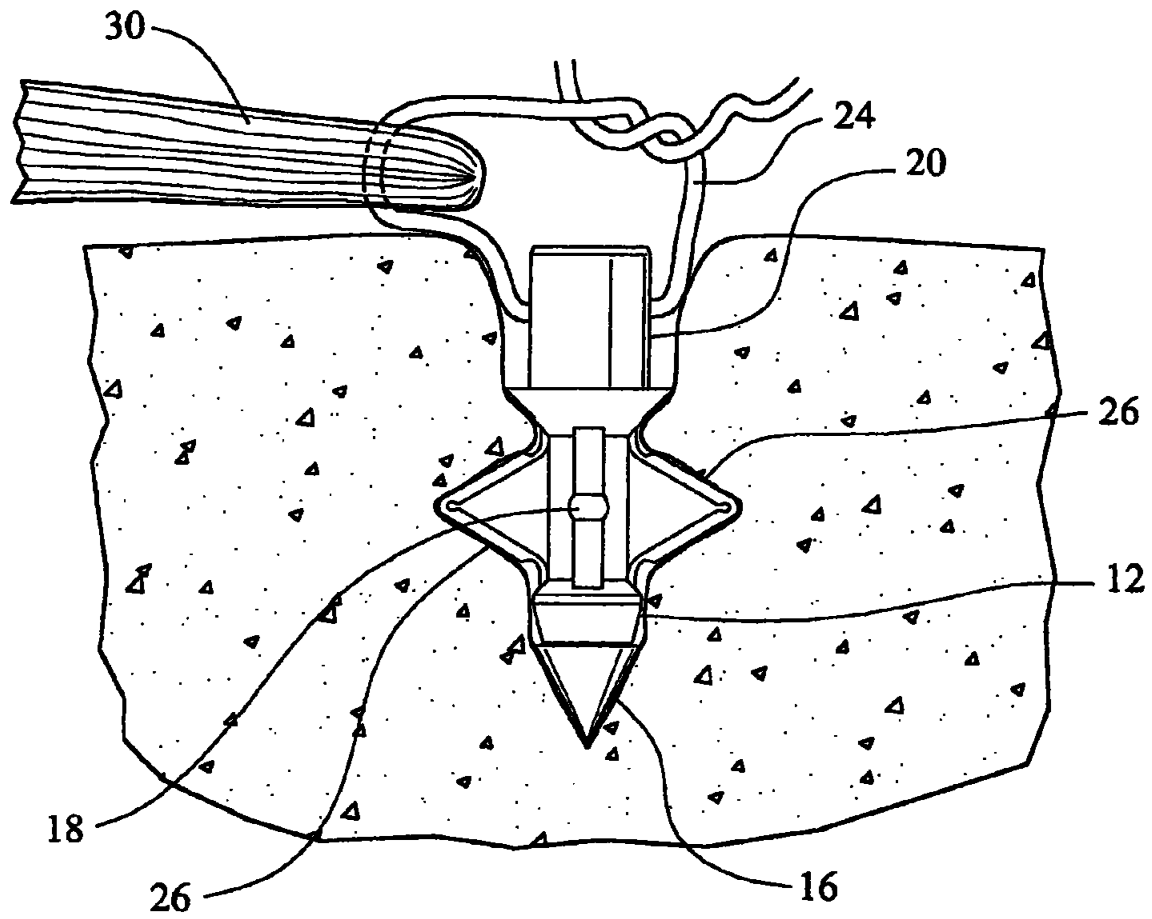
FIG. 9 (PRIOR ART)
